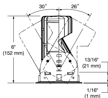
WITH FLANGE
