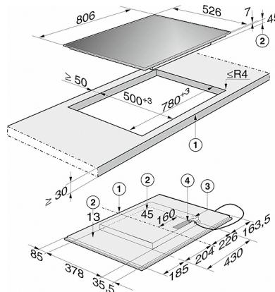
KM 6344 (Installation Drawing)
