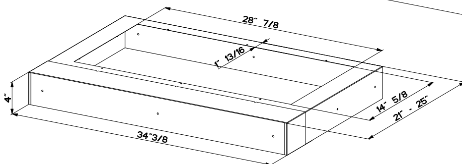
LINE36PR Dimensions
