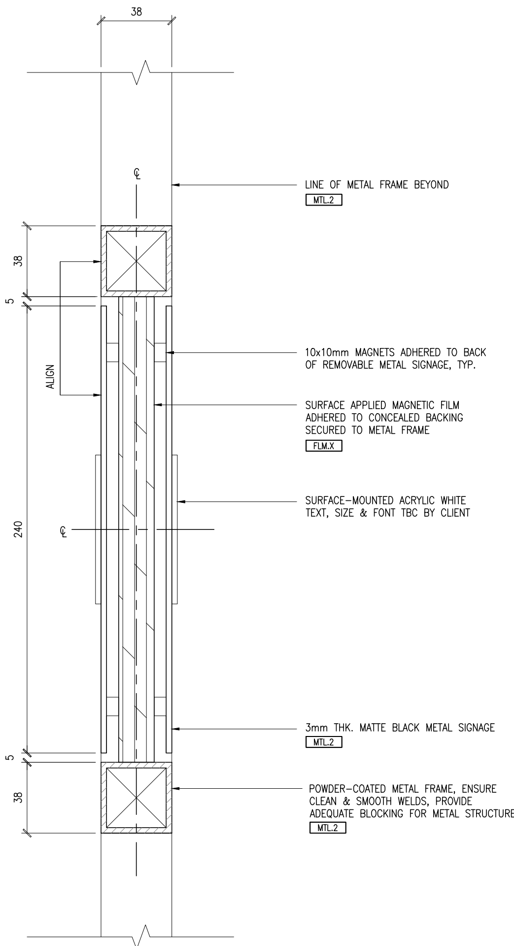
3 ID6.4 SCALE 1:1.2 SECTION - MAGNETIC SIGNAGE
