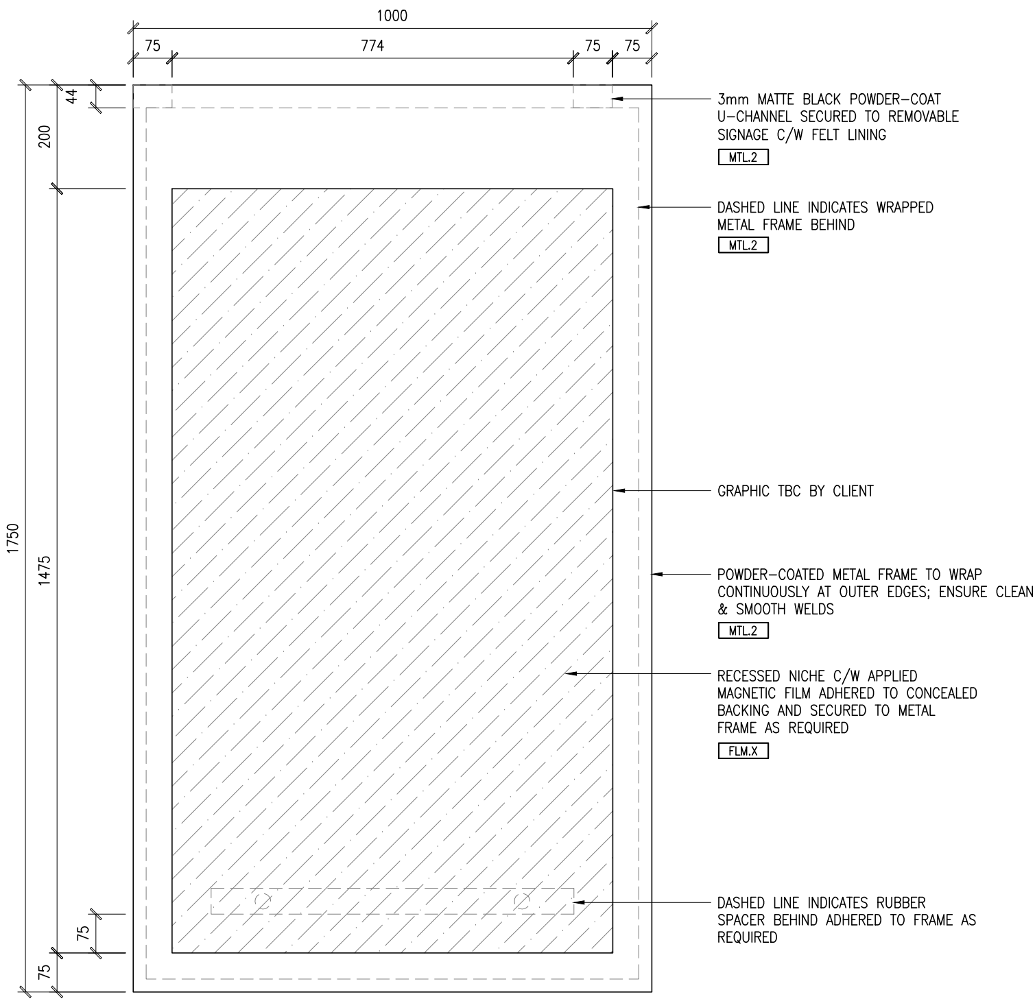
1 ID6.4 SCALE 1:1.0 DETAIL - HANGING SIGNAGE BOARD
