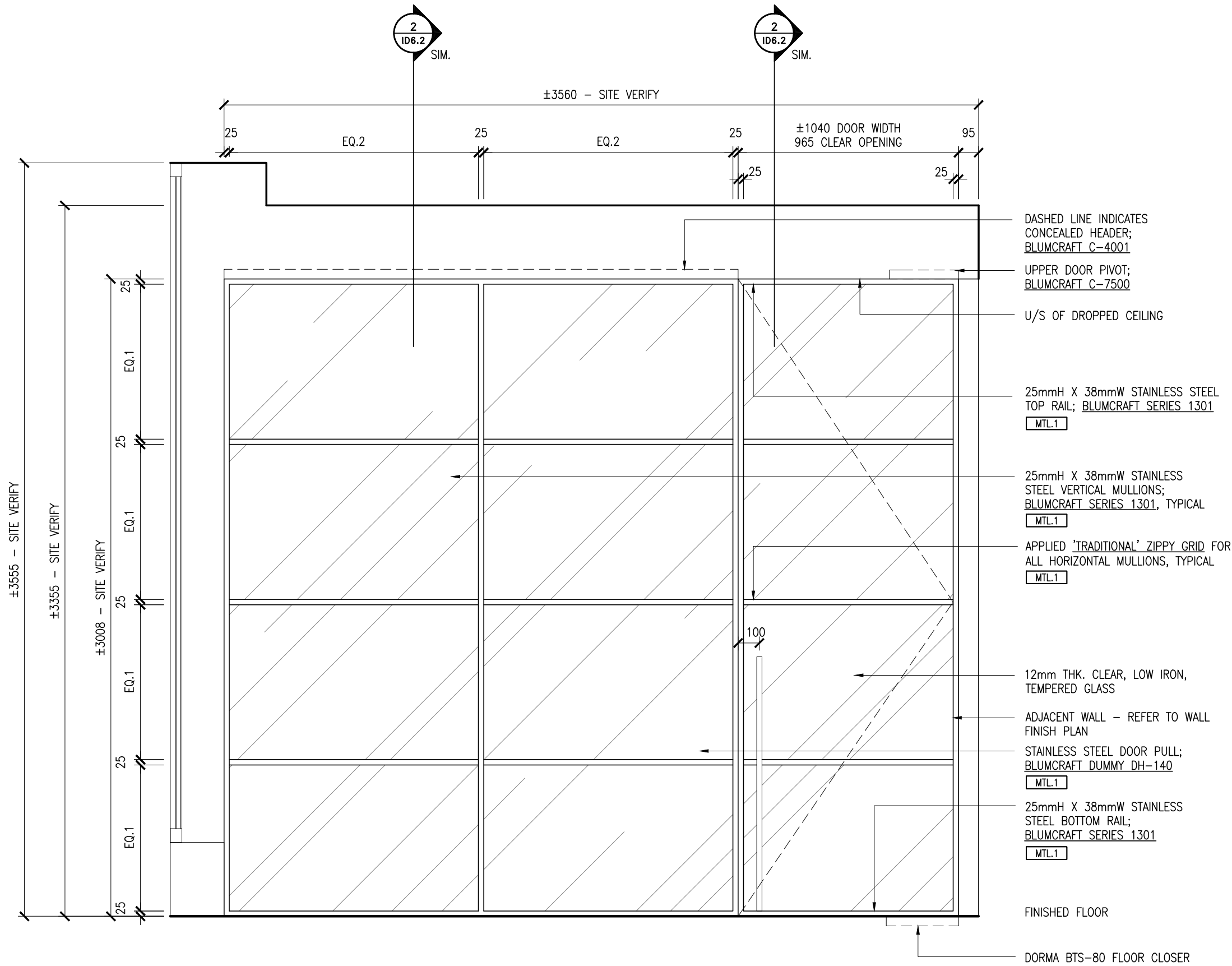
3 ID6.1 DETAIL - GLASS PARTITION @ APPOINTMENT ROOM SCALE 1:20
