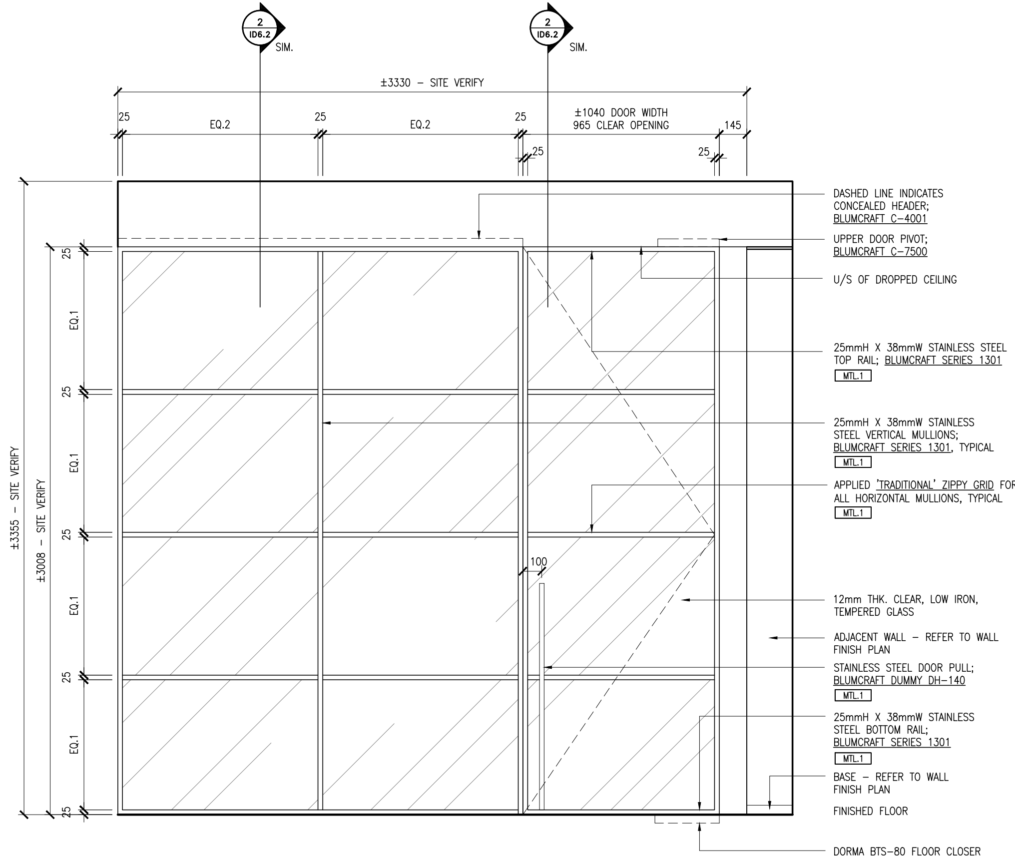
2 ID6.2 DETAIL - GLASS PARTITION @ VR ROOM SCALE 1:20
