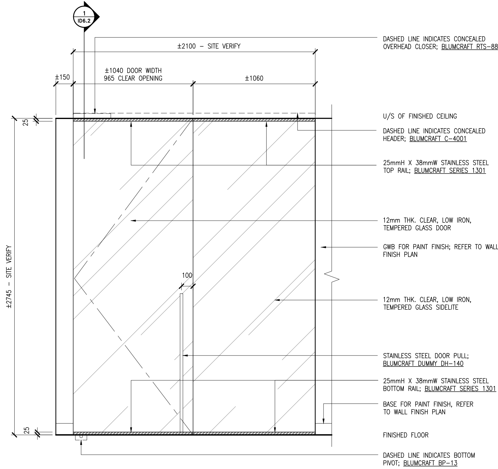
1 ID6.0 SCALE 1:2.0 DETAIL — GLASS PARTITION @ MEETING ROOM
