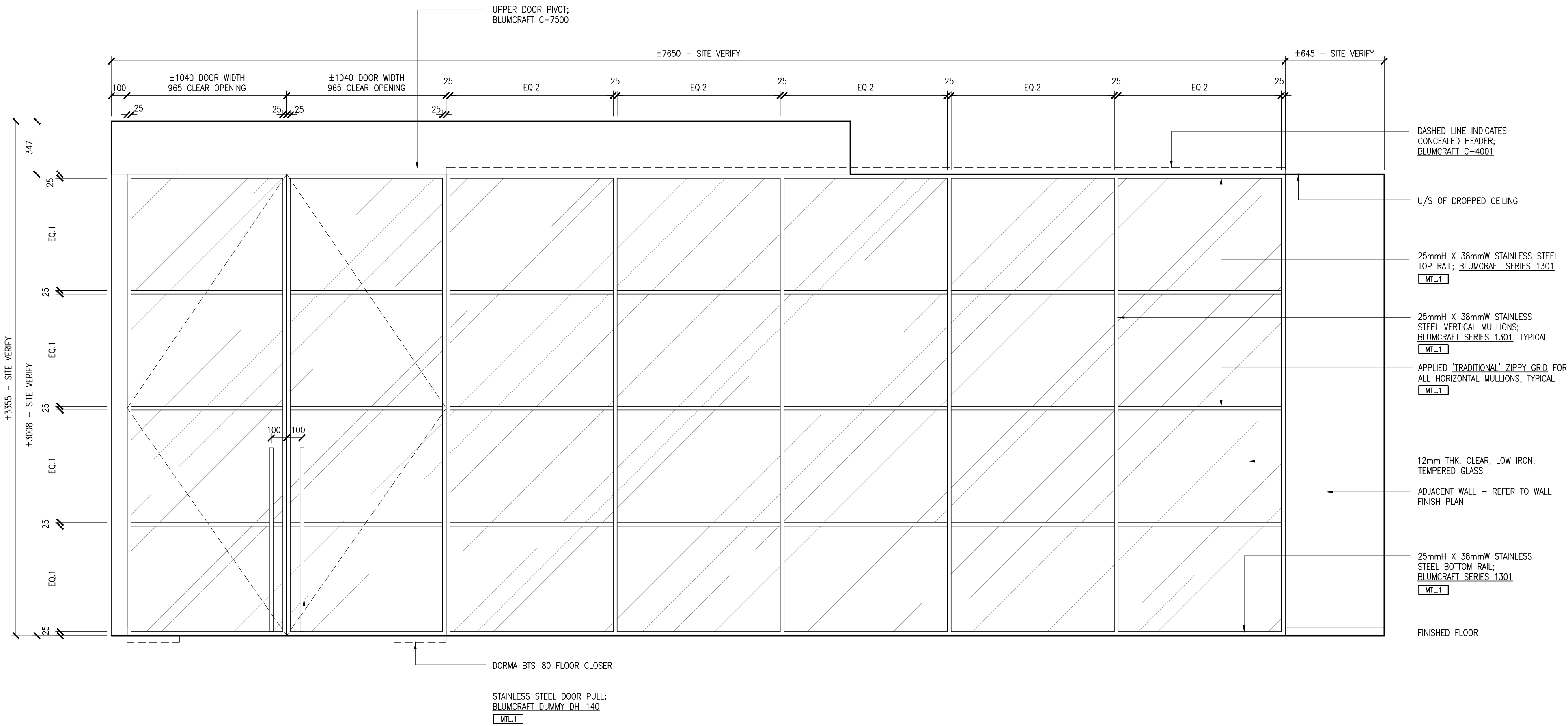
1 ID6.0 SCALE 1:2.0 DETAIL — GLASS PARTITION @ DESIGN STUDIO
