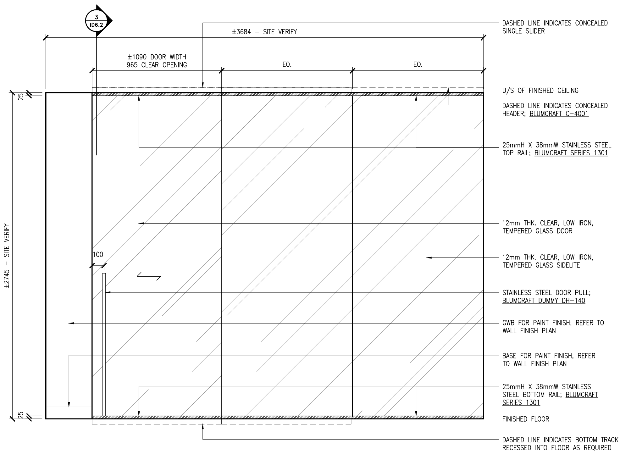
4 ID6.0 SCALE 1:2.0 DETAIL — GLASS PARTITION @ PRIVATE OFFICE
