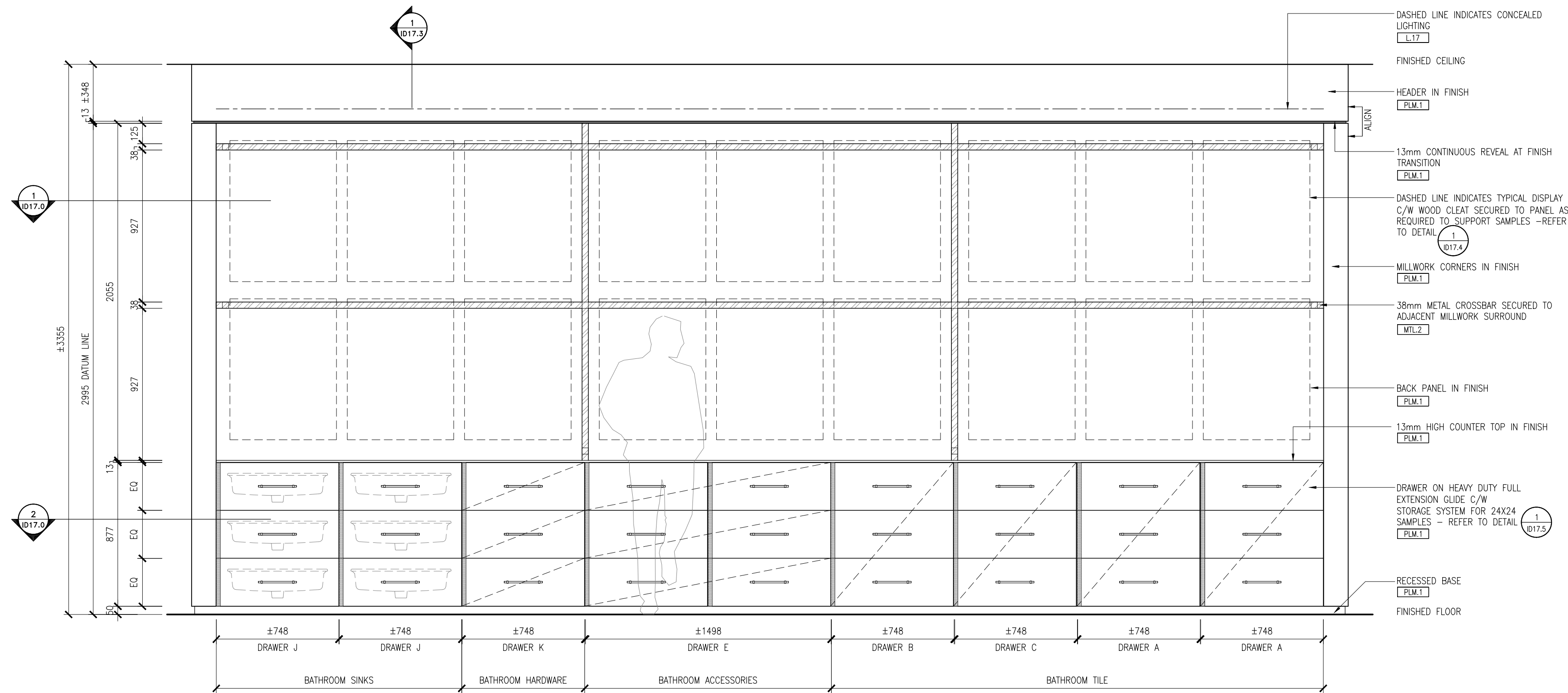
3 ELEVATION - TILE DISPLAY SCALE 1:2.0
