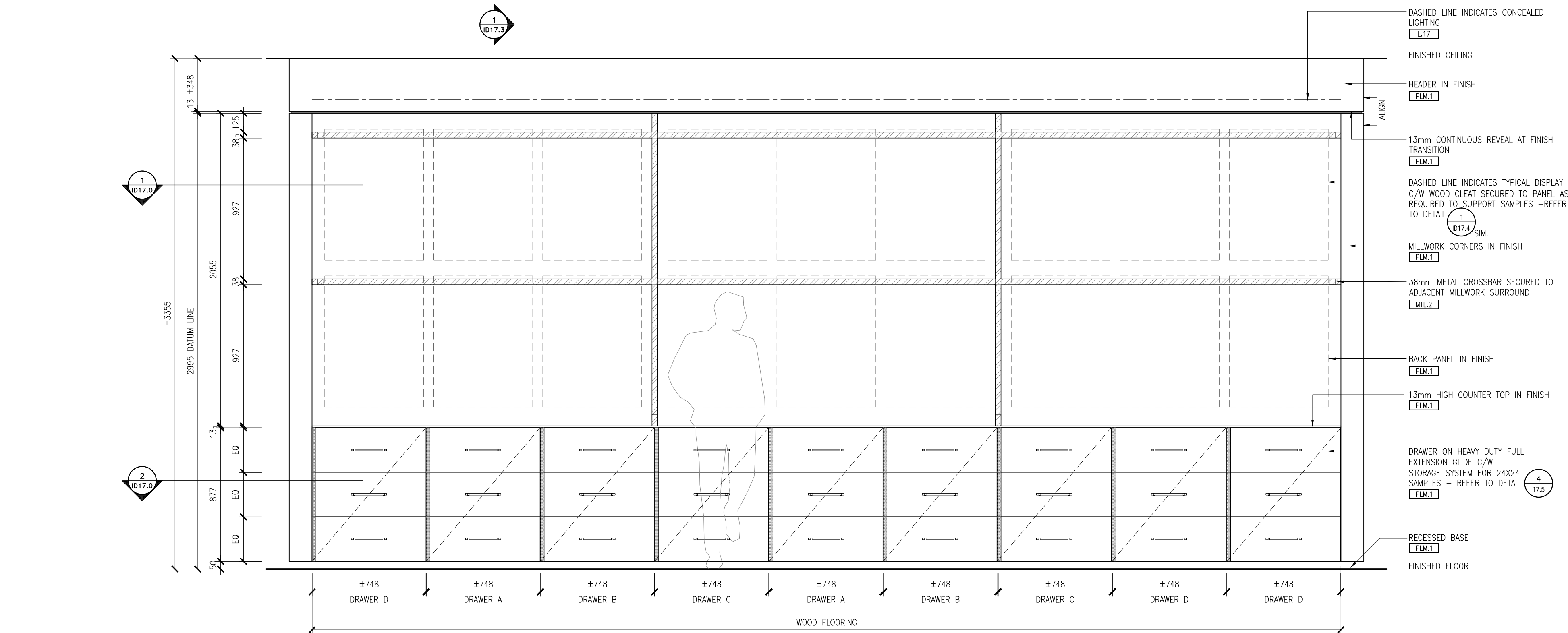
1 ELEVATION - WOOD FLOORING DISPLAY SCALE 1:2.0
