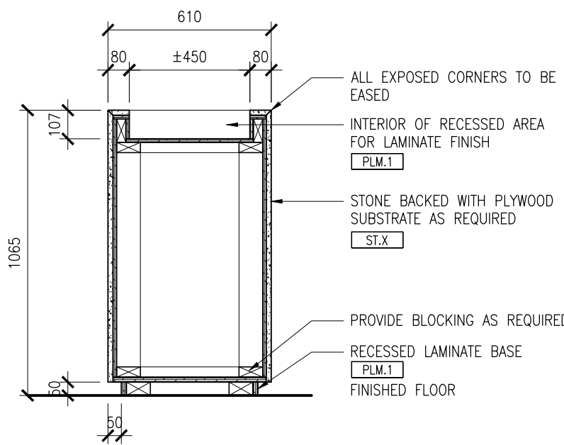
5 SECTION - MOVEABLE STONE PLINTH SCALE 1:20
