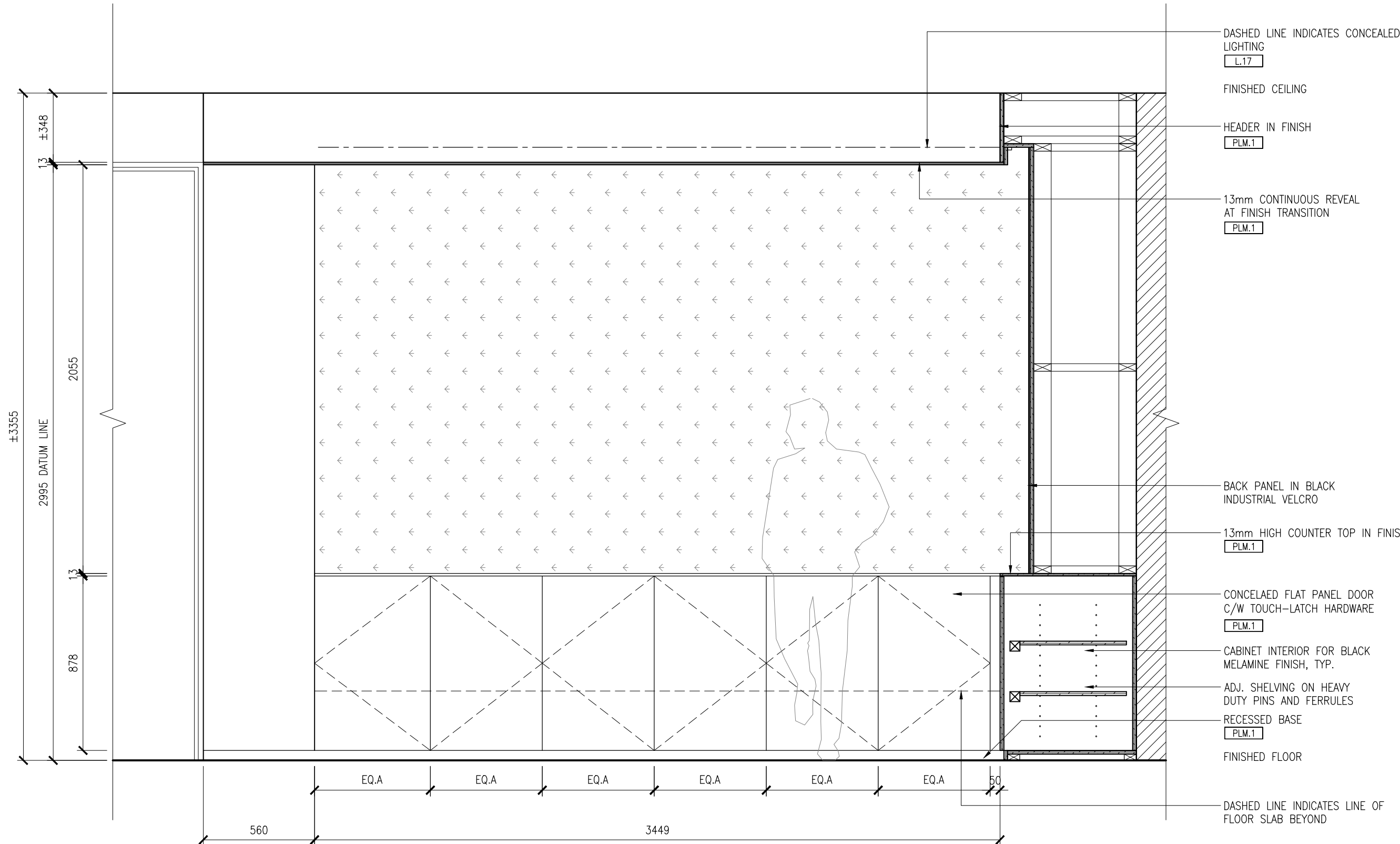
2 ELEVATION - LIFESTYLE + PALETTE DISPLAY SCALE 1:20
