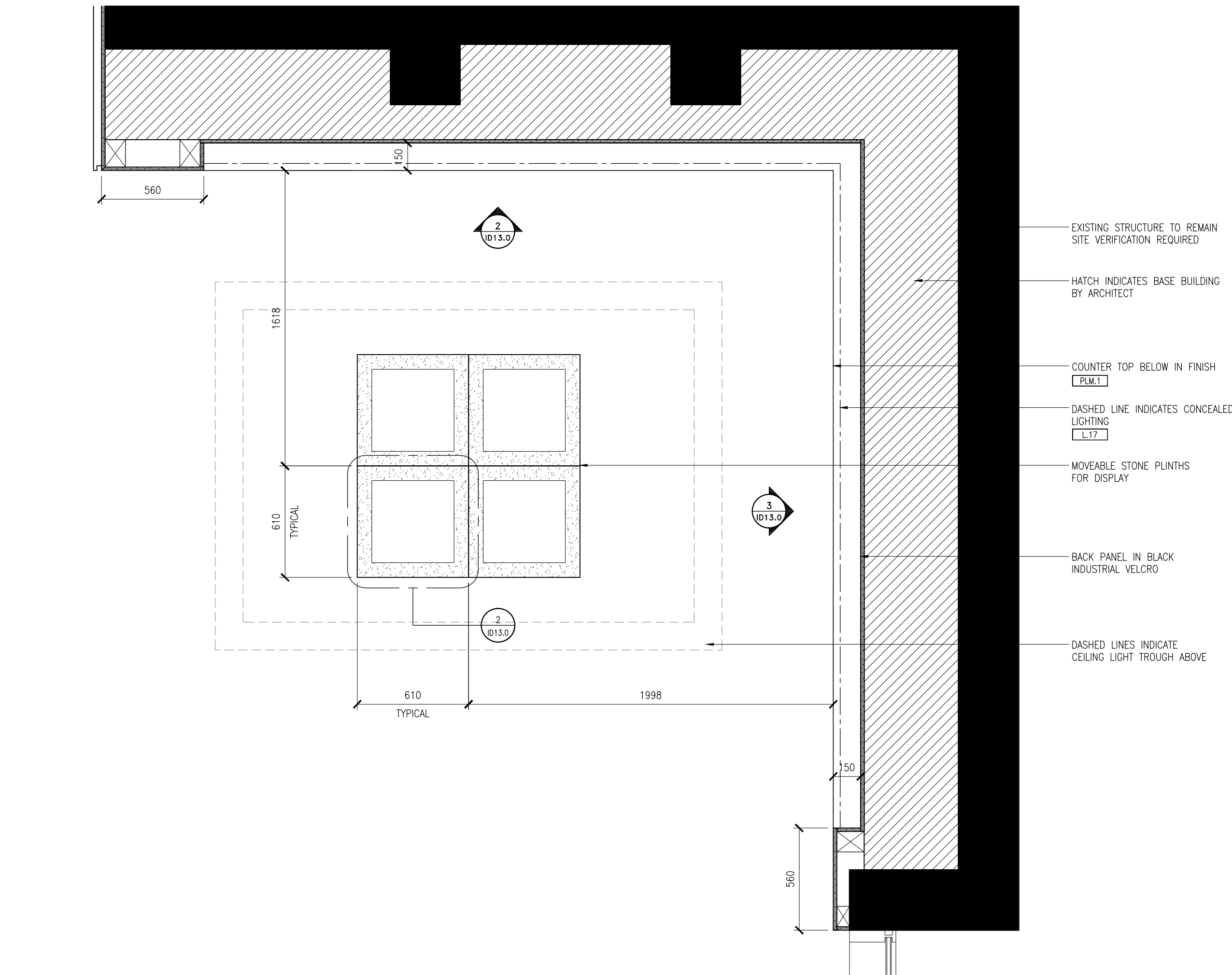
1 PLAN - LIFESTYLE + PALETTE DISPLAY SCALE 1:20
