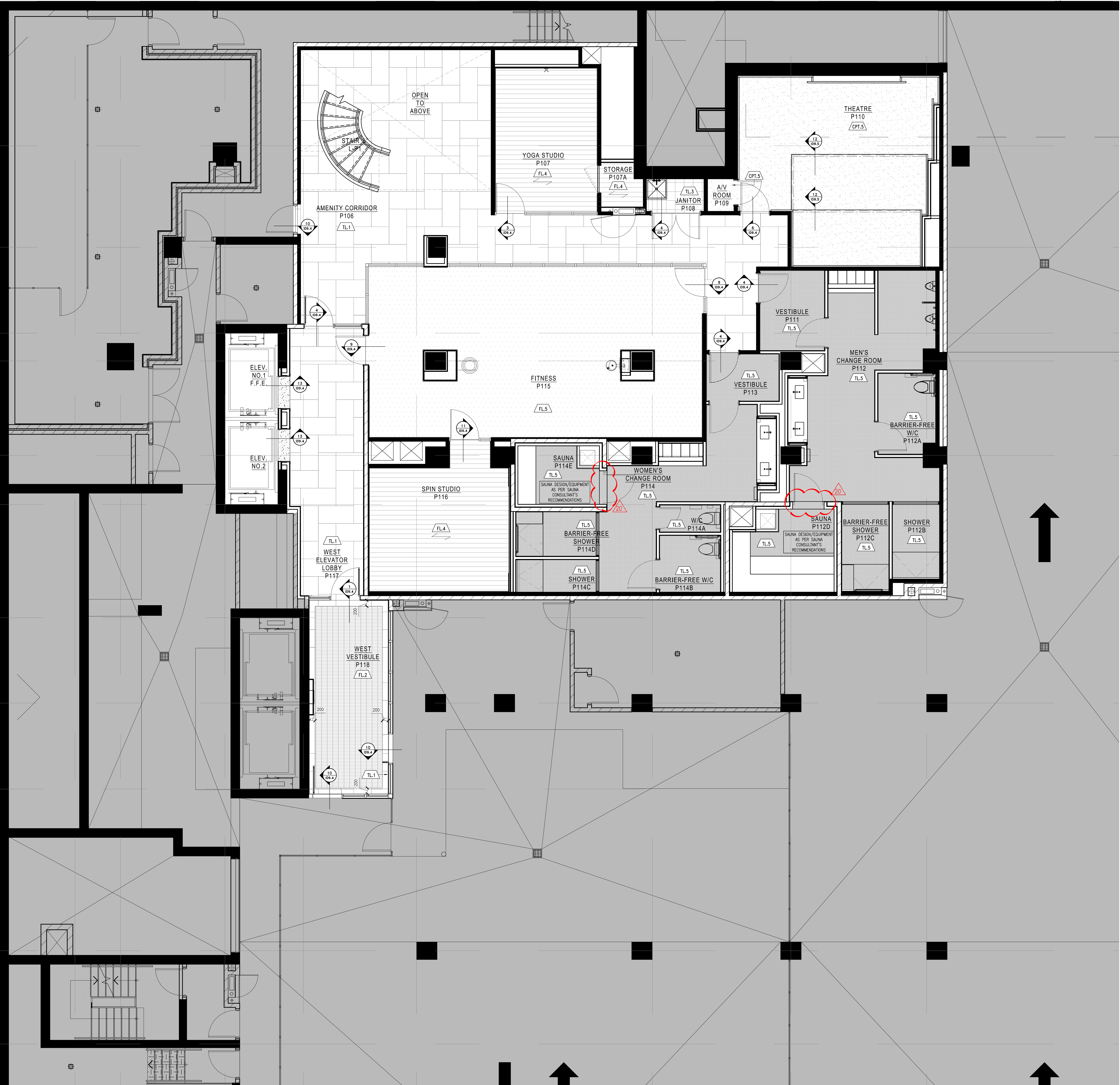
1 FLOOR FINISH PLAN 107.4 SCALE 1:50
