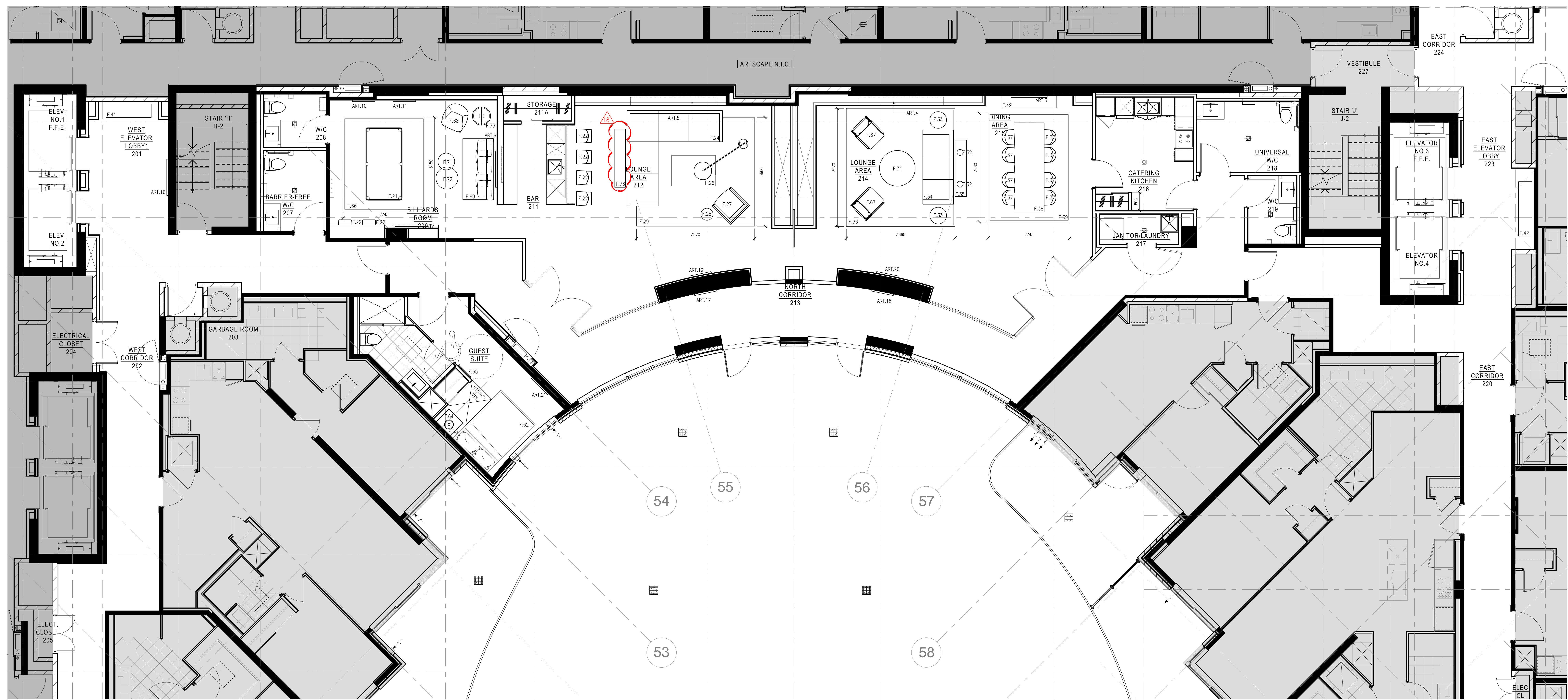
1. FIXTURE PLAN 05.84 942 1:50
