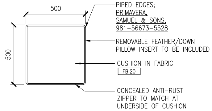
2 SMALL CUSHION (F.67A) D3.14.0 SCALE 1:20 QTY. 2
