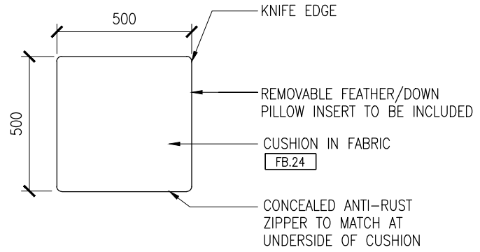
3 SMALL CUSHION (F.68A) D3.14.0 SCALE 1:20 QTY. 1
