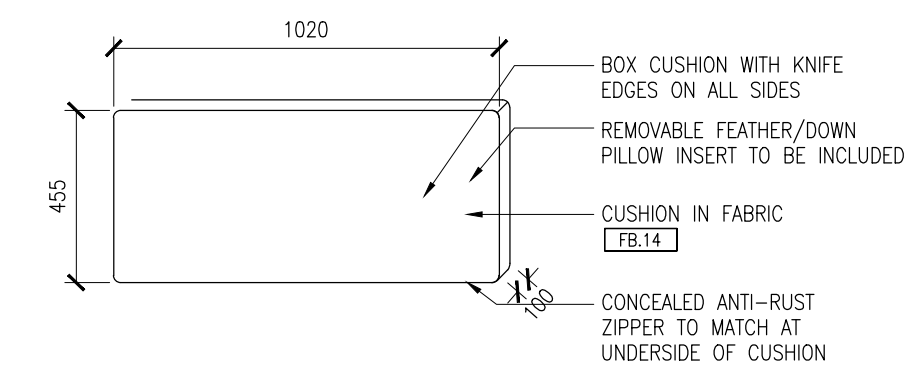
3 LARGE BOX CUSHION ELEVATION D3.13.0 SCALE 1:20 QTY: 4
