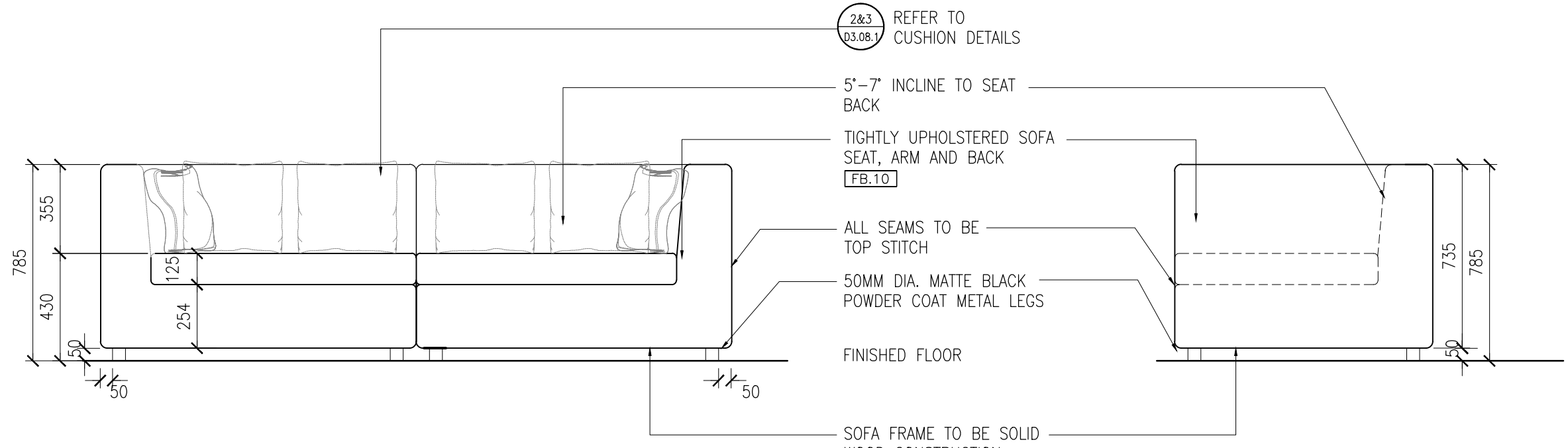
3 ELEVATION D3.08.0 SCALE 1:20
