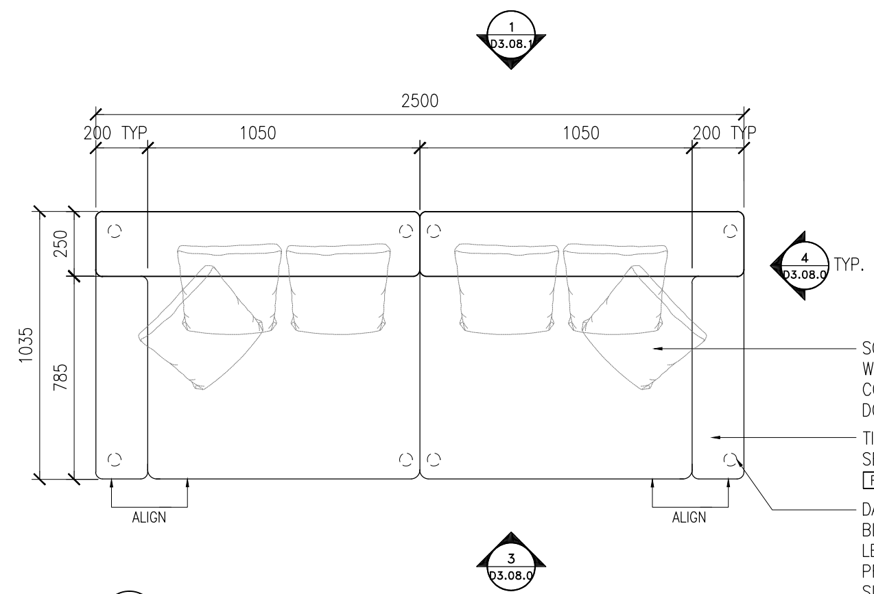
1 PLAN D3.08.0 SCALE 1:20
