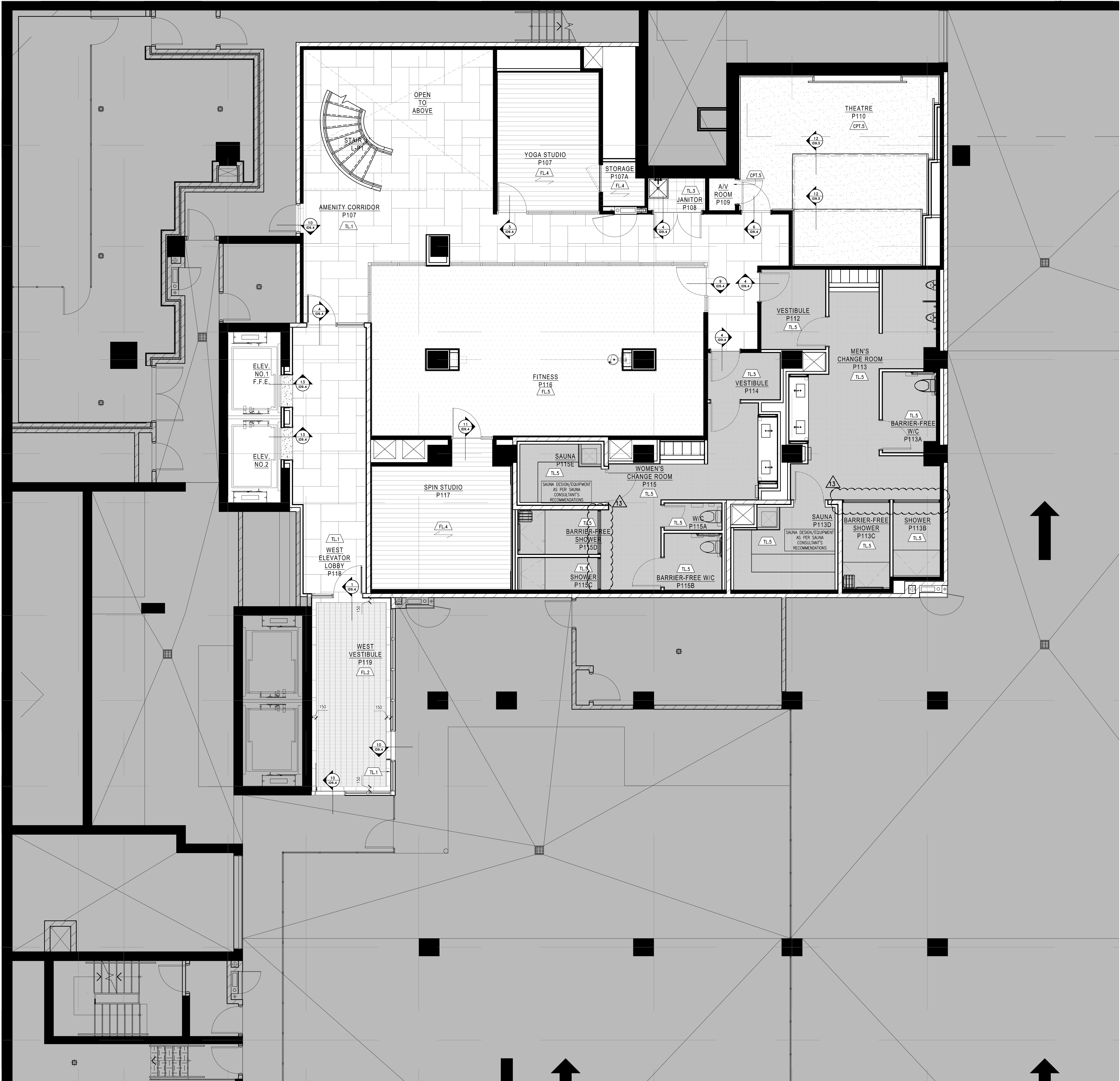
1 FLOOR FINISH PLAN 107.4 SCALE 1:150
