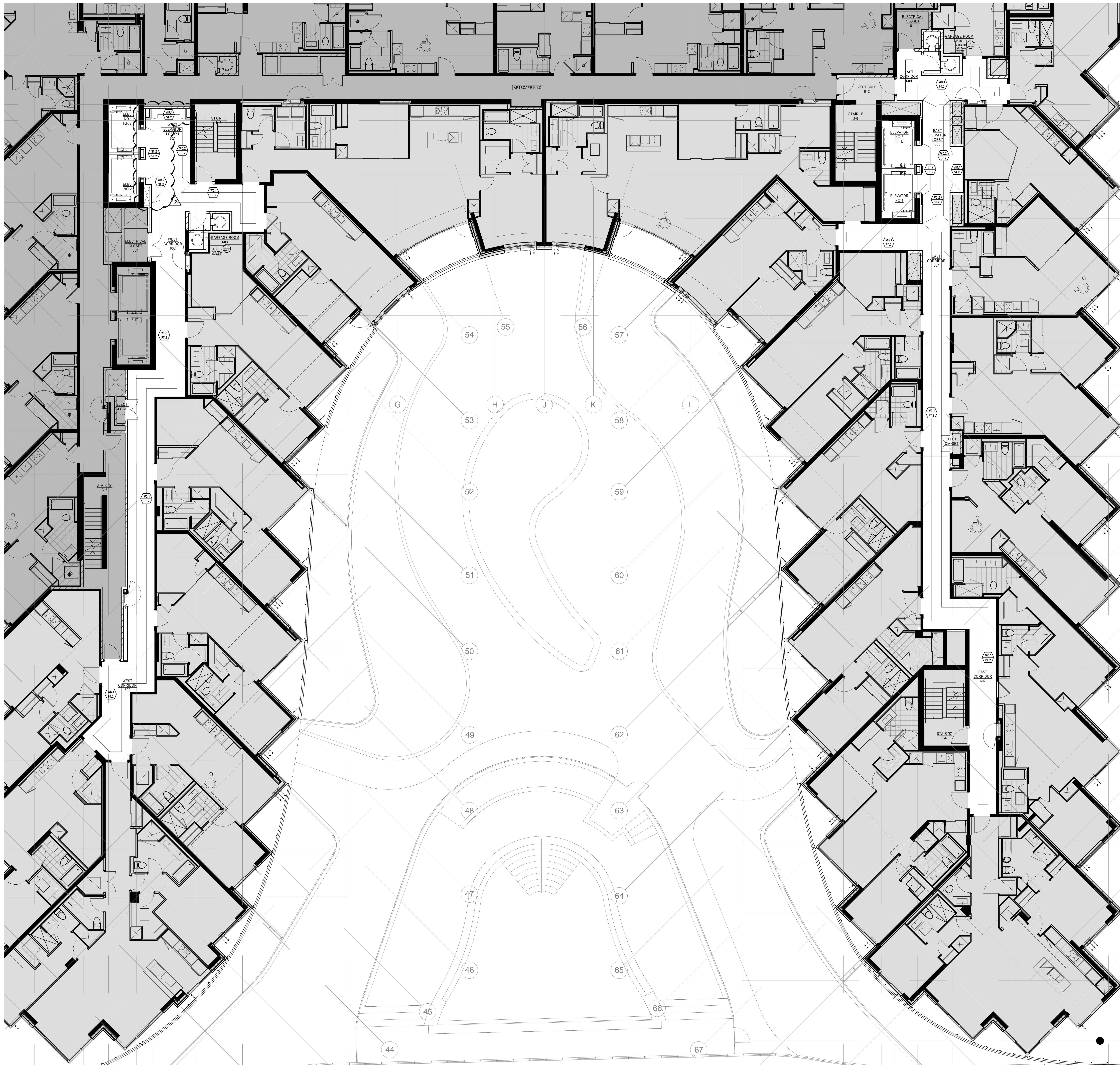
1 WALL FINISH PLAN 06.12 SCALE: 1:7.5
