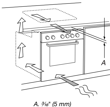
Installed in Built-In Cabinet
