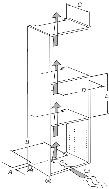
Installed in Built-In Cabinet
