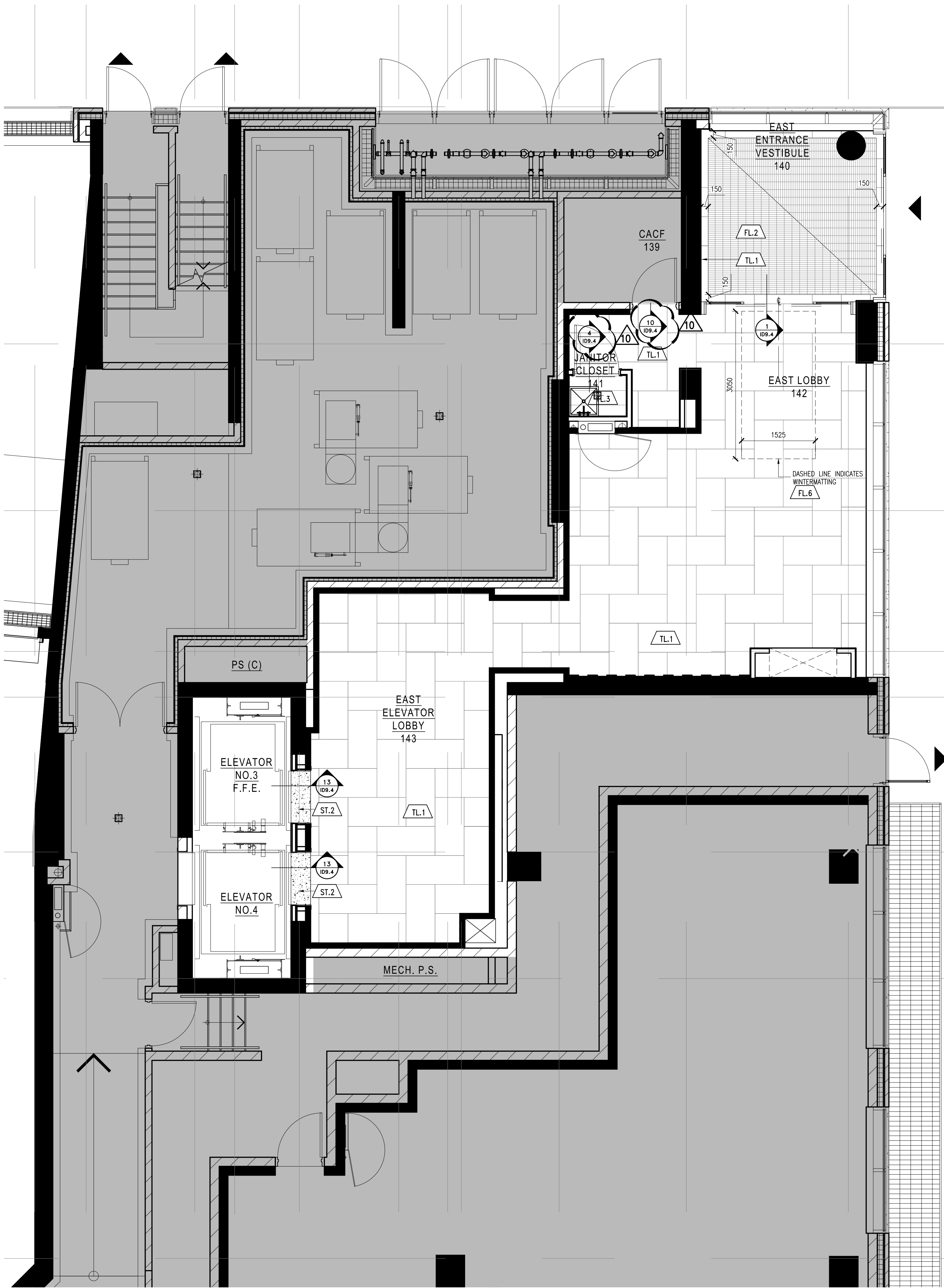
2 FLOOR FINISH PLAN SCALE 1:150
