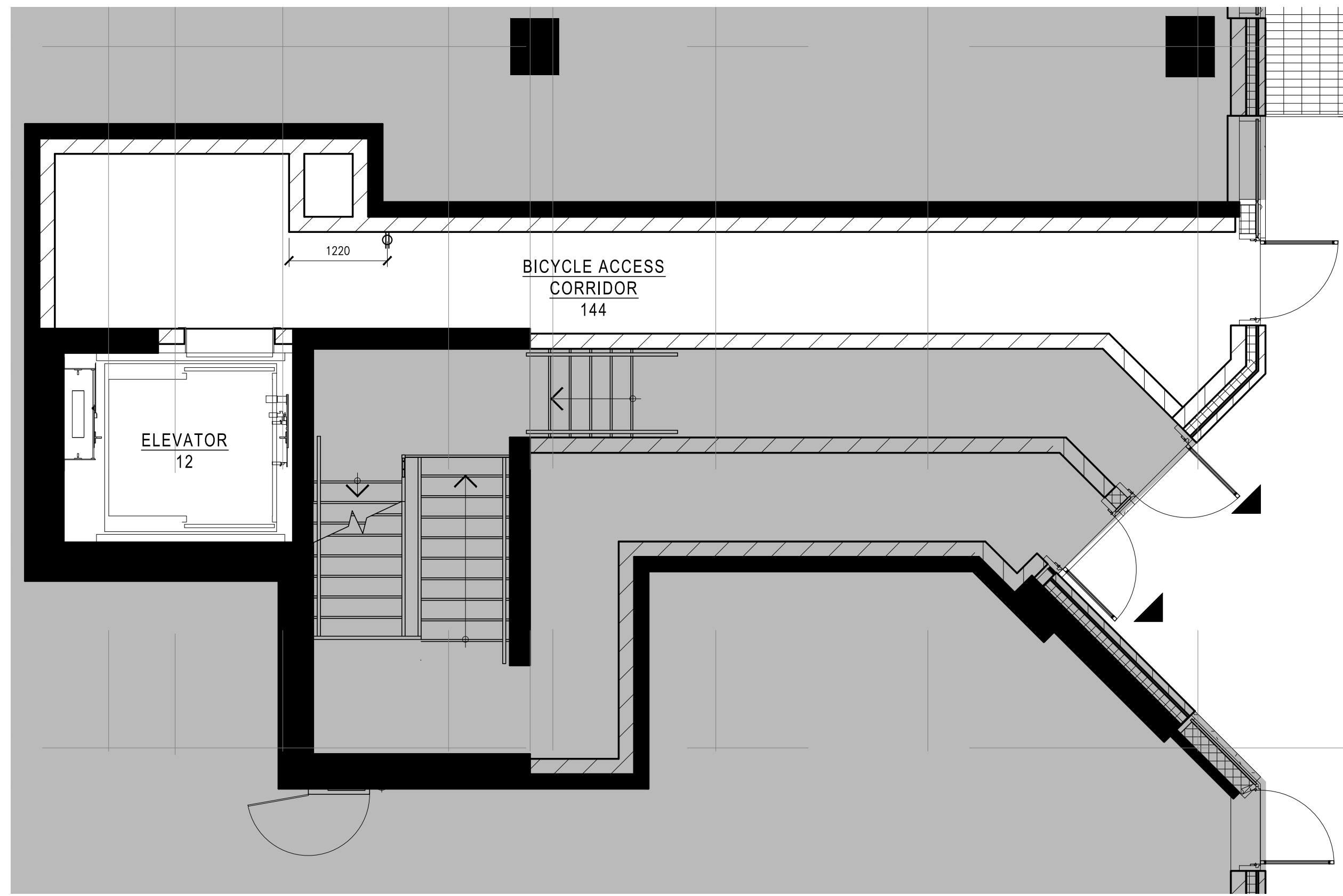
3 POWER AND COMMUNICATION PLAN 02.3 SCALE 1:50
