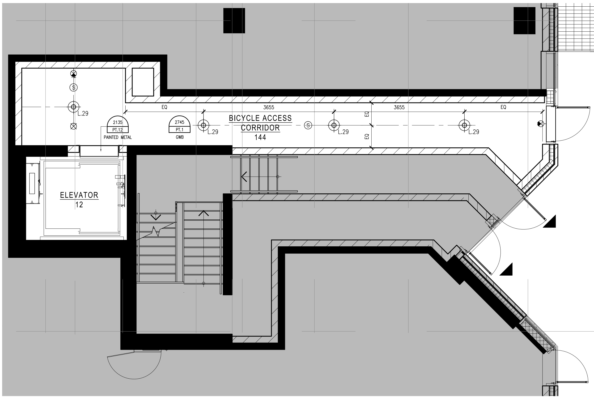
2 REFLECTED CEILING PLAN 02.3 SCALE 1:50
