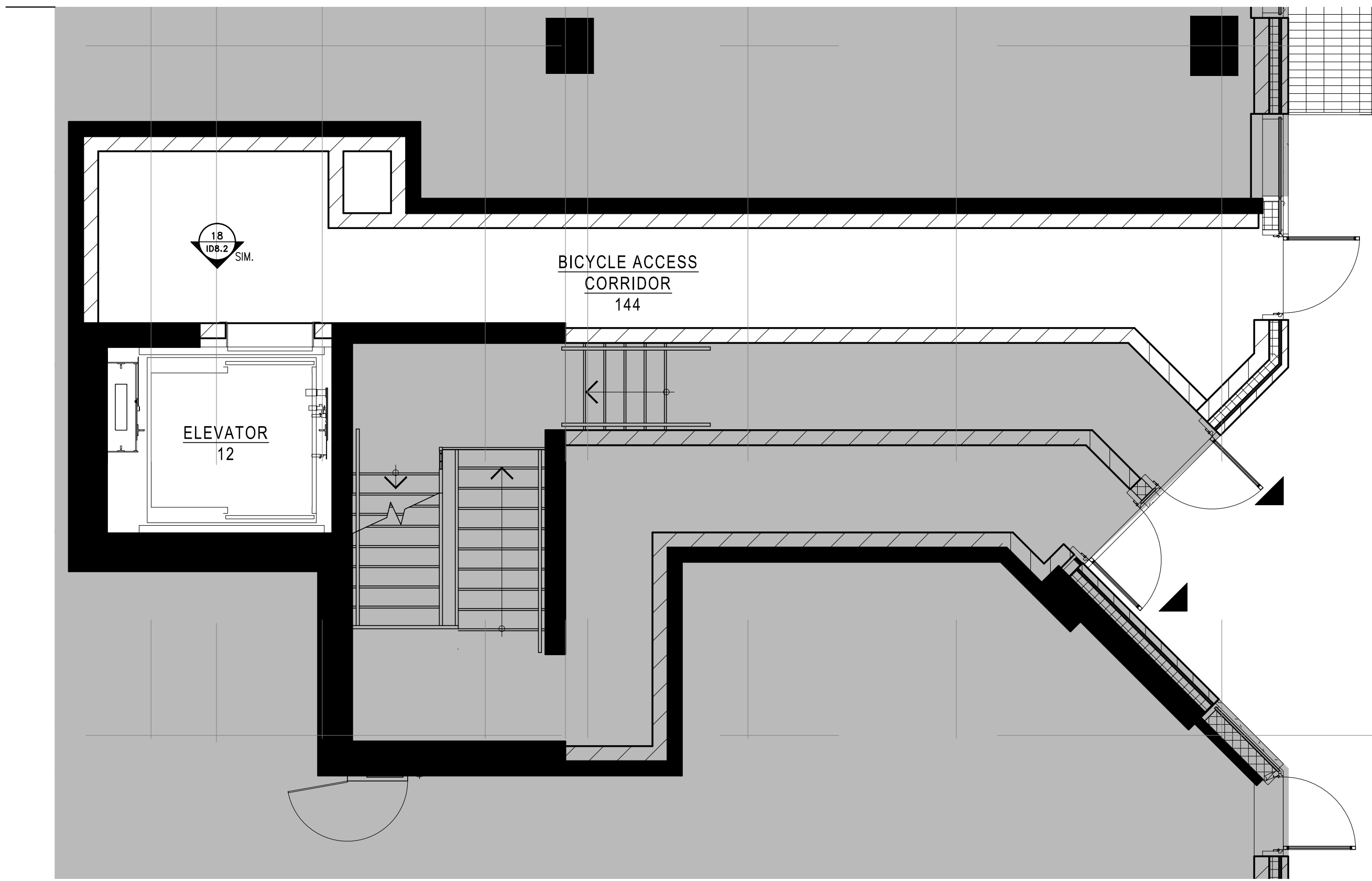
1 CONSTRUCTION PLAN 02.3 SCALE 1:50
