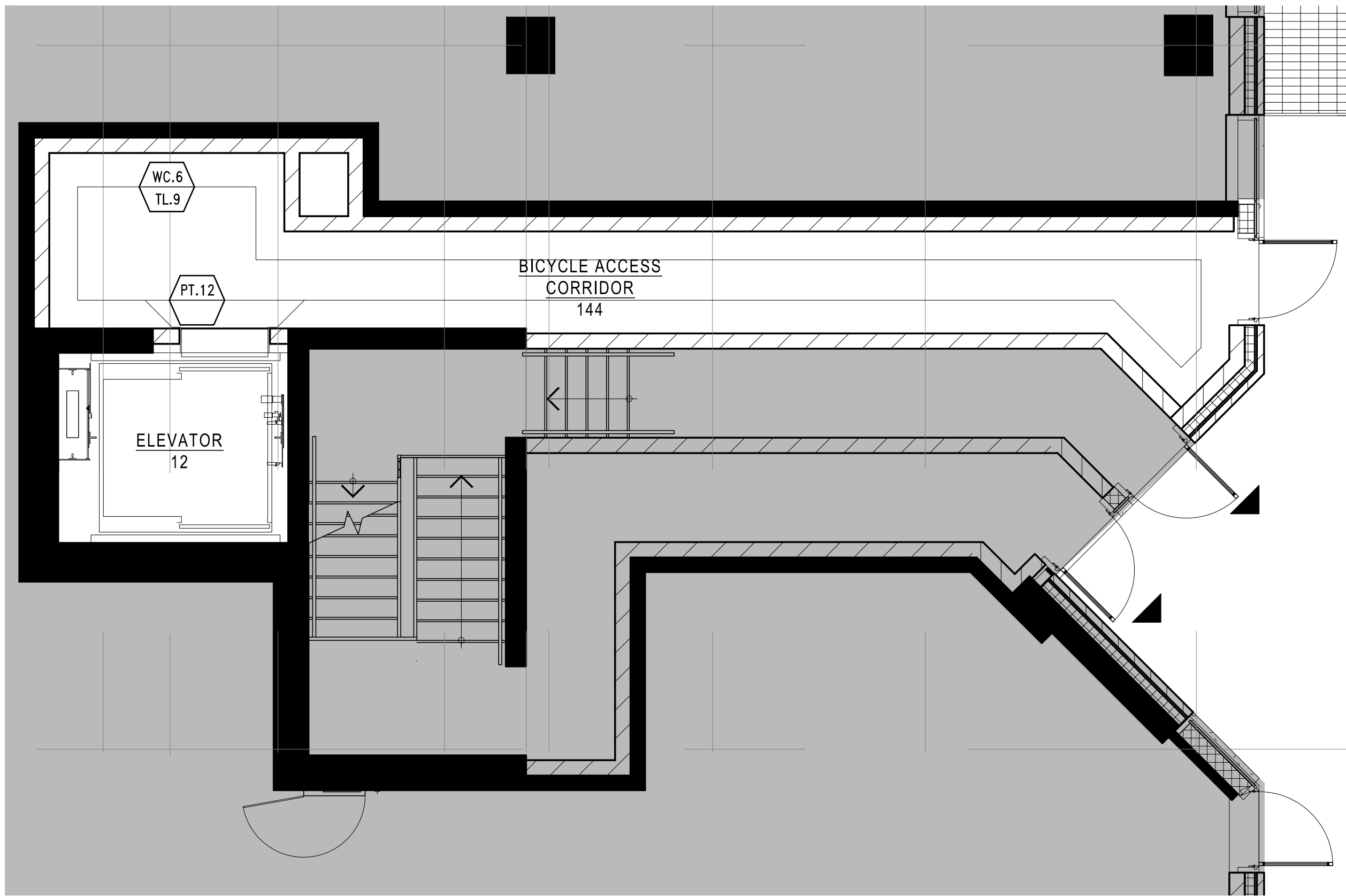
5 WALL FINISH PLAN 02.3 SCALE 1:50
