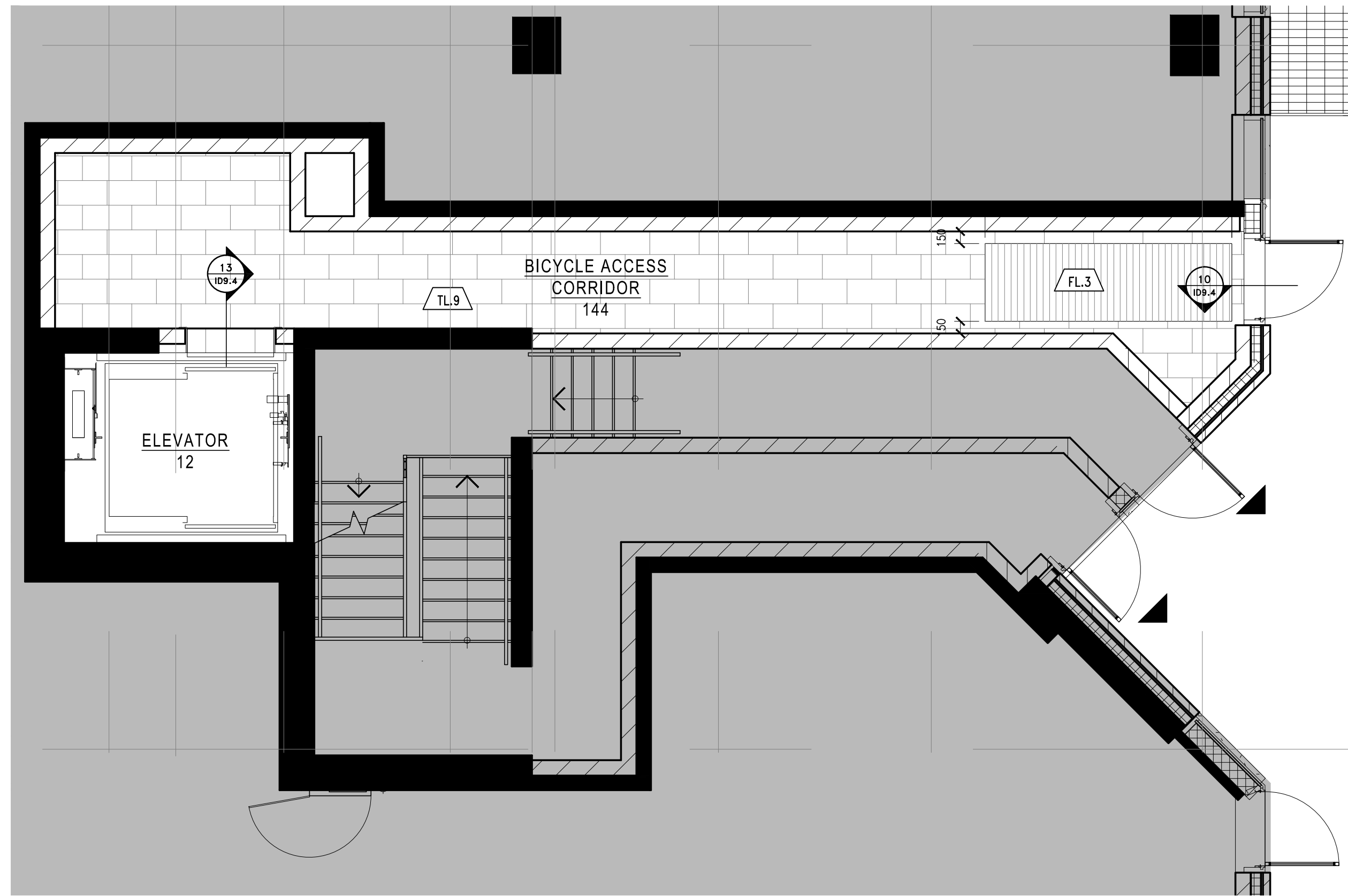
6 FLOOR FINISH PLAN 02.3 SCALE 1:50
