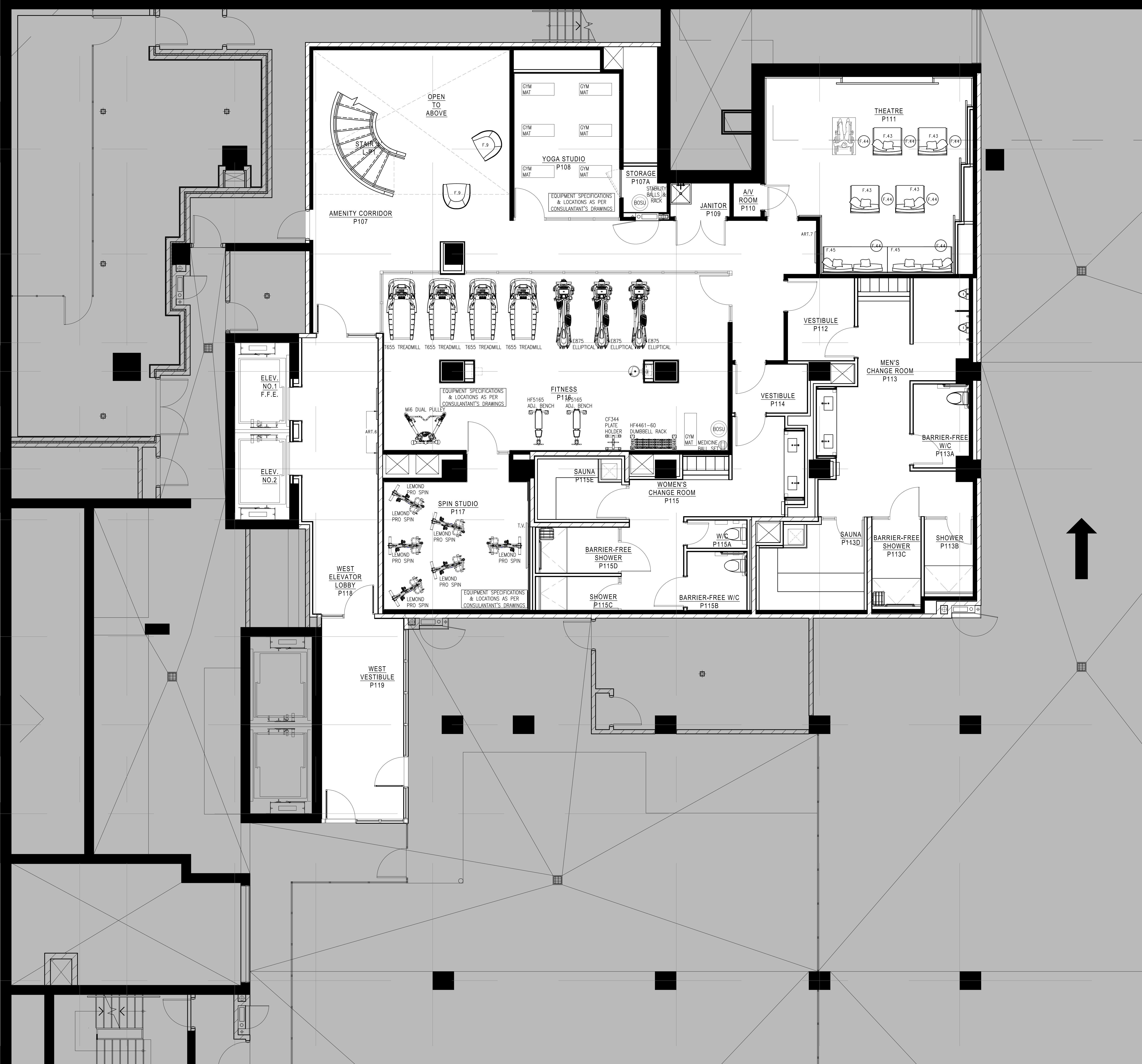
1 FIXTURE PLAN 05.4 SCALE 1:150
