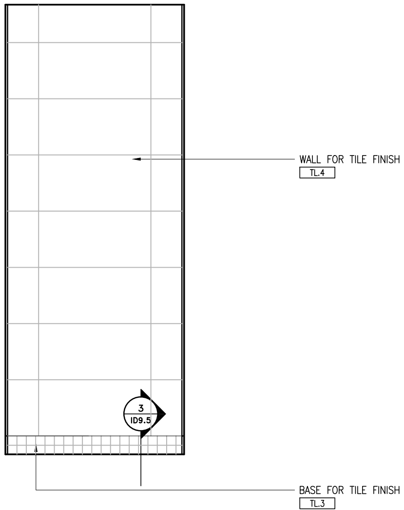
8 ELEVATION - TYPICAL EAST GARBAGE ROOM DR-17 SCALE 1:20
