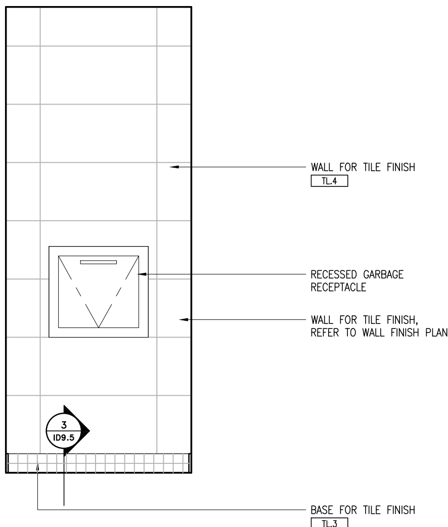
3 ELEVATION - TYPICAL WEST GARBAGE ROOM DR-17 SCALE 1:20
