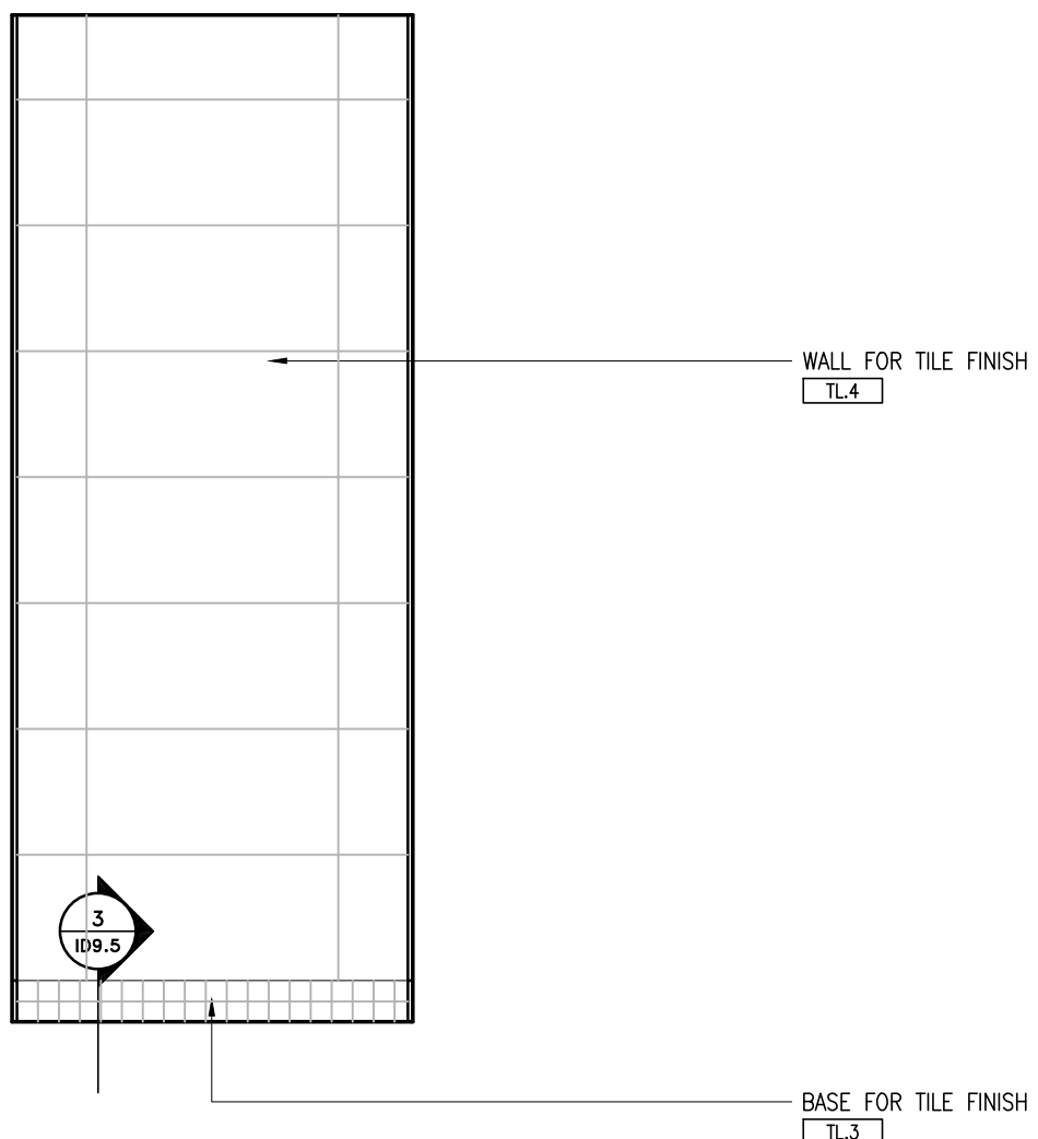
4 ELEVATION - TYPICAL WEST GARBAGE ROOM DR-17 SCALE 1:20
