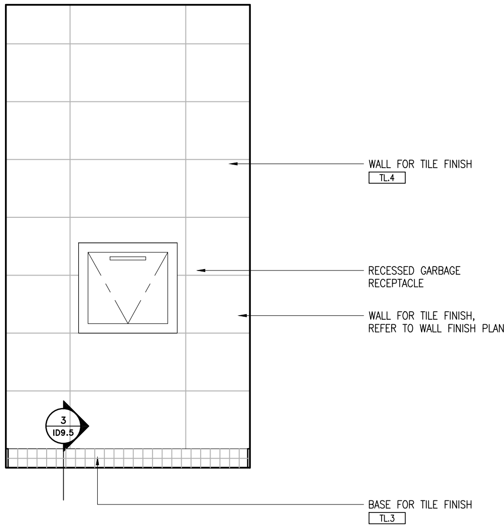
7 ELEVATION - TYPICAL EAST GARBAGE ROOM DR-17 SCALE 1:20
