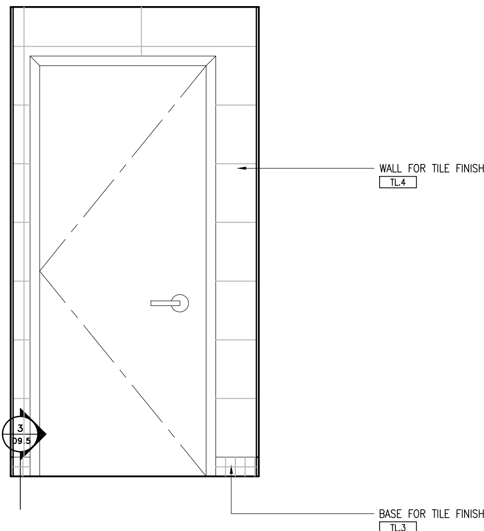
2 ELEVATION - TYPICAL WEST GARBAGE ROOM DR-17 SCALE 1:20
