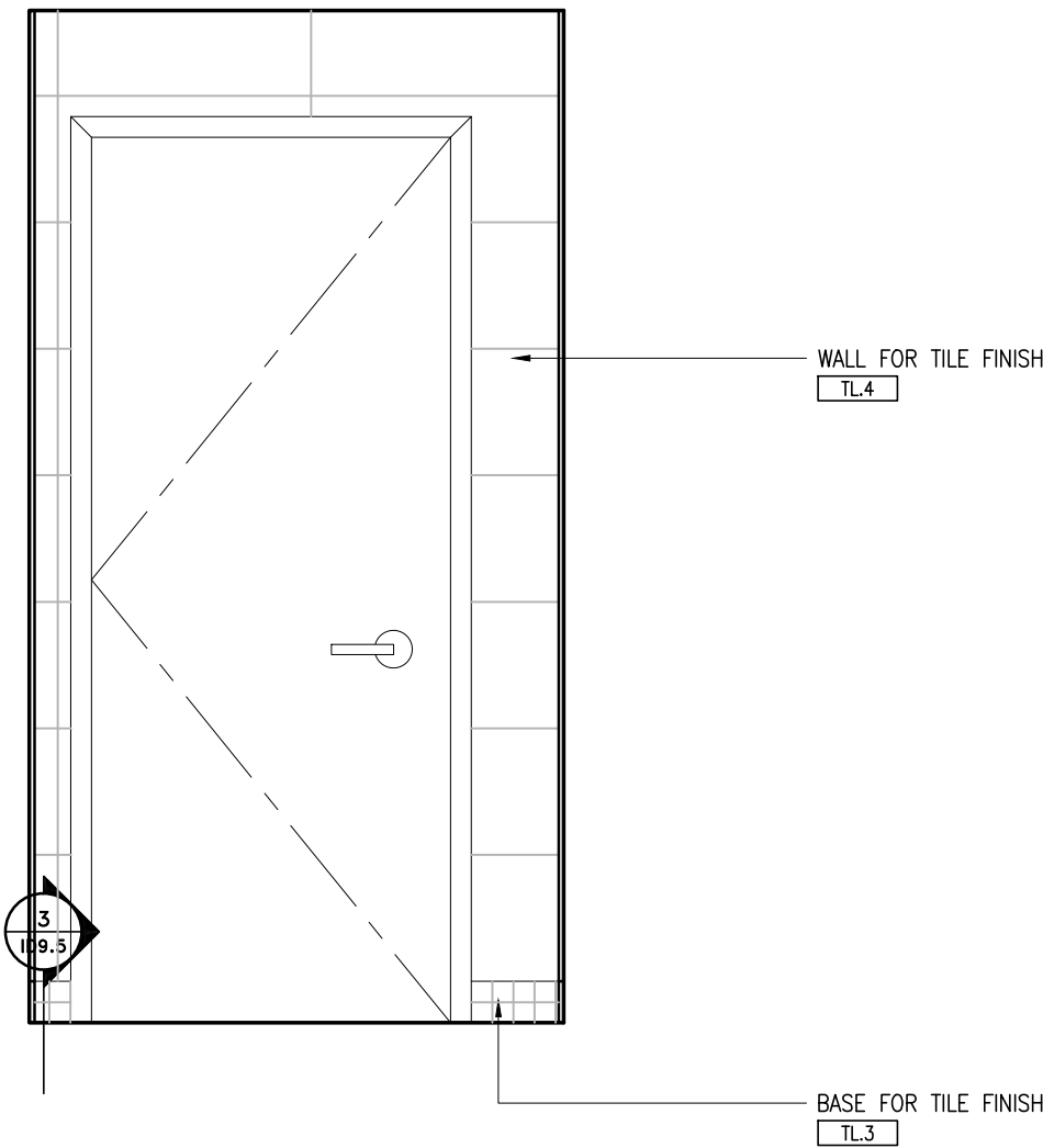
6 ELEVATION - TYPICAL EAST GARBAGE ROOM DR-17 SCALE 1:20
