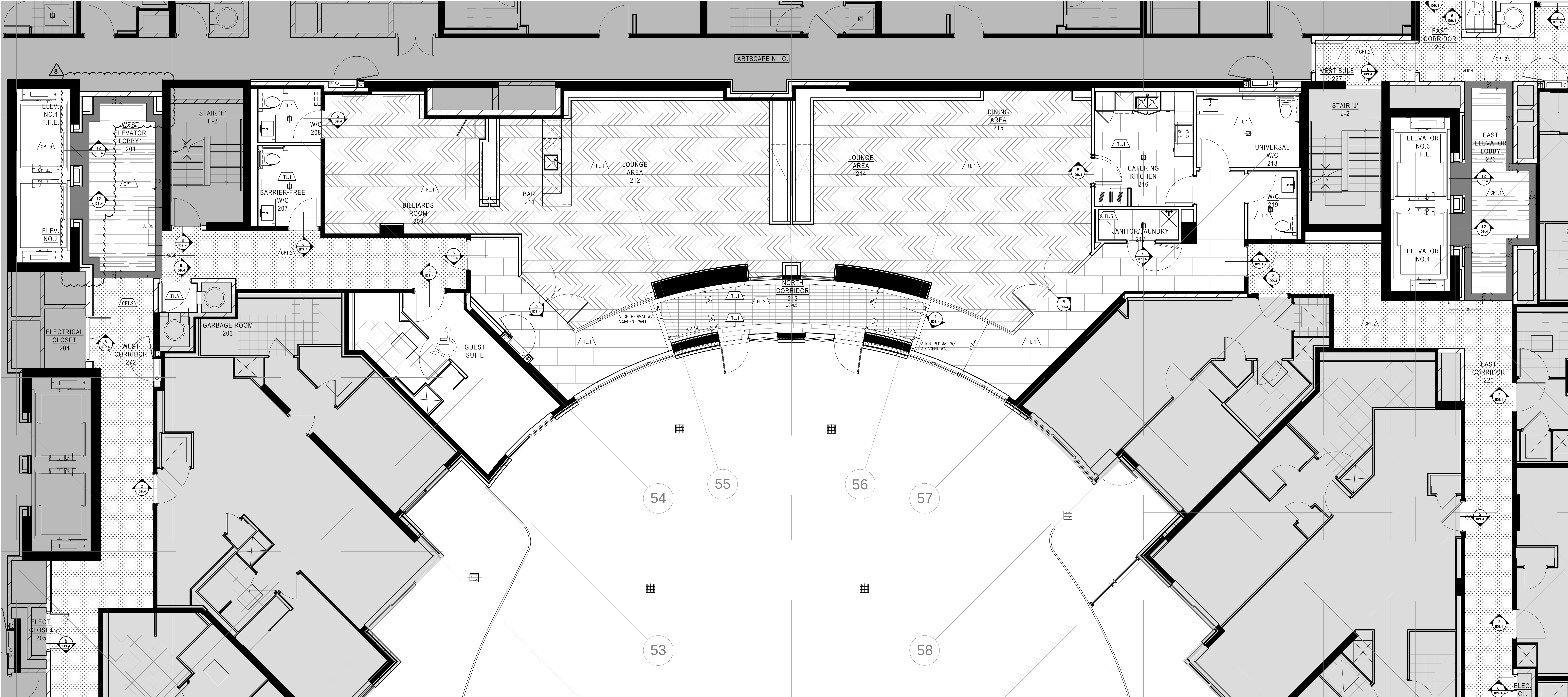
1 FLOOR FINISH PLAN 07.8A SCALE 1:50
