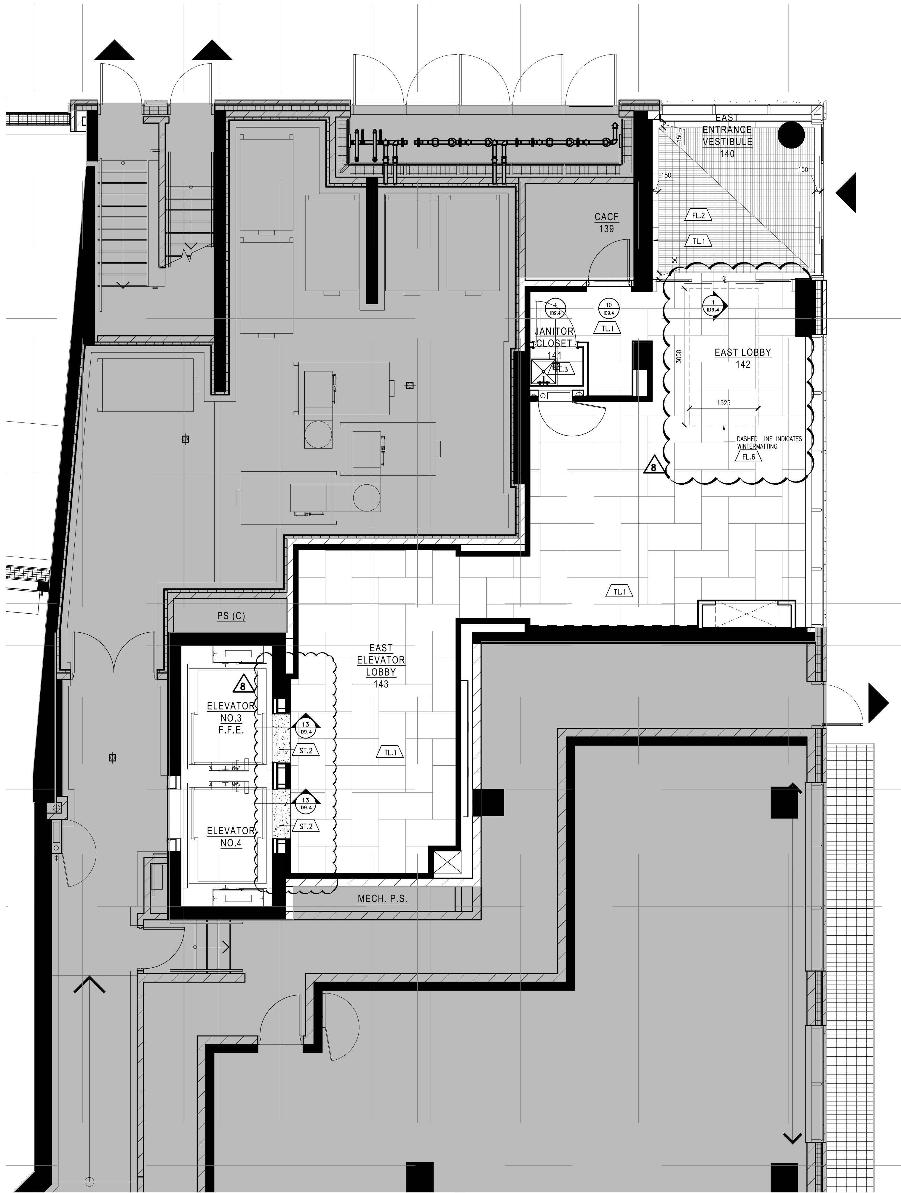
2 FLOOR FINISH PLAN SCALE 1:150
