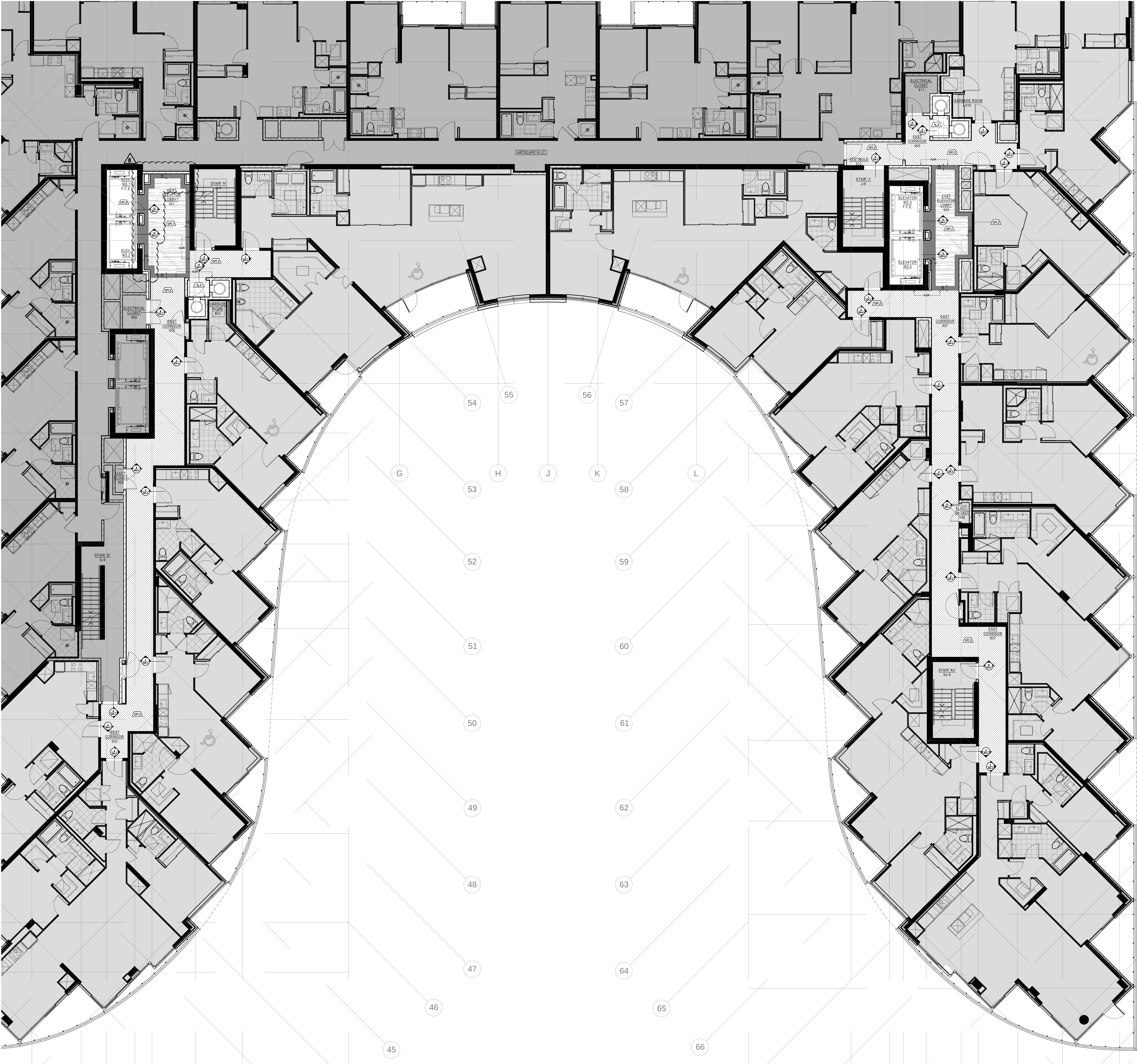
1 FLOOR FINISH PLAN 07.15 SCALE 1:7.5
