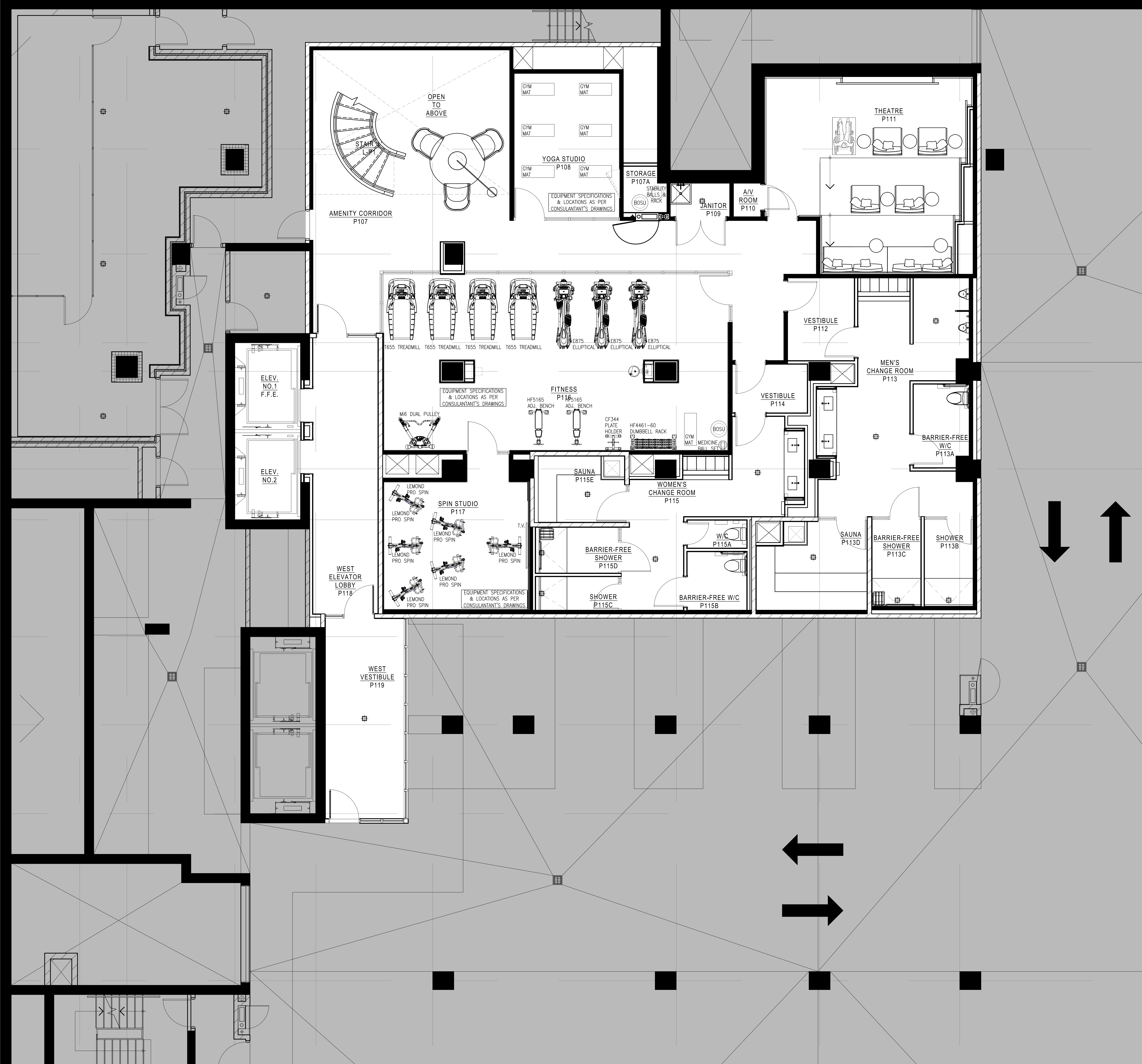
1. FIXTURE PLAN 05.4 SCALE: 1/50
