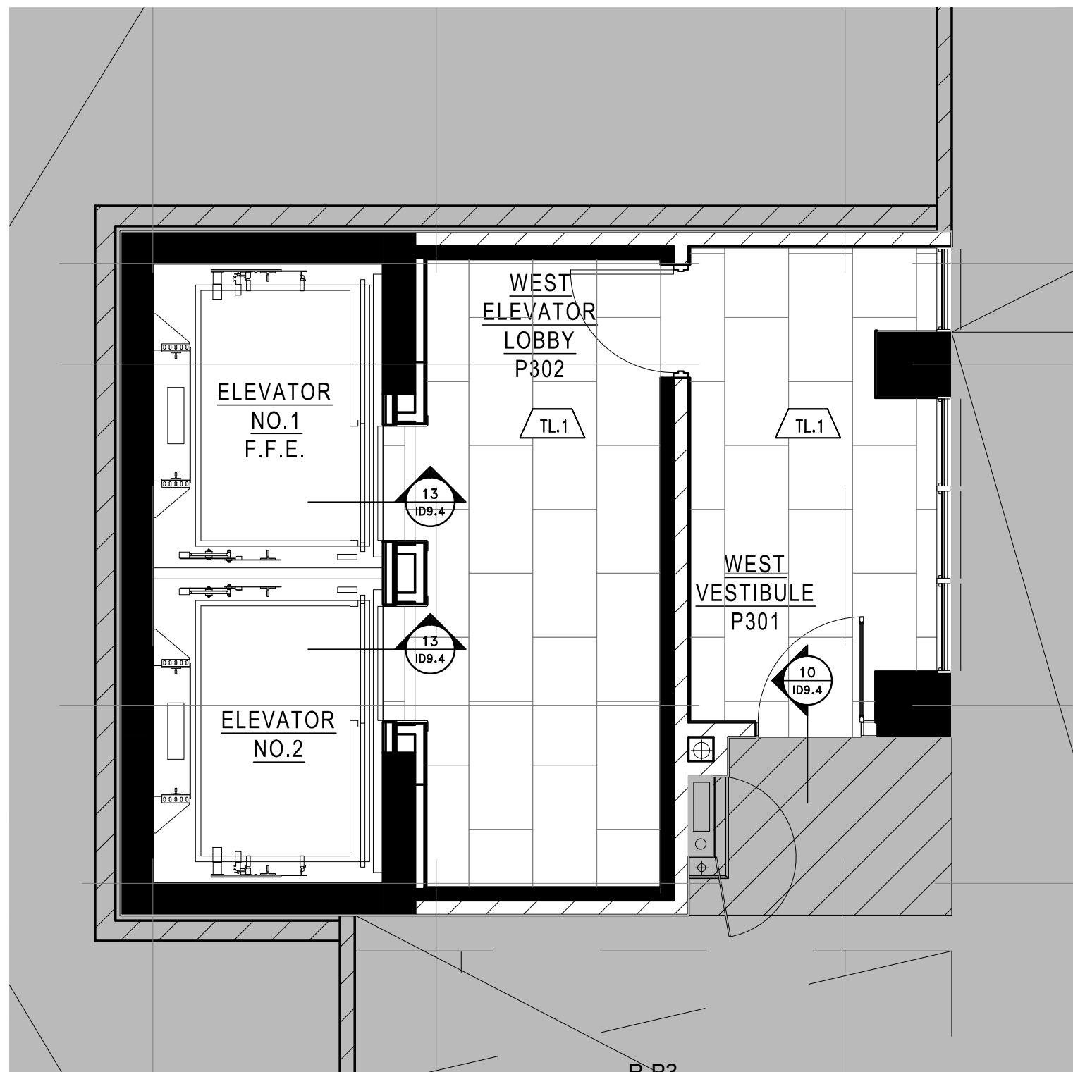
6 FLOOR FINISH PLAN R3.2 SCALE 1:50
