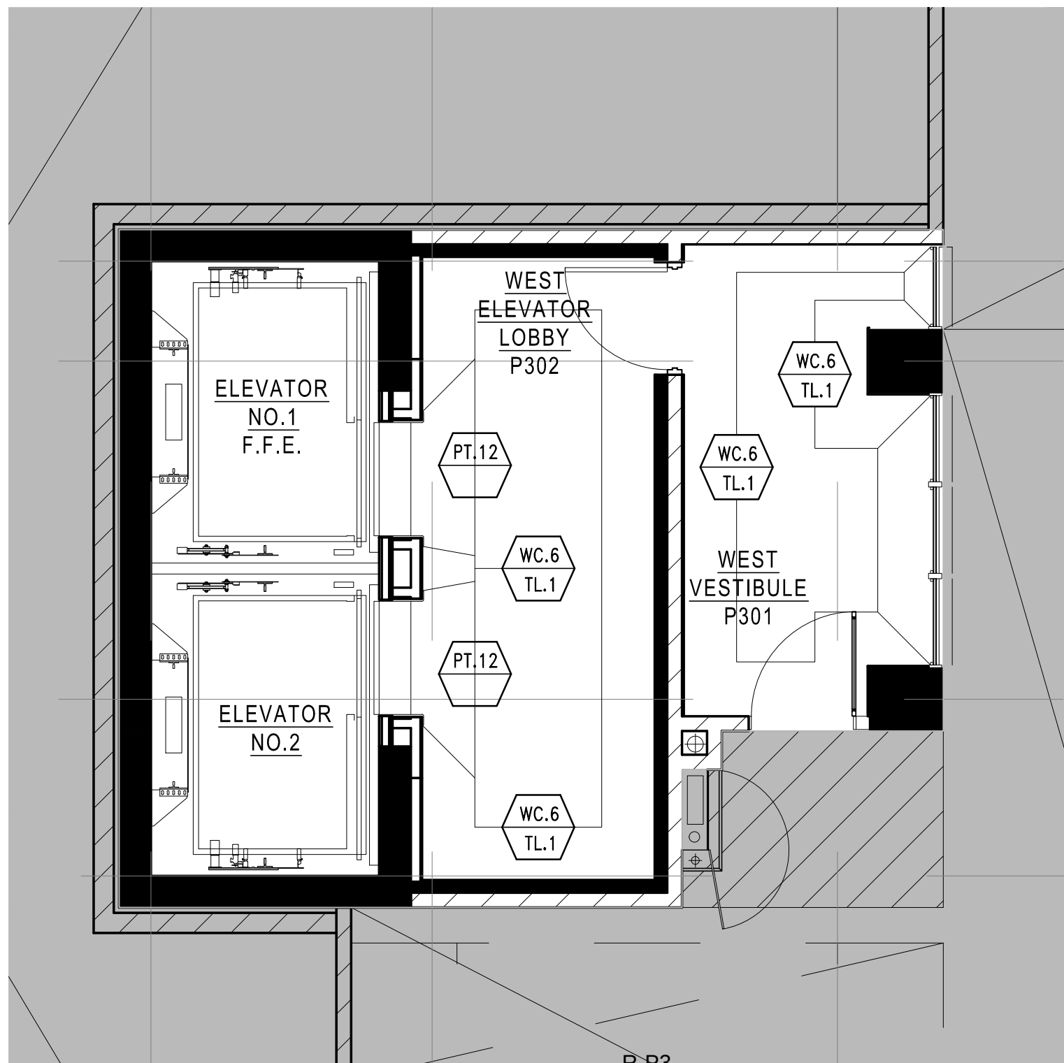
5 WALL FINISH PLAN R3.2 SCALE 1:50
