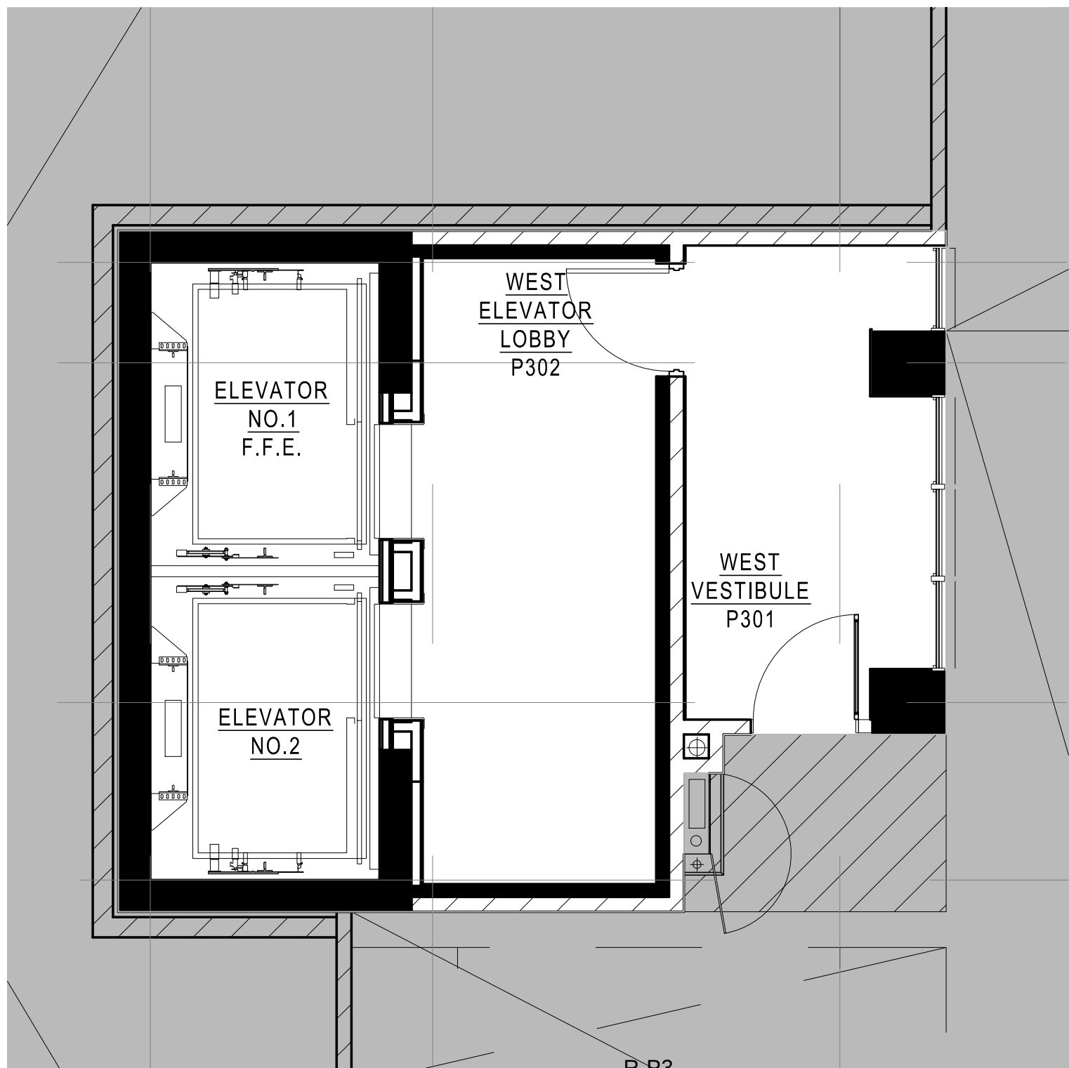
4 FURNITURE PLAN R3.2 SCALE 1:50
