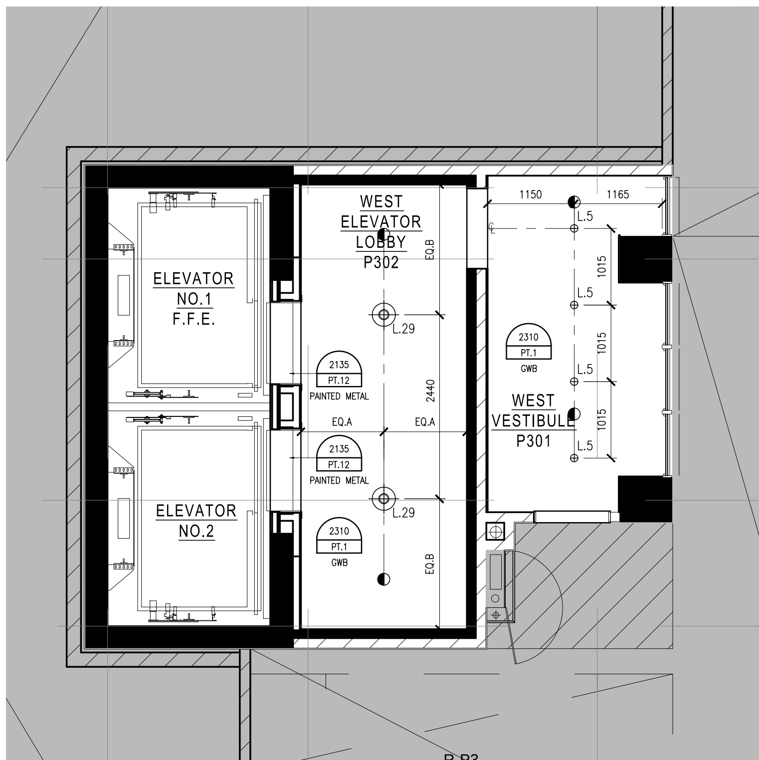
2 REFLECTED CEILING PLAN R3.2 SCALE 1:50
