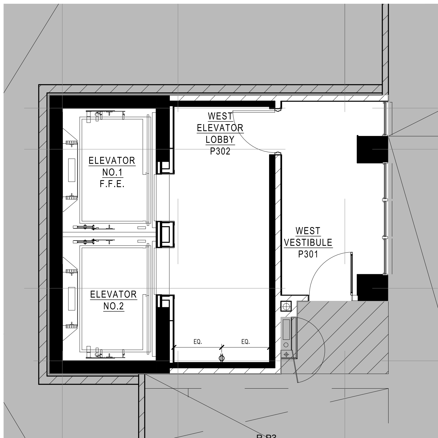
3 POWER AND COMMUNICATION PLAN R3.2 SCALE 1:50
