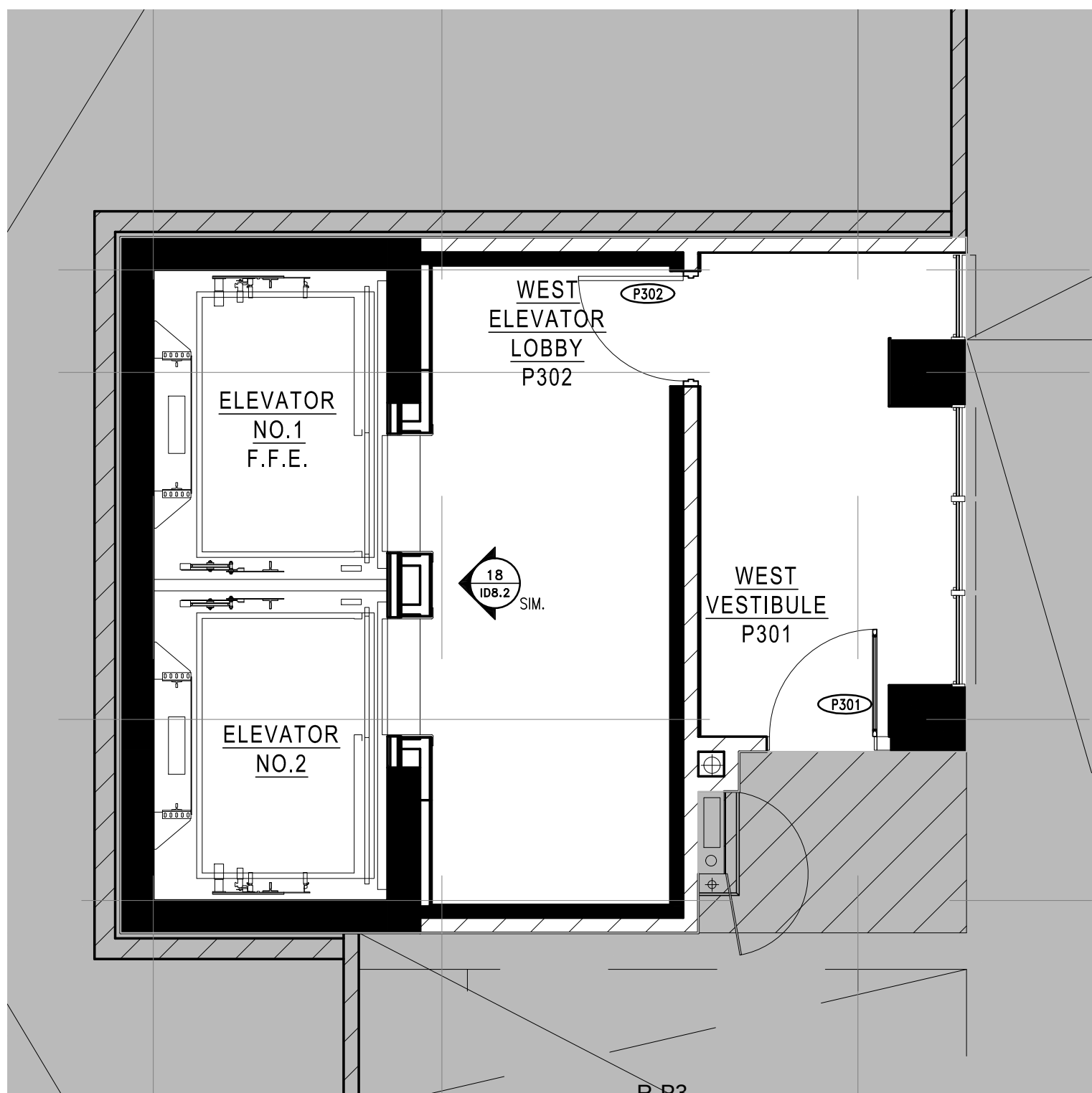
1 CONSTRUCTION PLAN R3.2 SCALE 1:50
