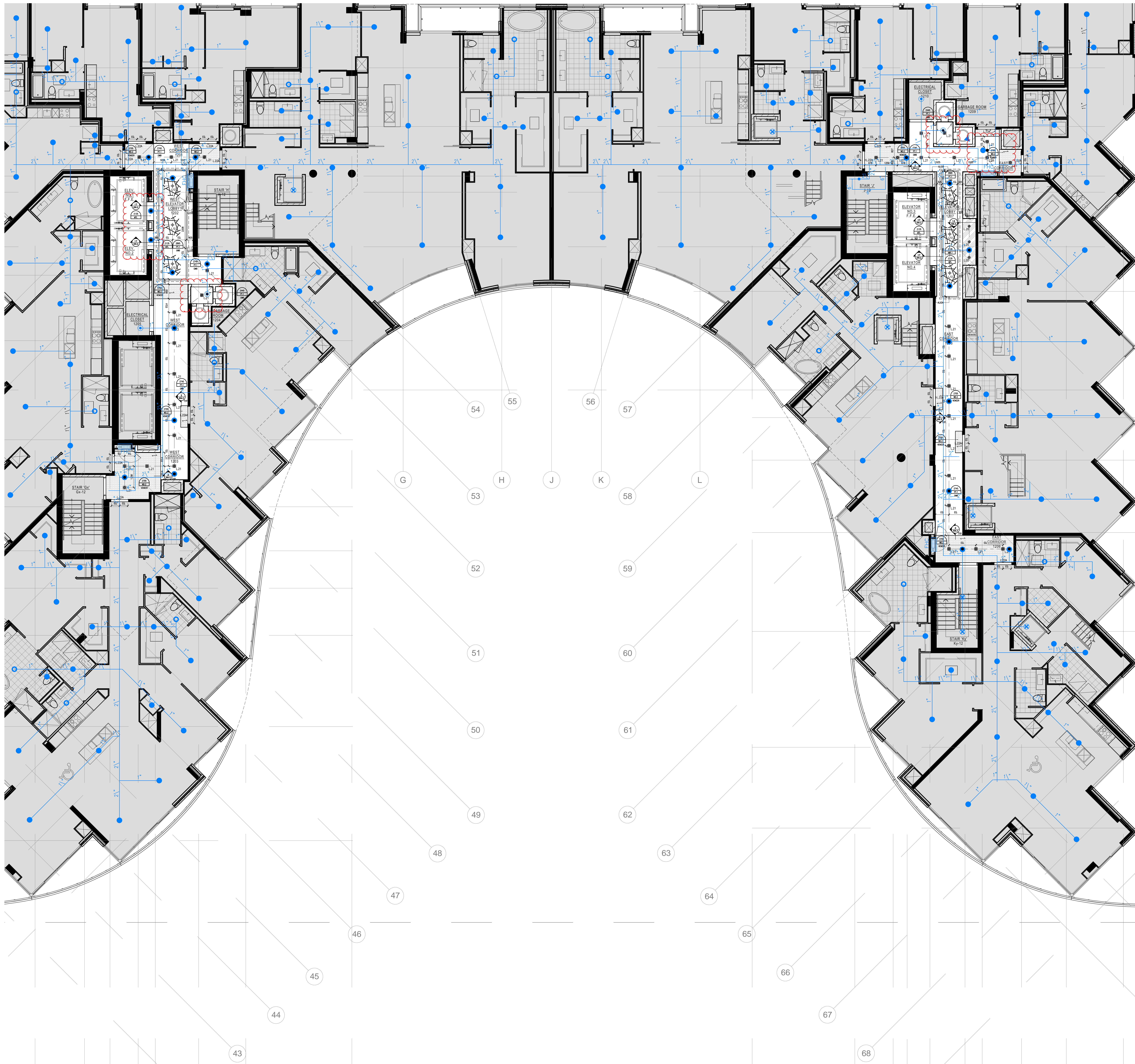
1 REFLECTED CEILING PLAN 03.18 SCALE: 1:75
