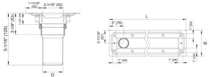
Dimensional Chart
