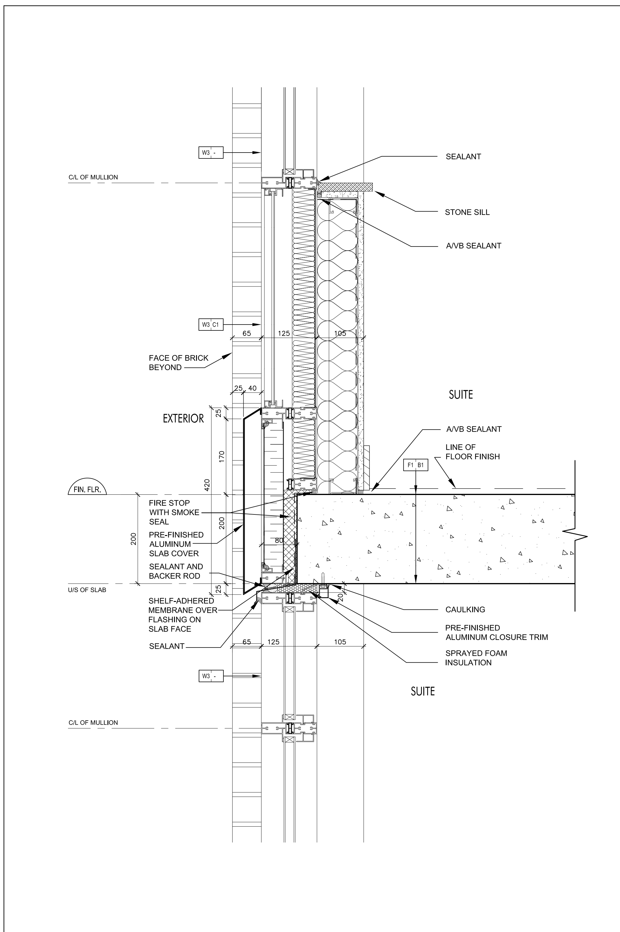
Pre-Finished Aluminum Slab Cover @ Window Wall 6 SCALE 1:5 A7-11
