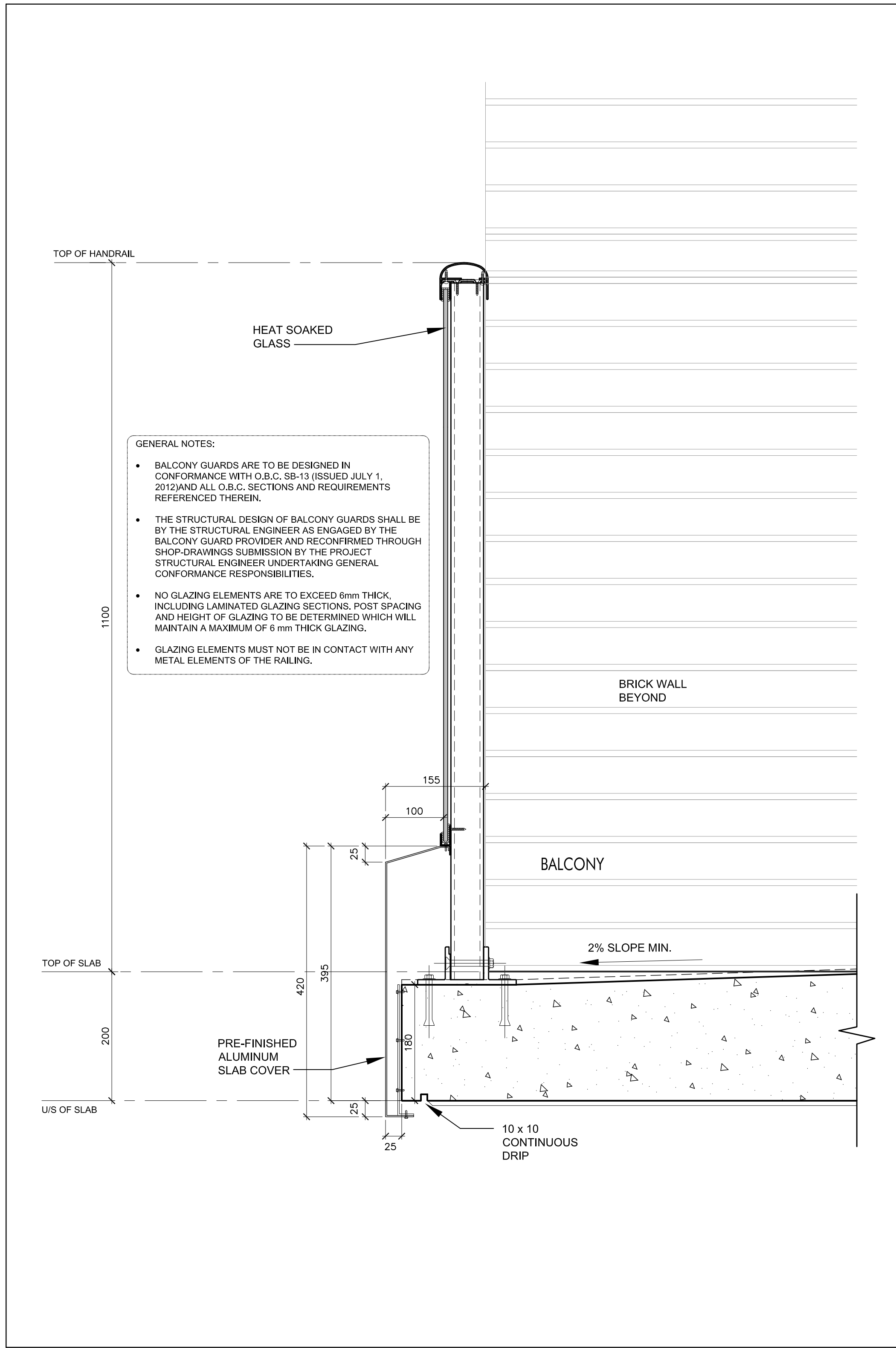
Railing @ Balcony 7 SCALE 1:5 A7-11
