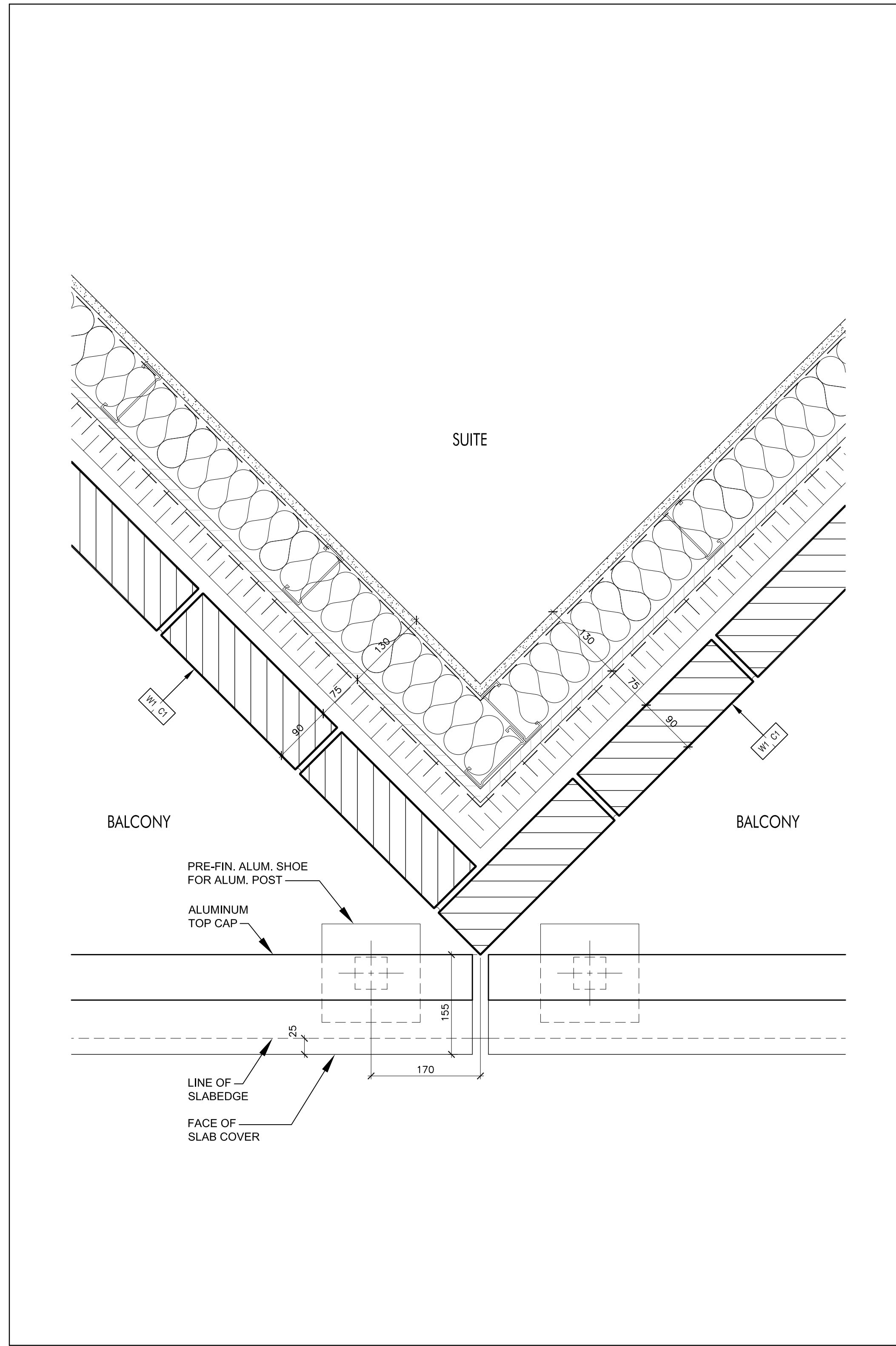
Plan Detail @ Balcony Railing @ Brick wall 8 SCALE 1:5 A7-11
