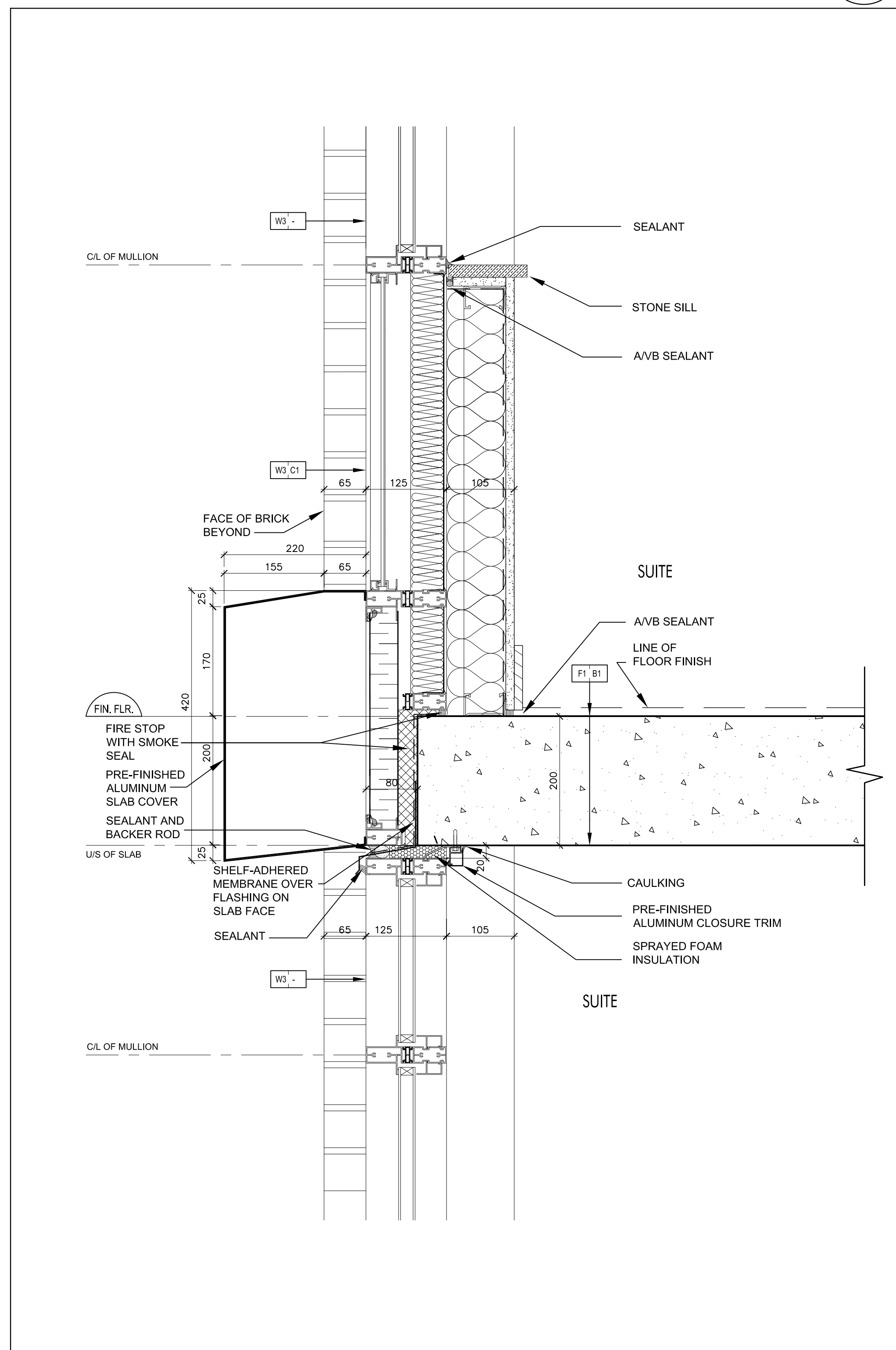
Pre-Finished Aluminum Slab Cover @ Window Wall 3 SCALE 1:5 A7-11
