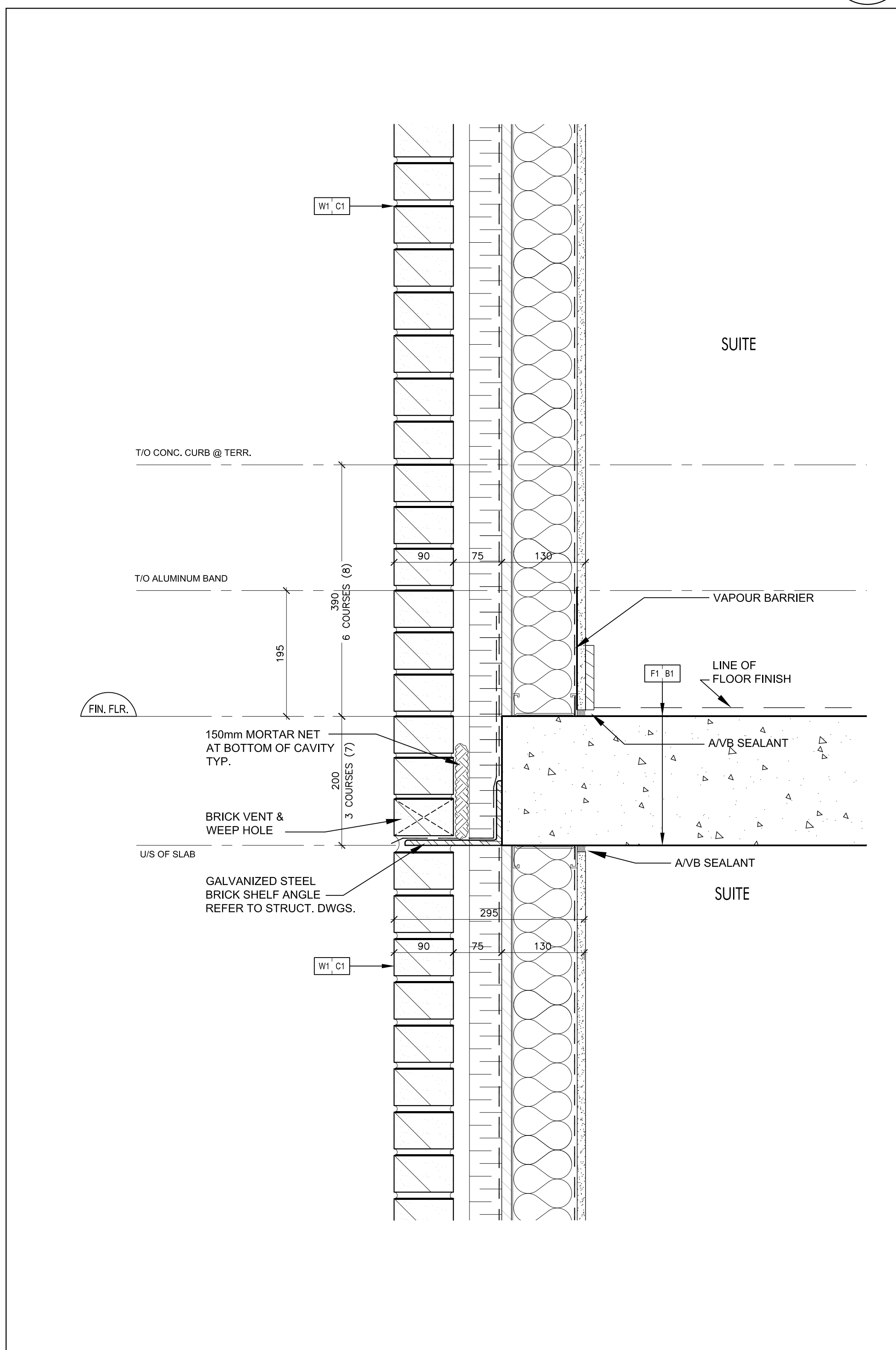
Typical Brick Coursing @ Concrete Slab 1 SCALE 1:5 A7-11
