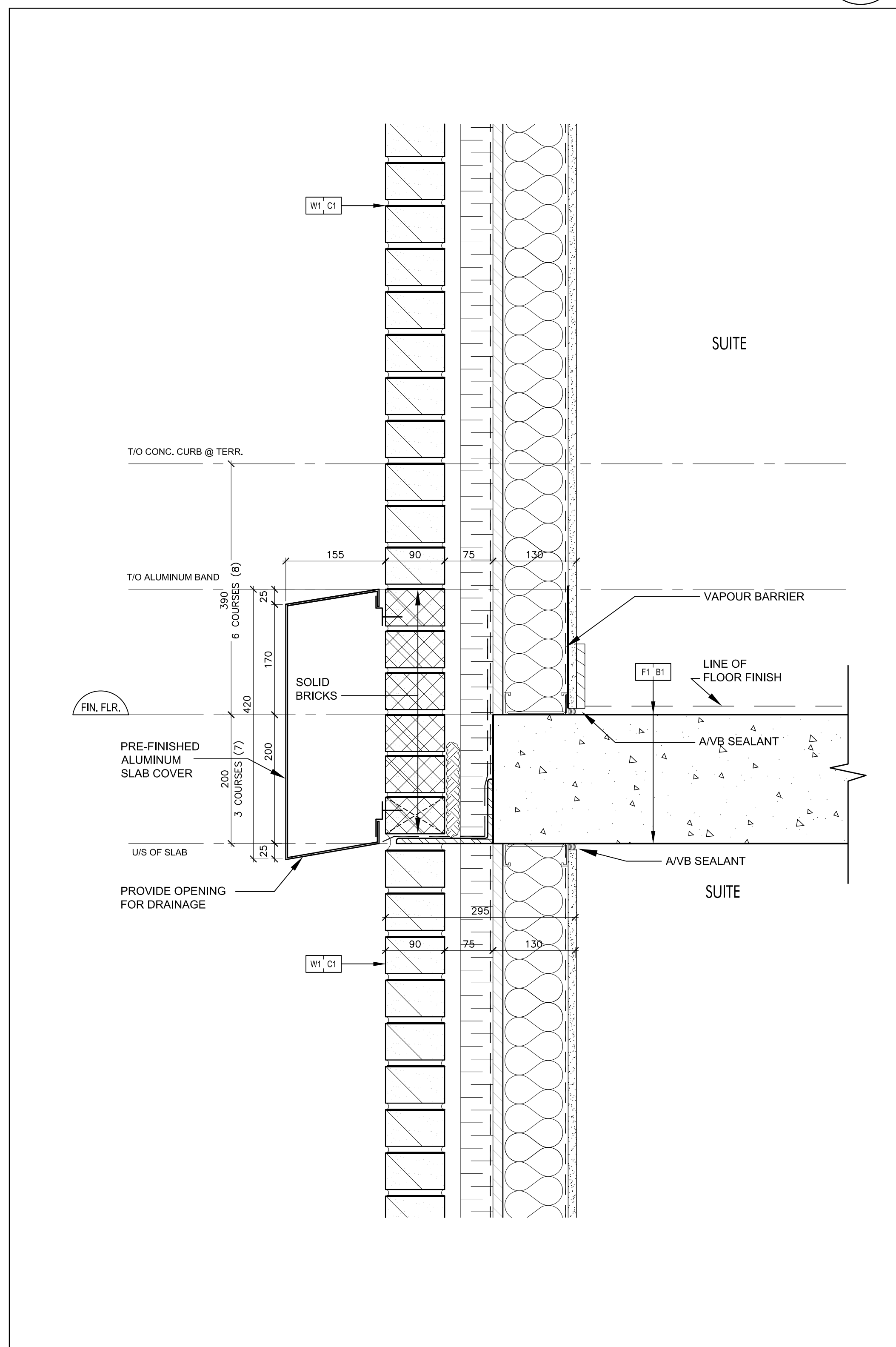
Pre-Finished Aluminum Slab Cover @ Brick Wall 2 SCALE 1:5 A7-11
