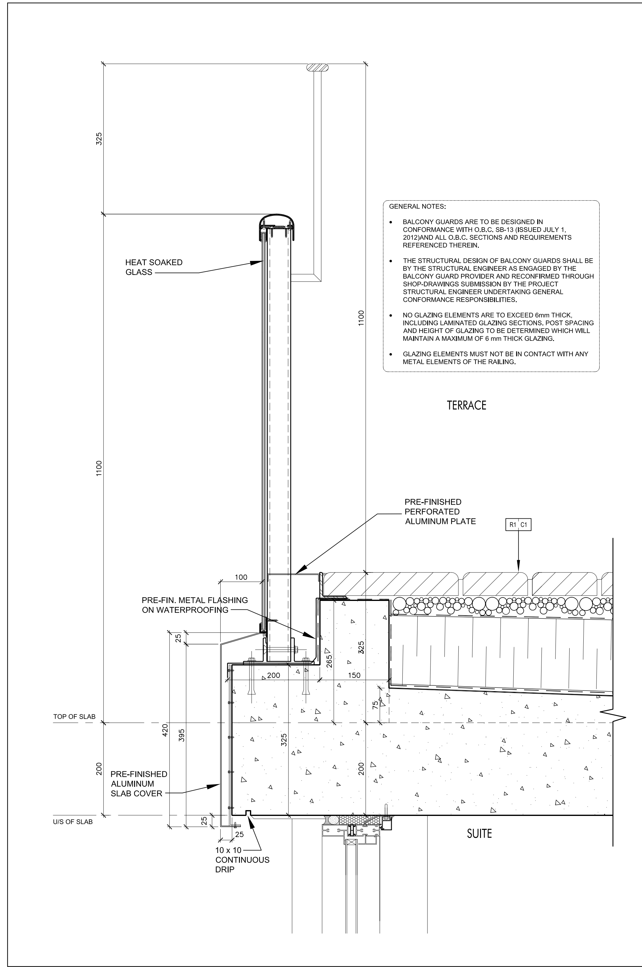
Railing @ Terrace 9 SCALE 1:5 A7-11
