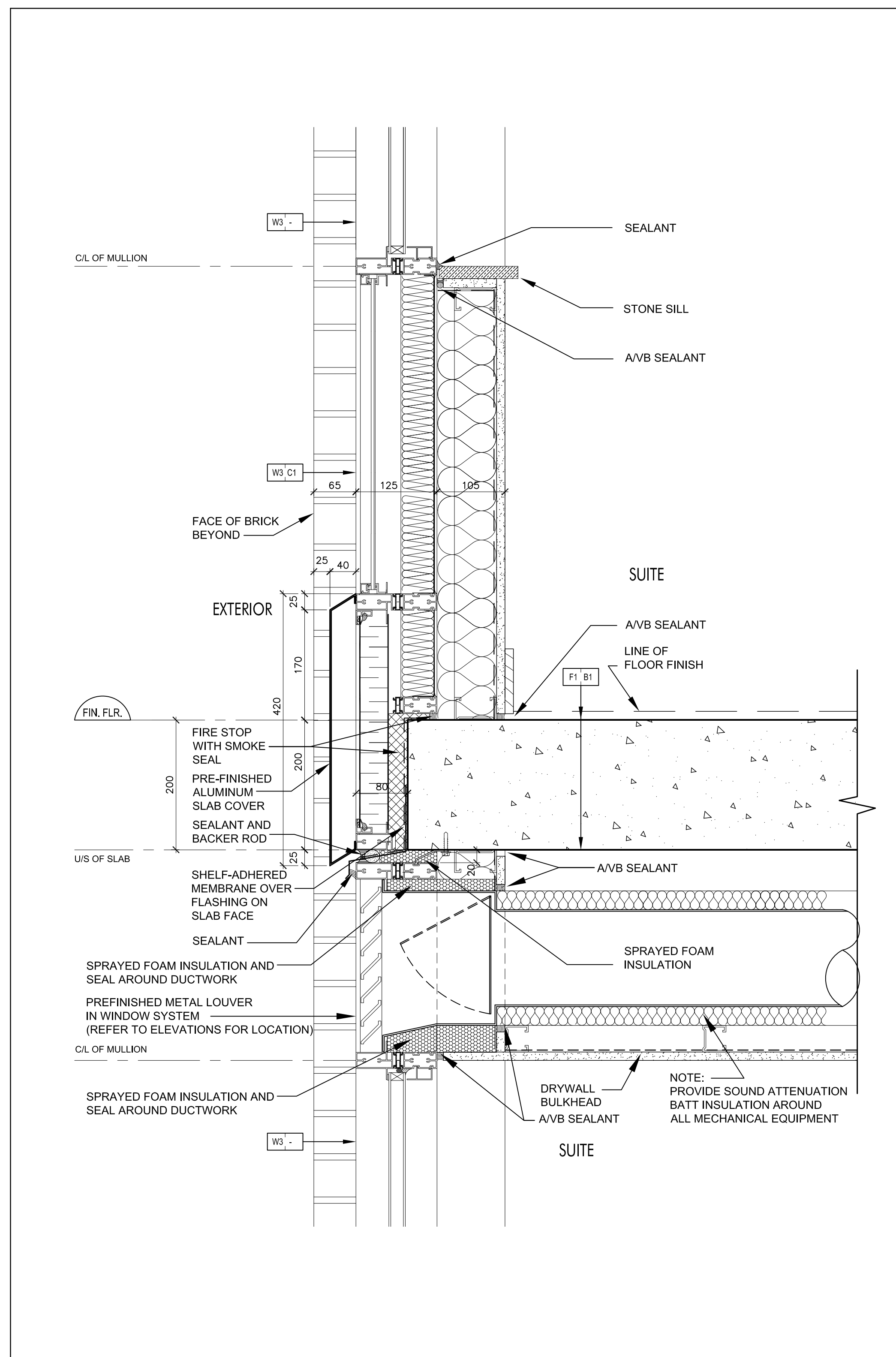
Pre-Finished Aluminum Slab Cover @ Window Wall 5 SCALE 1:5 A7-11
