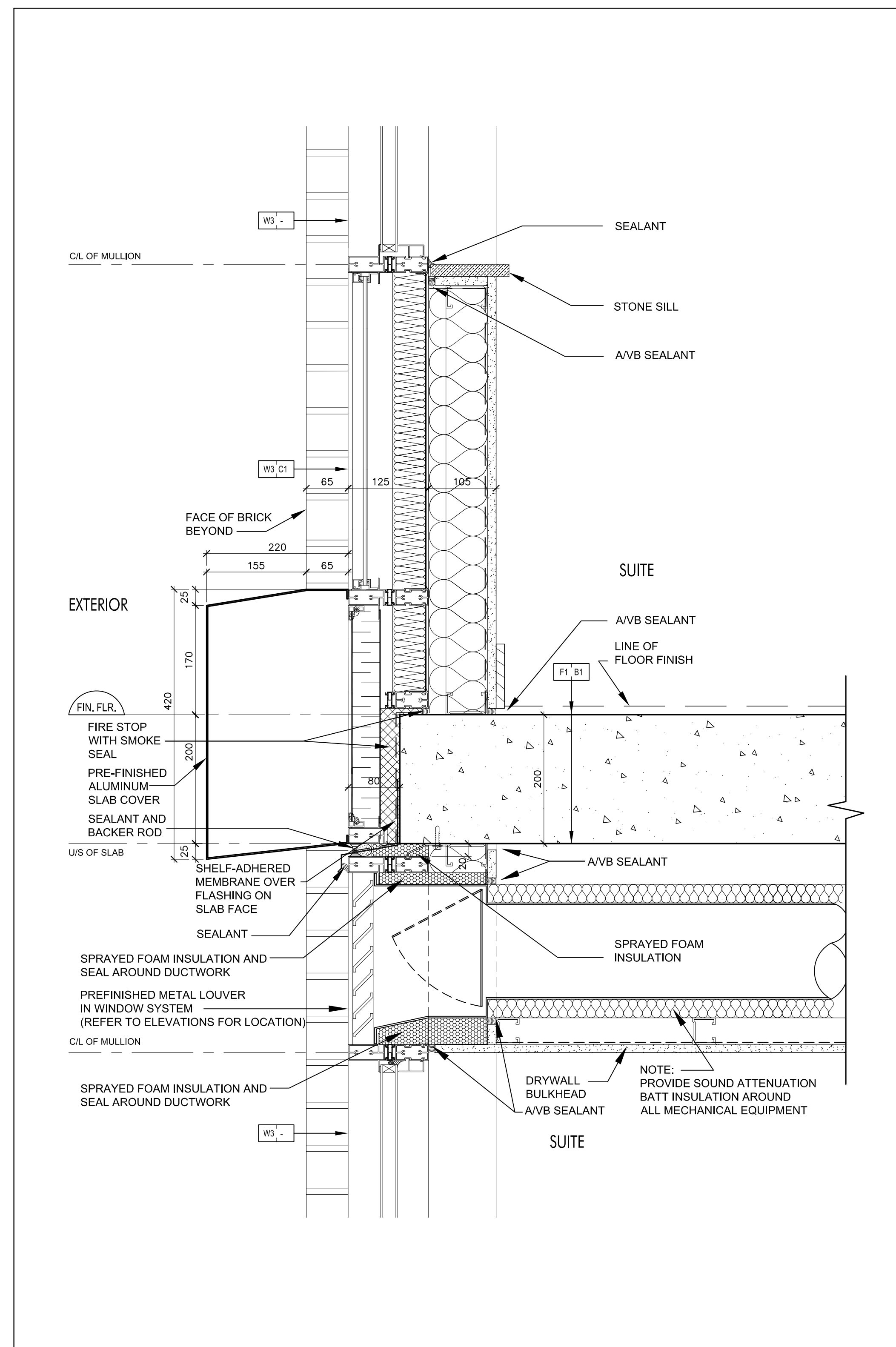
Pre-Finished Aluminum Slab Cover @ Window Wall 4 SCALE 1:5 A7-11
