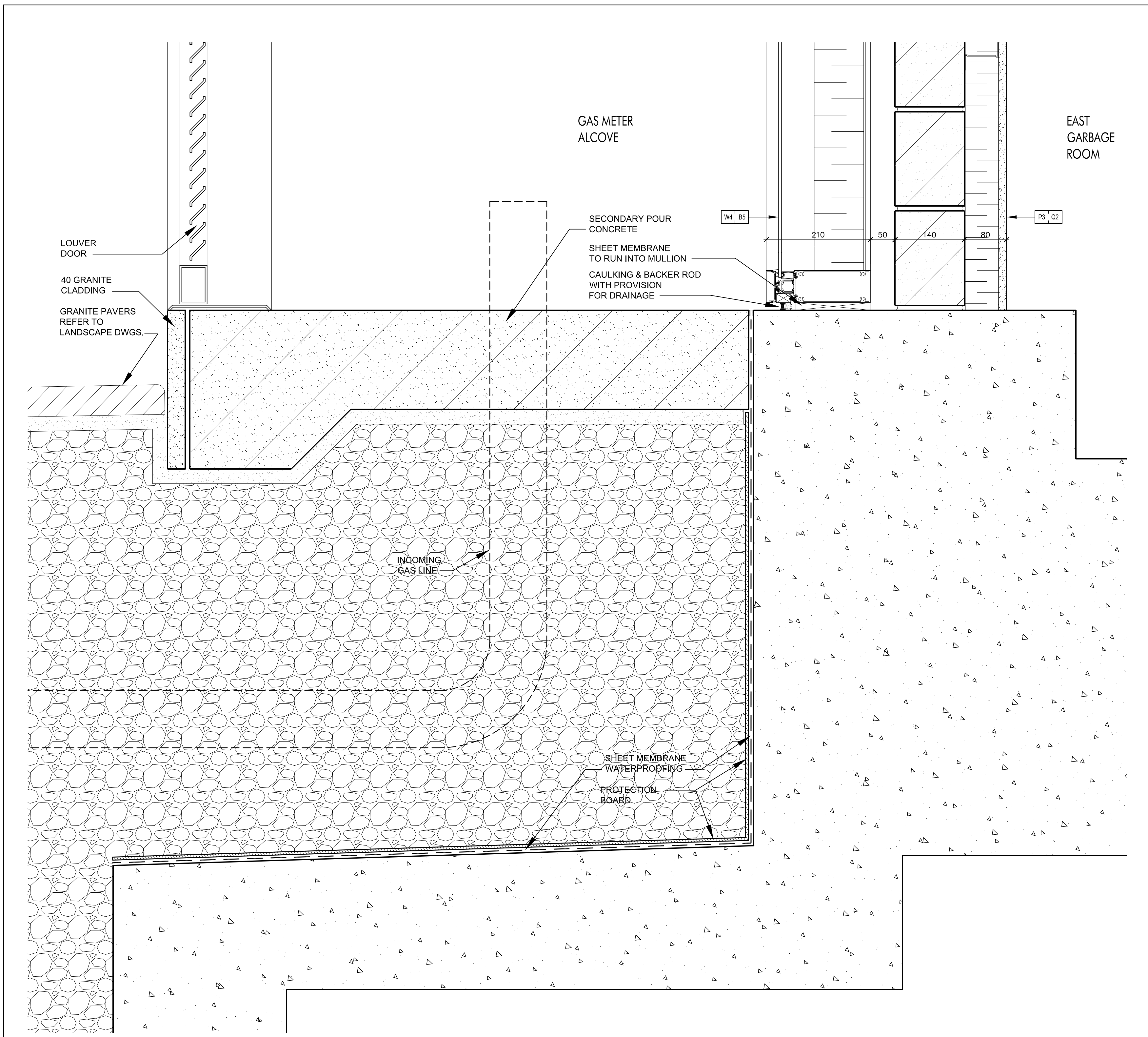
Curtain Wall Sill @ Gas Meter Alcove 9 SCALE 1:5 A7-08
