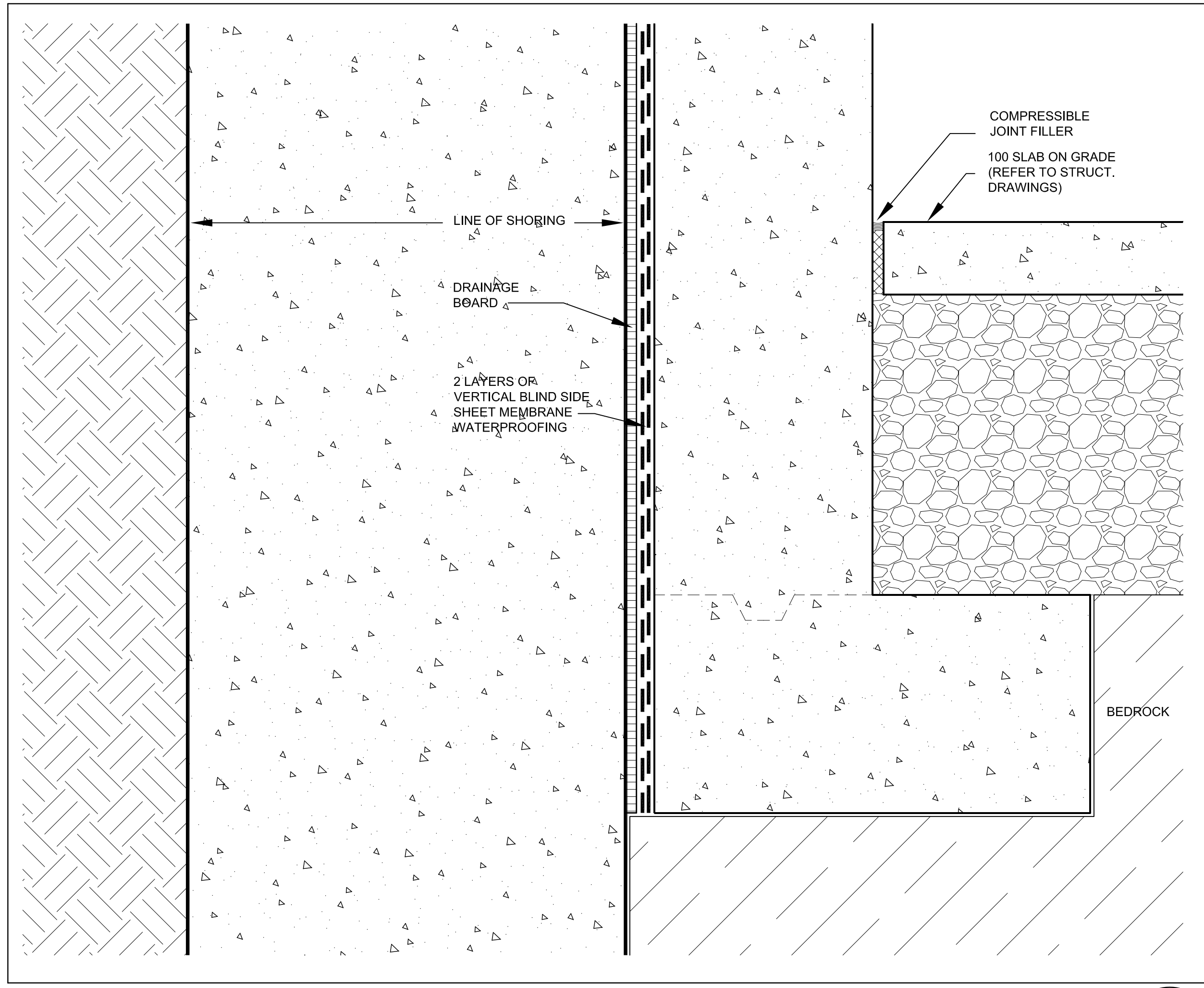
Foundation Wall @ Caisson Wall 5 SCALE 1:5 A7-08
