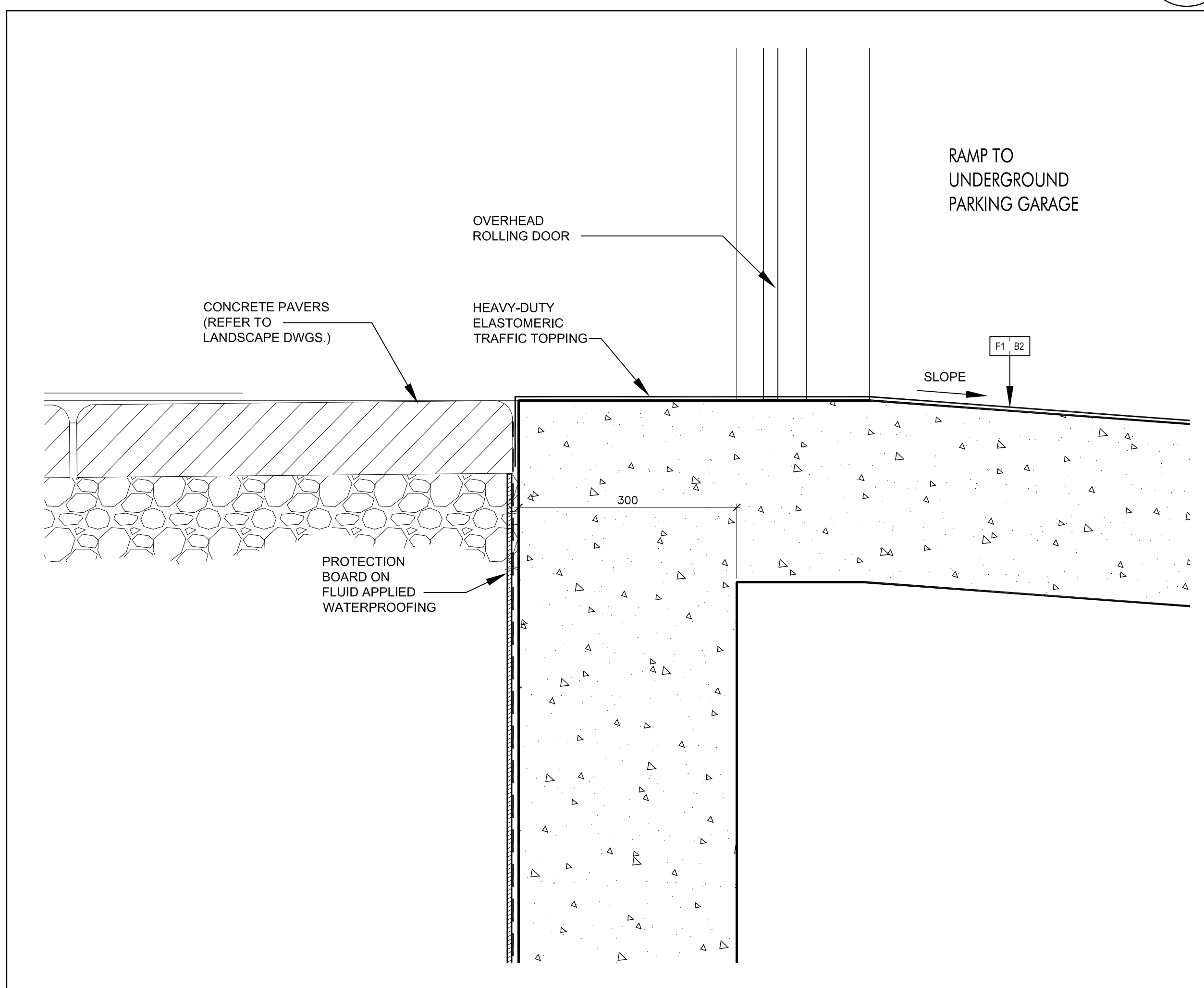
Entrance to Residential Parking 1 SCALE 1:5 A7-08
