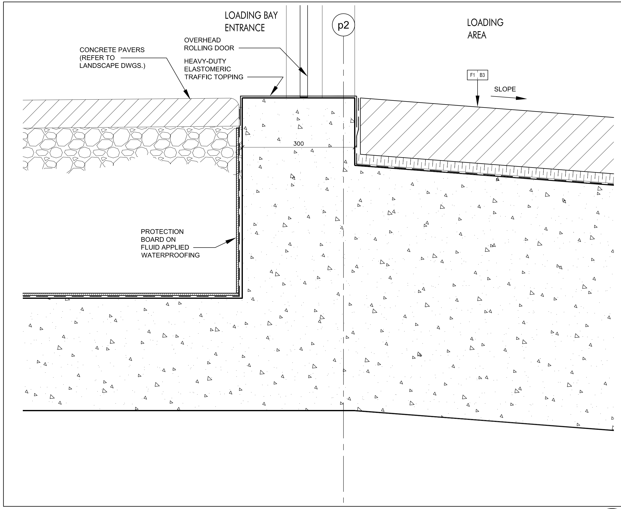
Entrance & O/H Door @ Loading Area 2 SCALE 1:5 A7-08
