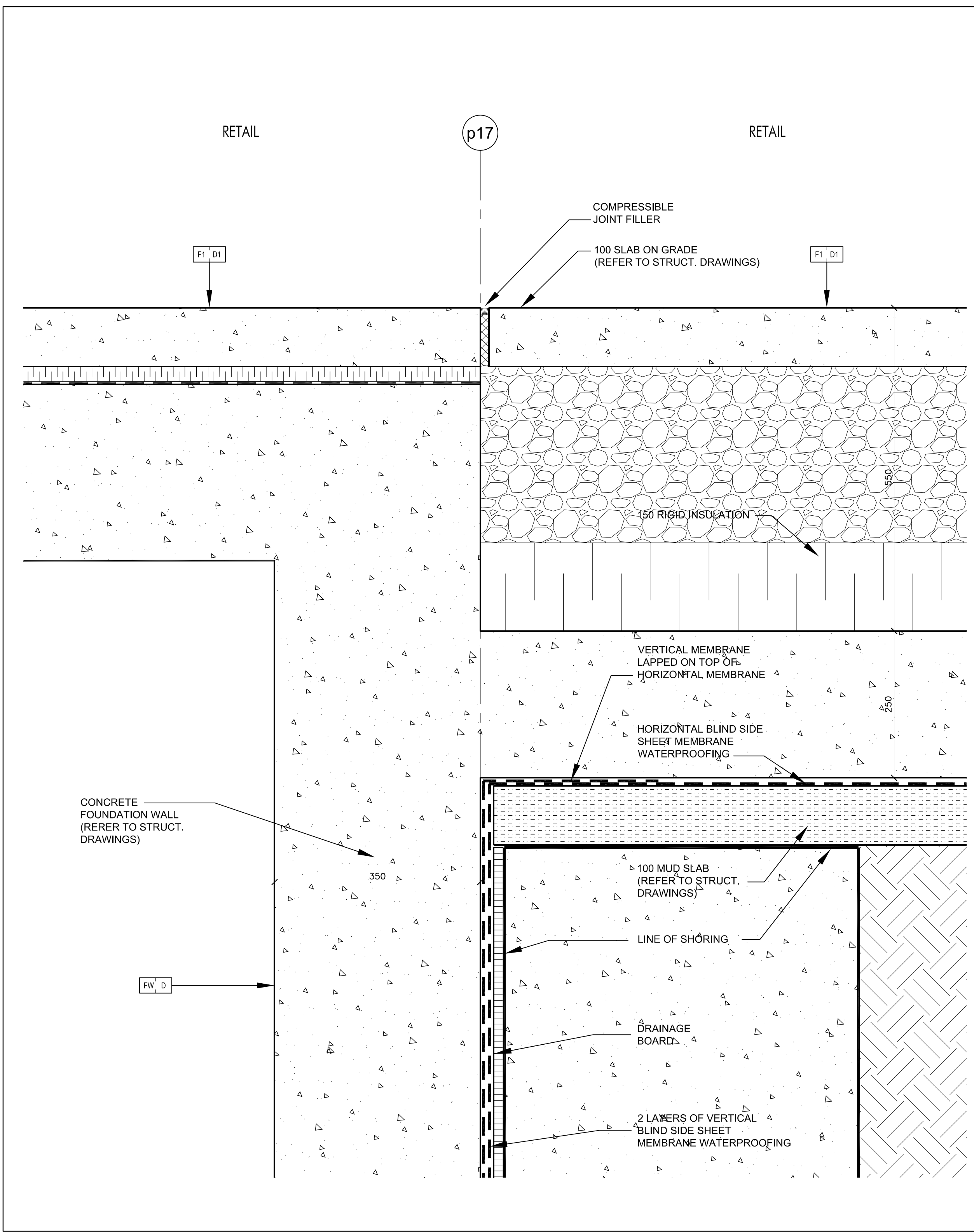
Foundation Wall @ Caisson Wall 8 SCALE 1:5 A7-08
