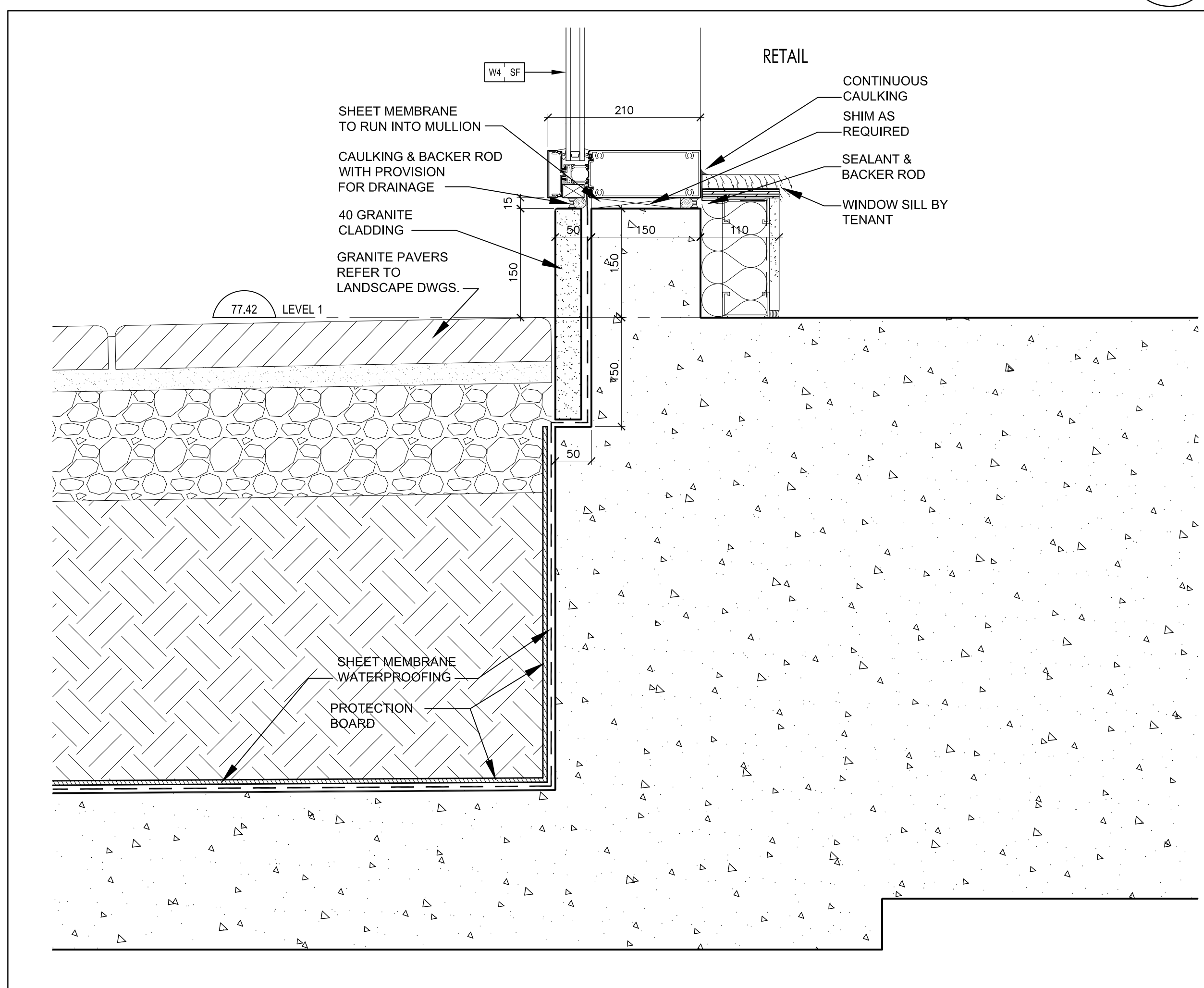
Typical Curtain Wall Sill @ Retail 4 SCALE 1:5 A7-08
