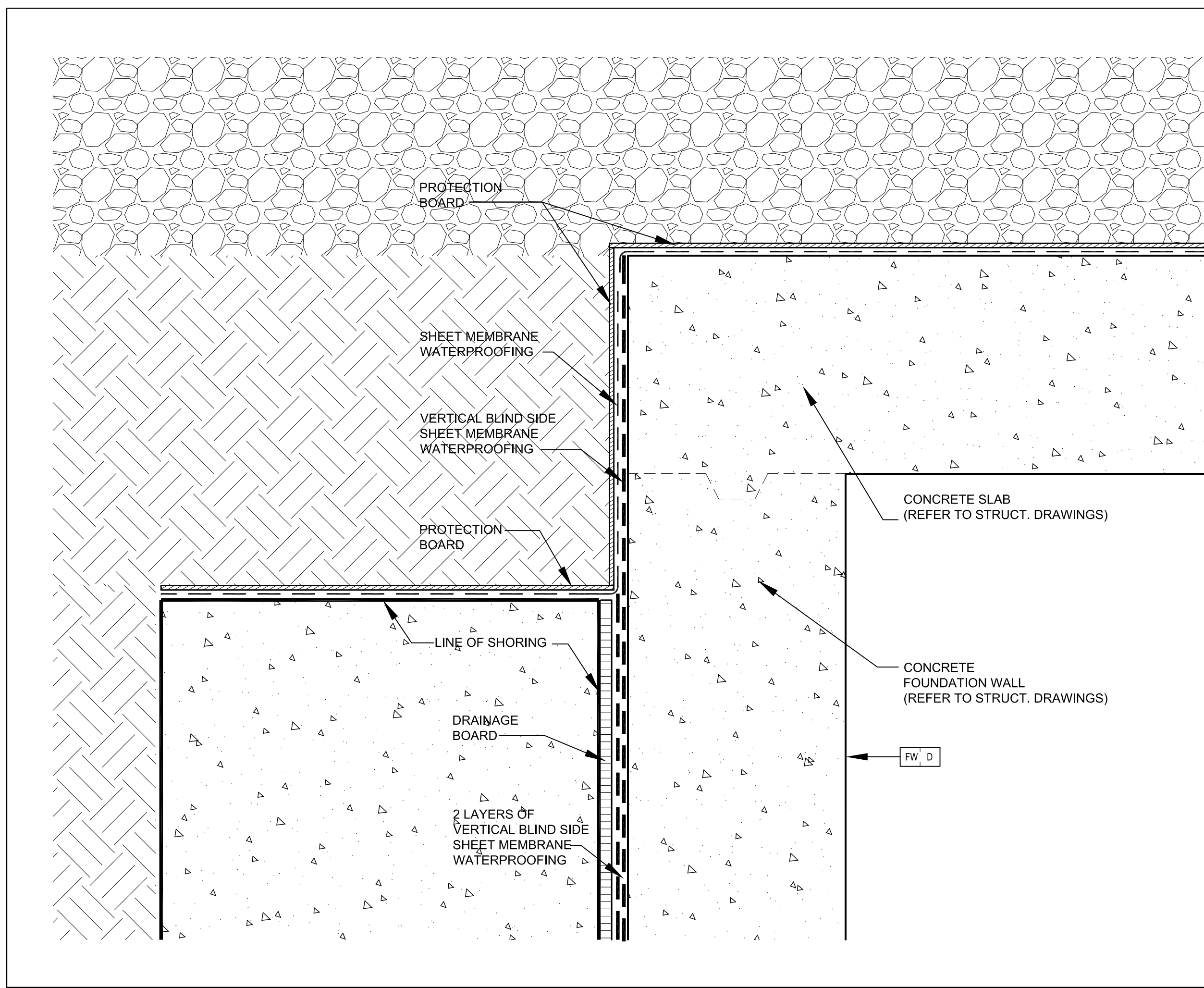
Foundation Wall @ Caisson Wall 3 SCALE 1:5 A7-08
