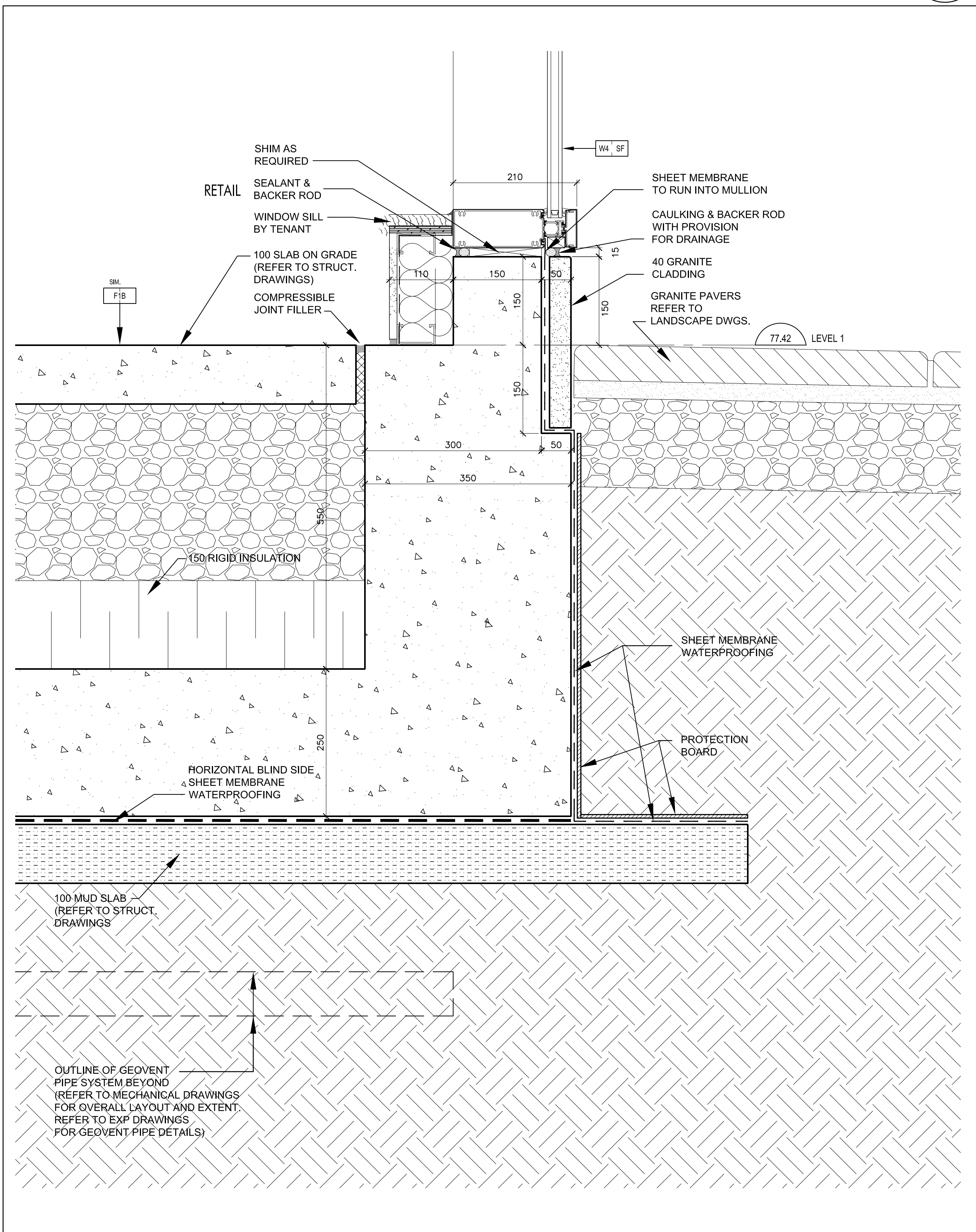
Curtain Wall Sill @ Retail 7 SCALE 1:5 A7-08
