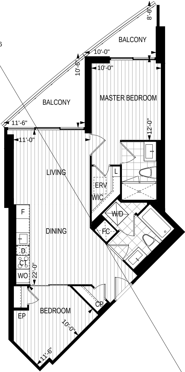
BALCONY PLAN: FLOORS 4, 6 2A1
