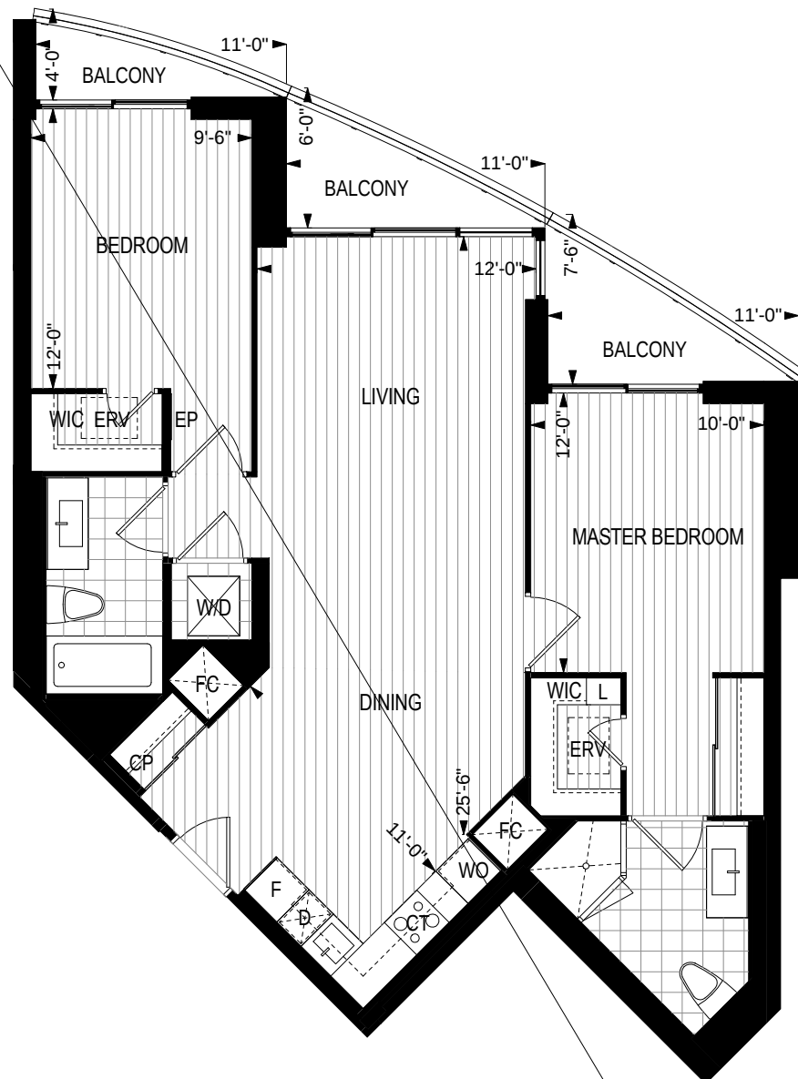
BALCONY PLAN: LEVELS 3, 5 2F1
