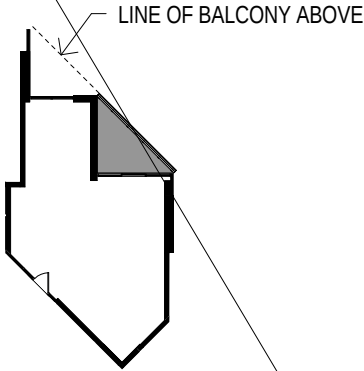
PARTIAL BALCONY PLAN: LEVELS 8, 10 1B+D1
