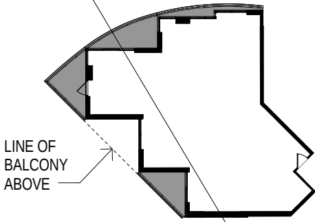
PARTIAL BALCONY PLAN: LEVELS 8, 10 S8-1
