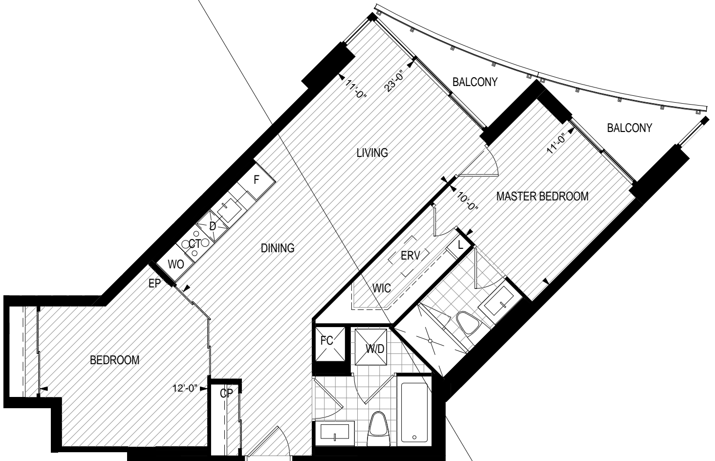
PARTIAL BALCONY PLAN: LEVEL 3-6
