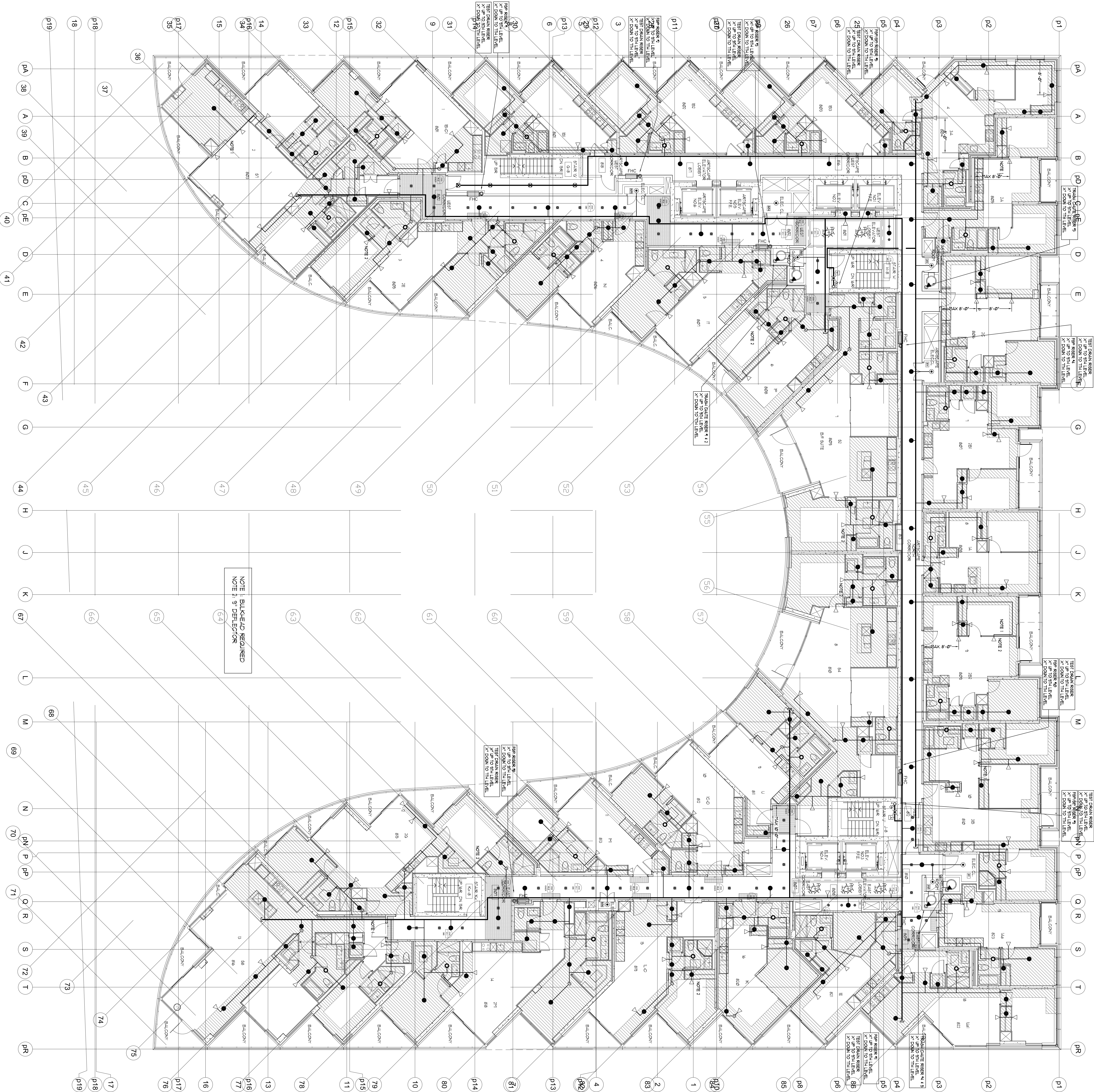
8TH LEVEL SPRINKLER LAYOUT
