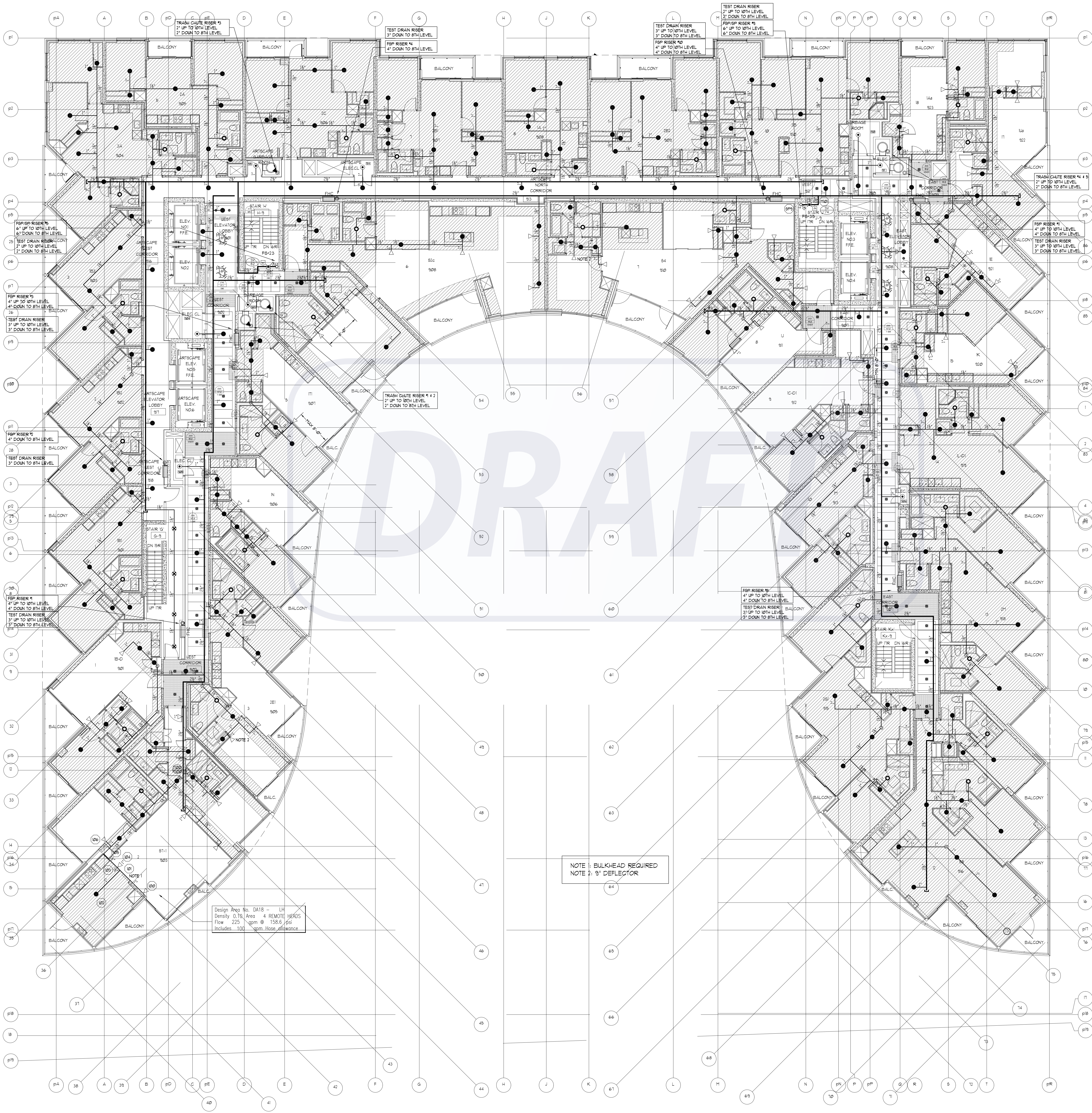
9TH LEVEL SPRINKLER LAYOUT SCALE: 1/8" = 1'-0"
