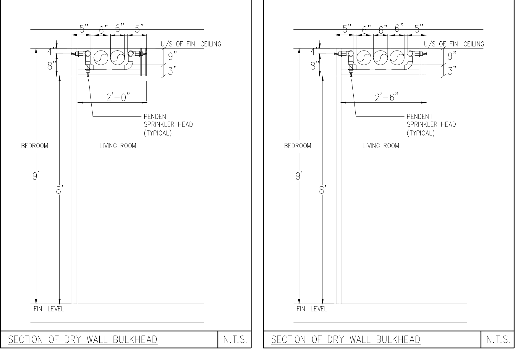
SPRINKLER DUCKWORK DETAIL
