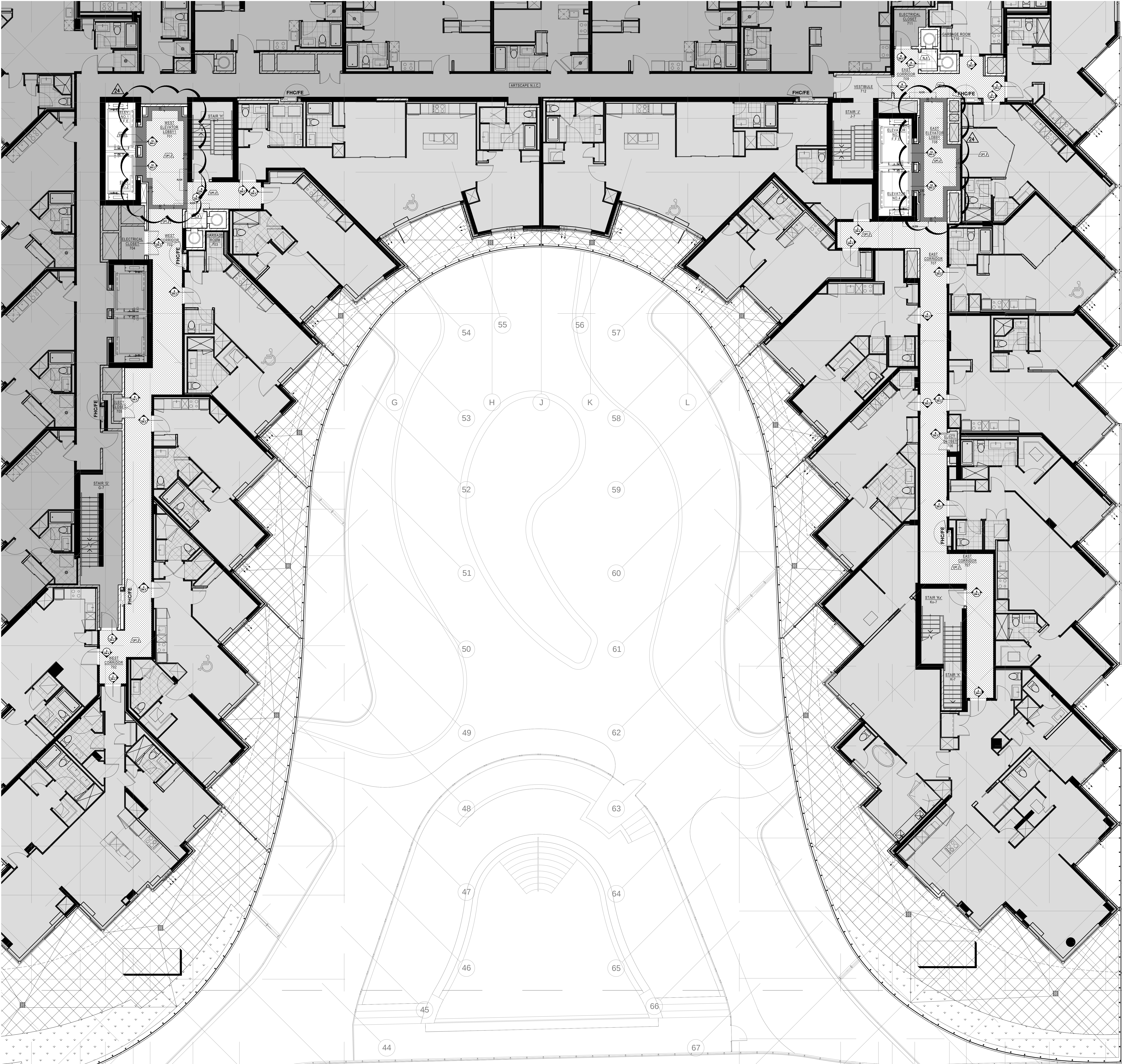
1 FLOOR FINISH PLAN 07.13 SCALE: 1:7.5
