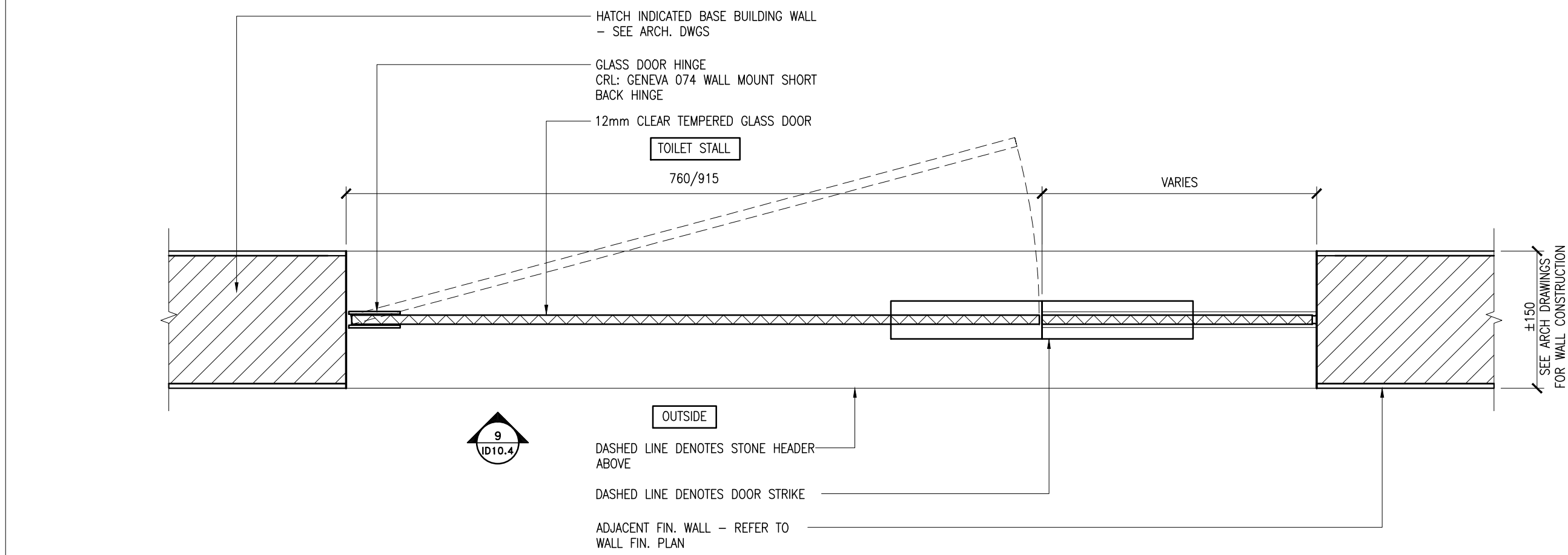
1 SECTION 1:10 SCALE
