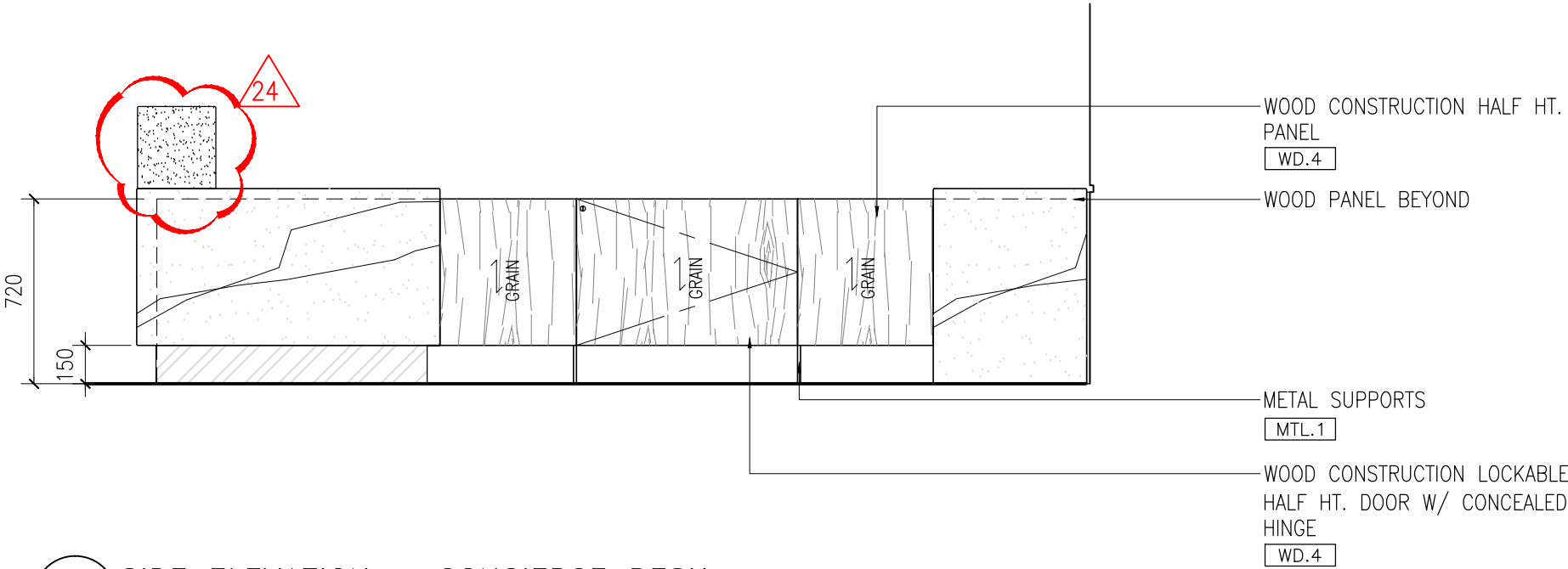
1 SIDE ELEVATION – CONCIERGE DESK D1.02.7 SCALE 1 : 2 5
