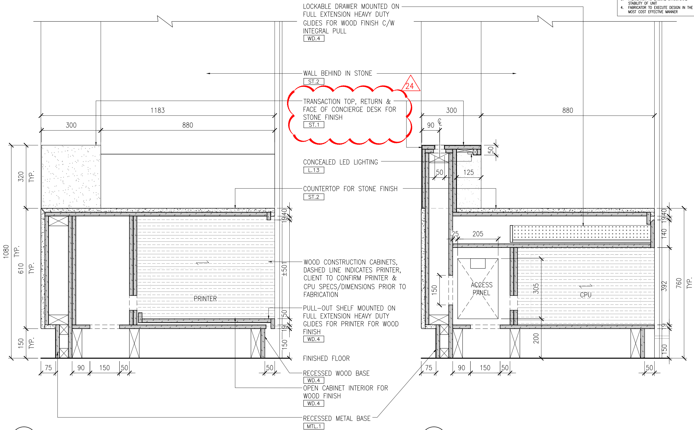
1 SECTION – CONCIERGE DESK D1.02.3 SCALE 1:1 O
