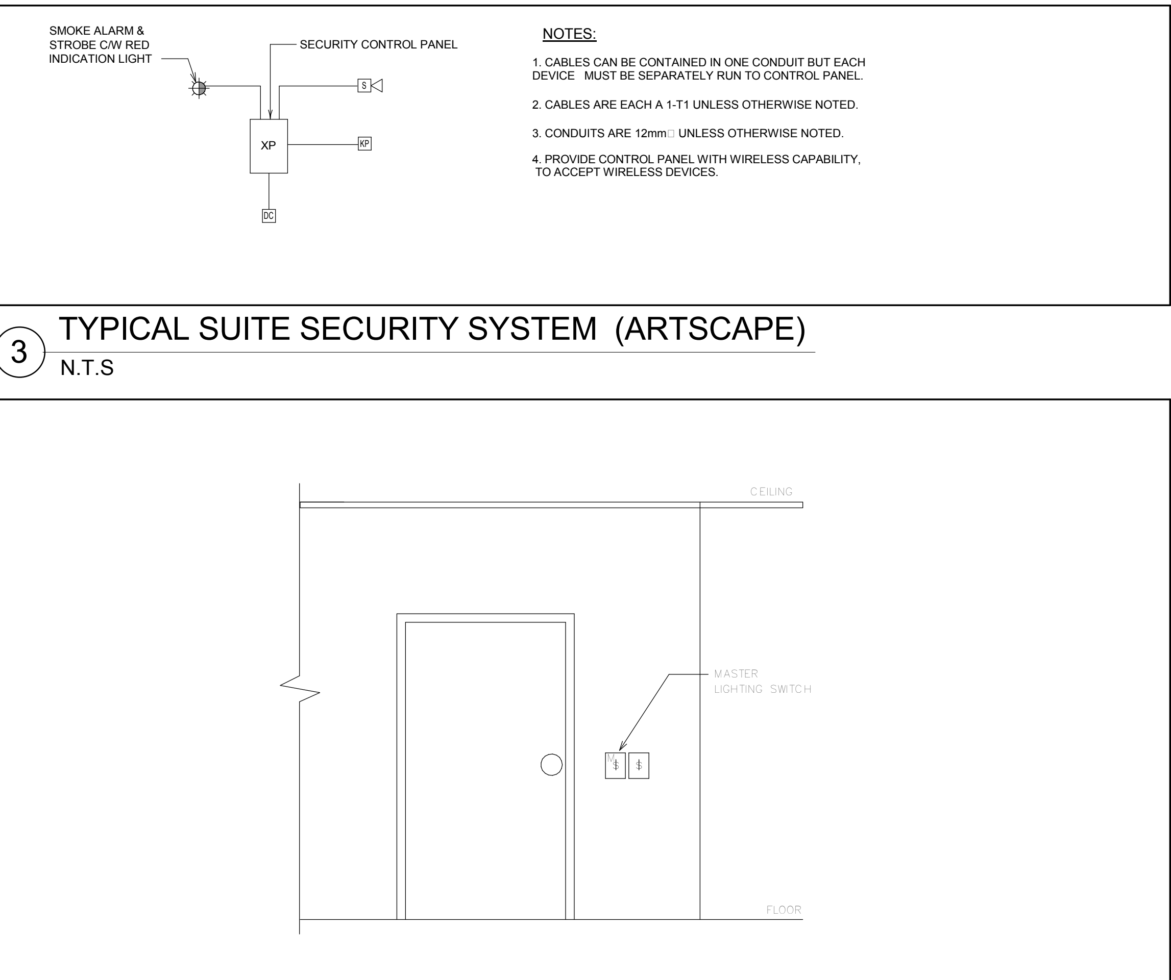
3 TYPICAL SUITE SECURITY SYSTEM (ARTSCAPE) N.T.S.
