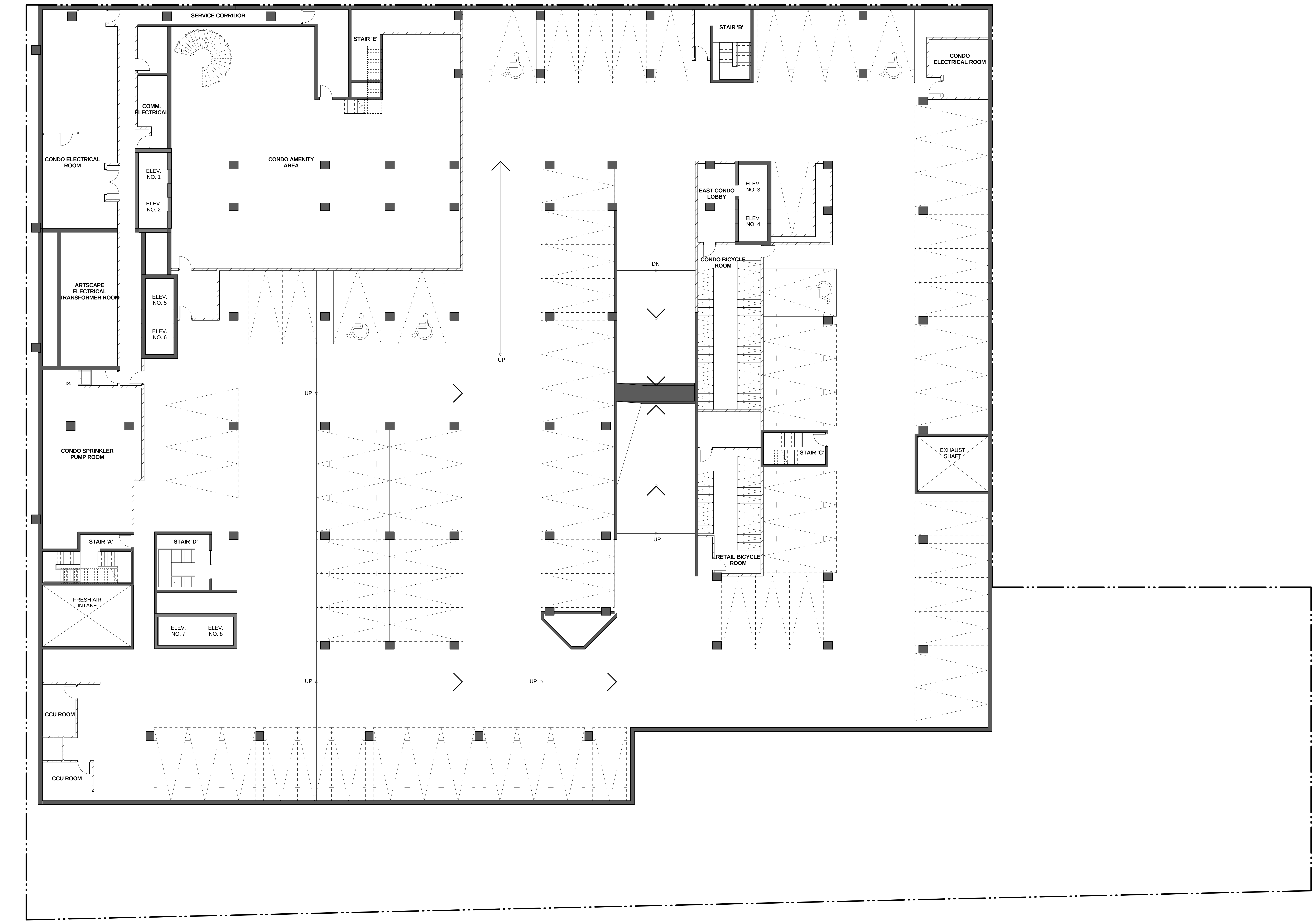
LEVEL P1 - 1:100
