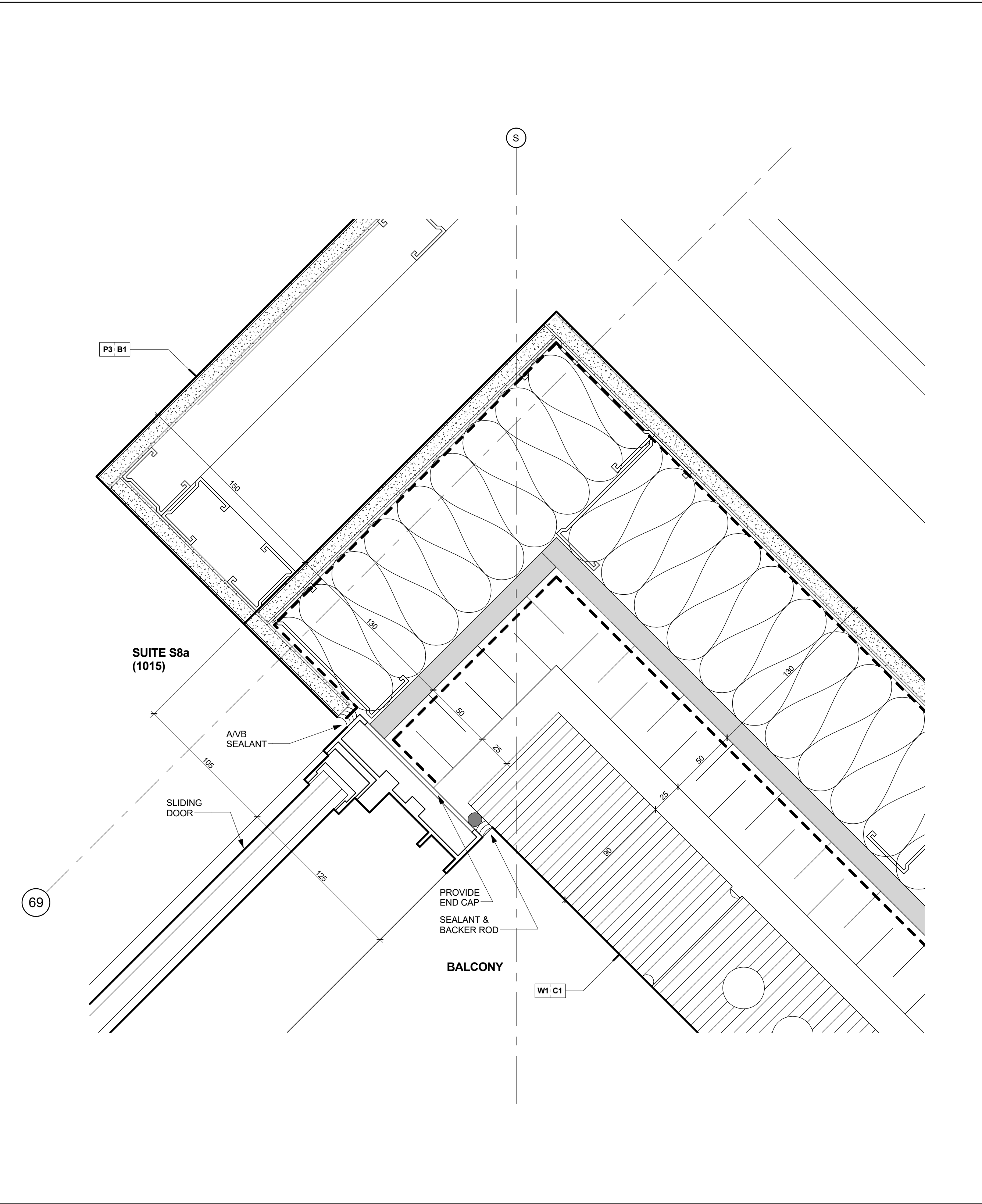
Enlarged Plan Detail @ Window Jamb @ Brick Veneer Wall with Metal Studs 3 Scale: 1 : 2 A7-25
