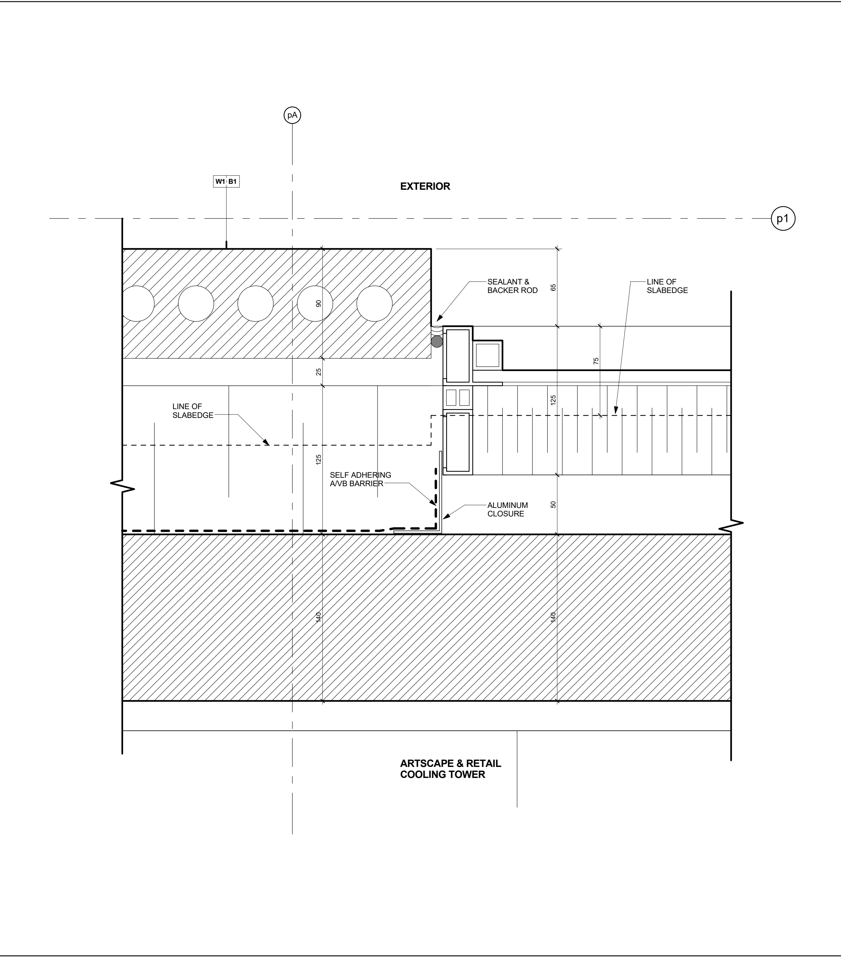
Enlarged Plan Detail @ Window Jamb @ Brick Veneer Wall with Conc. Block 4 Scale: 1 : 2 A7-25
