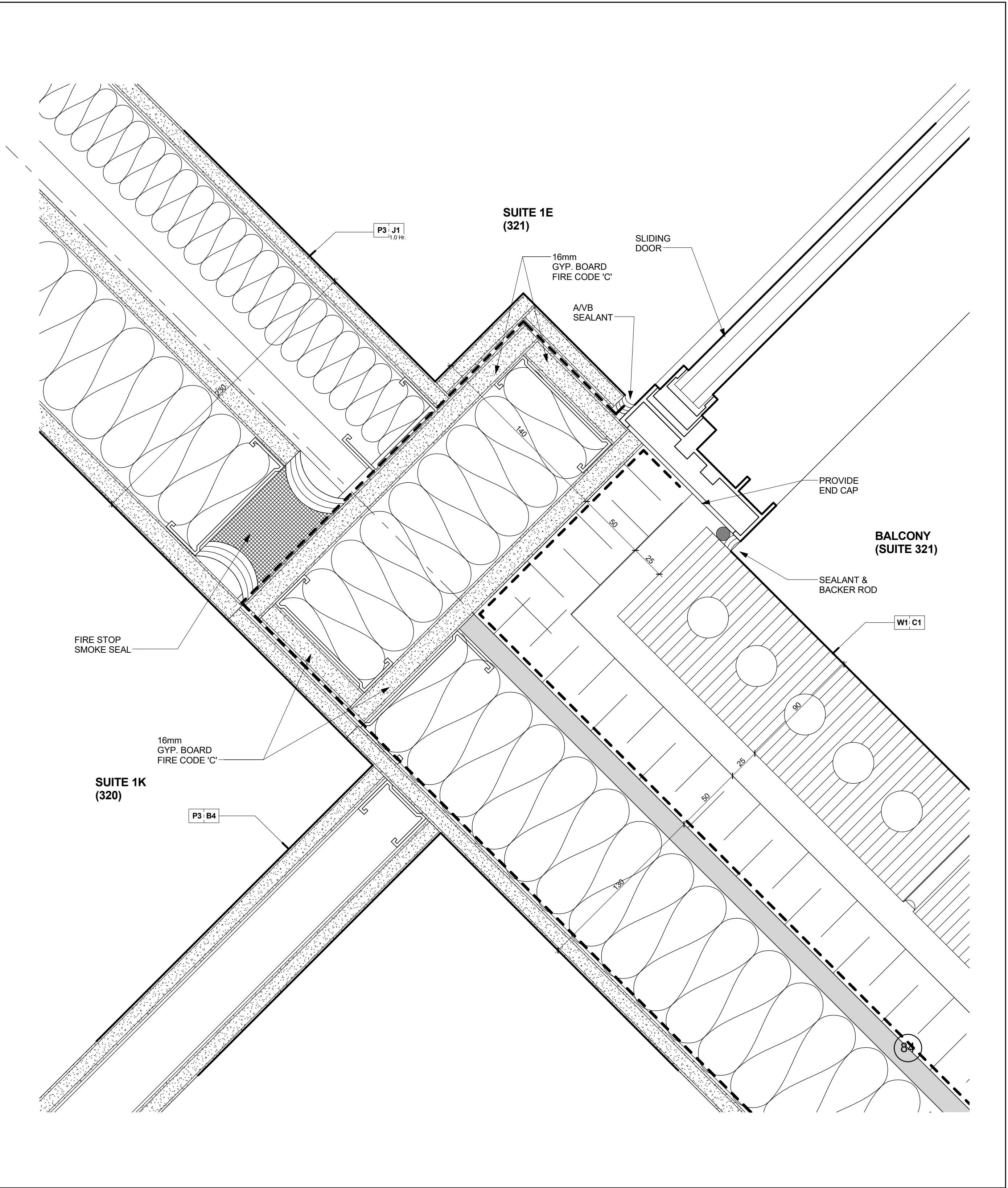
Enlarged Plan Detail @ Demising Wall (M/Studs) @ Brick Veneer Wall with Metal Studs 1 Scale: 1 : 2 A7-25
