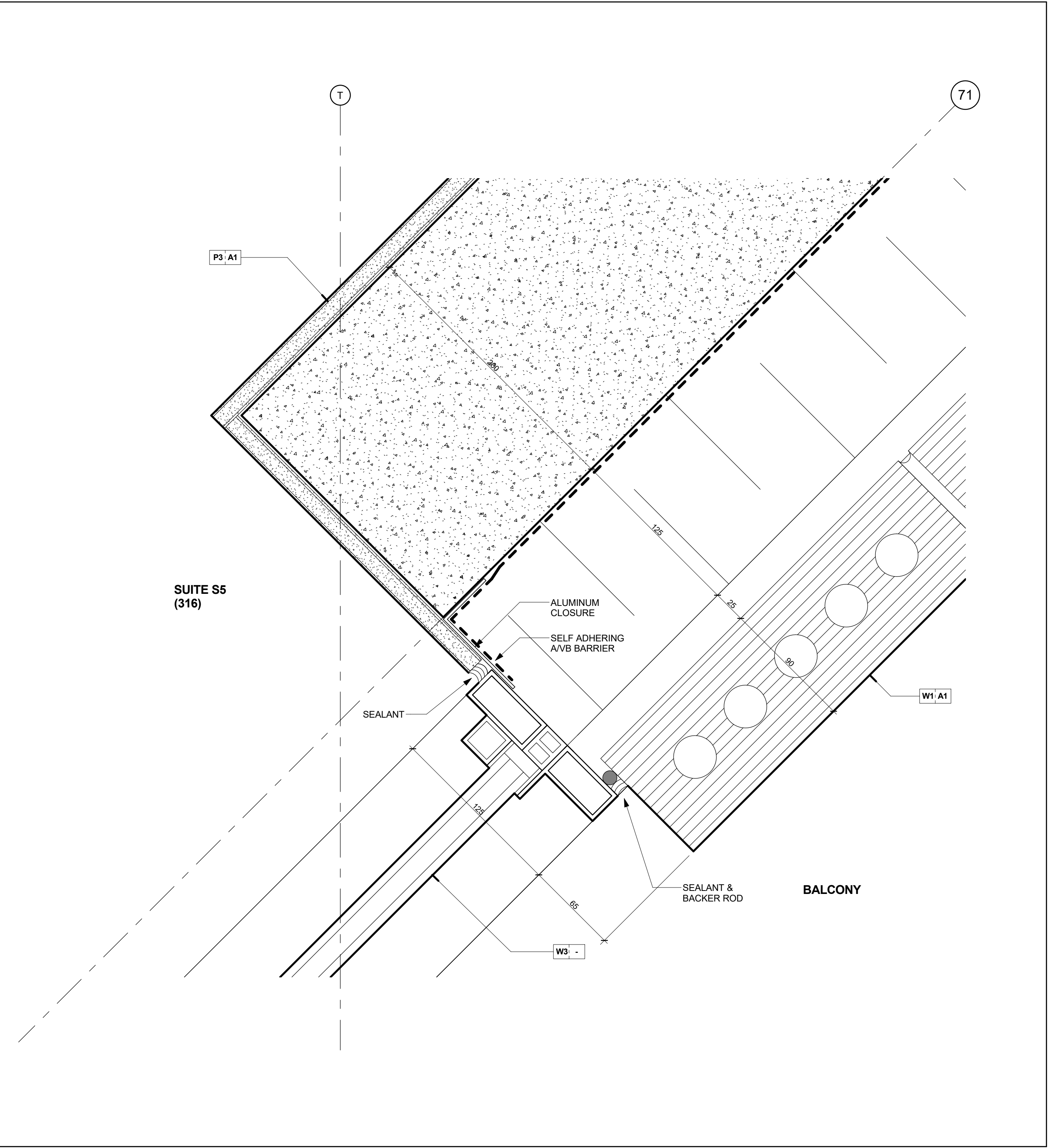
Enlarged Plan Detail @ Window Wall Brick Veneer Wall on Struct. Conc. 2 Scale: 1 : 2 A7-25
