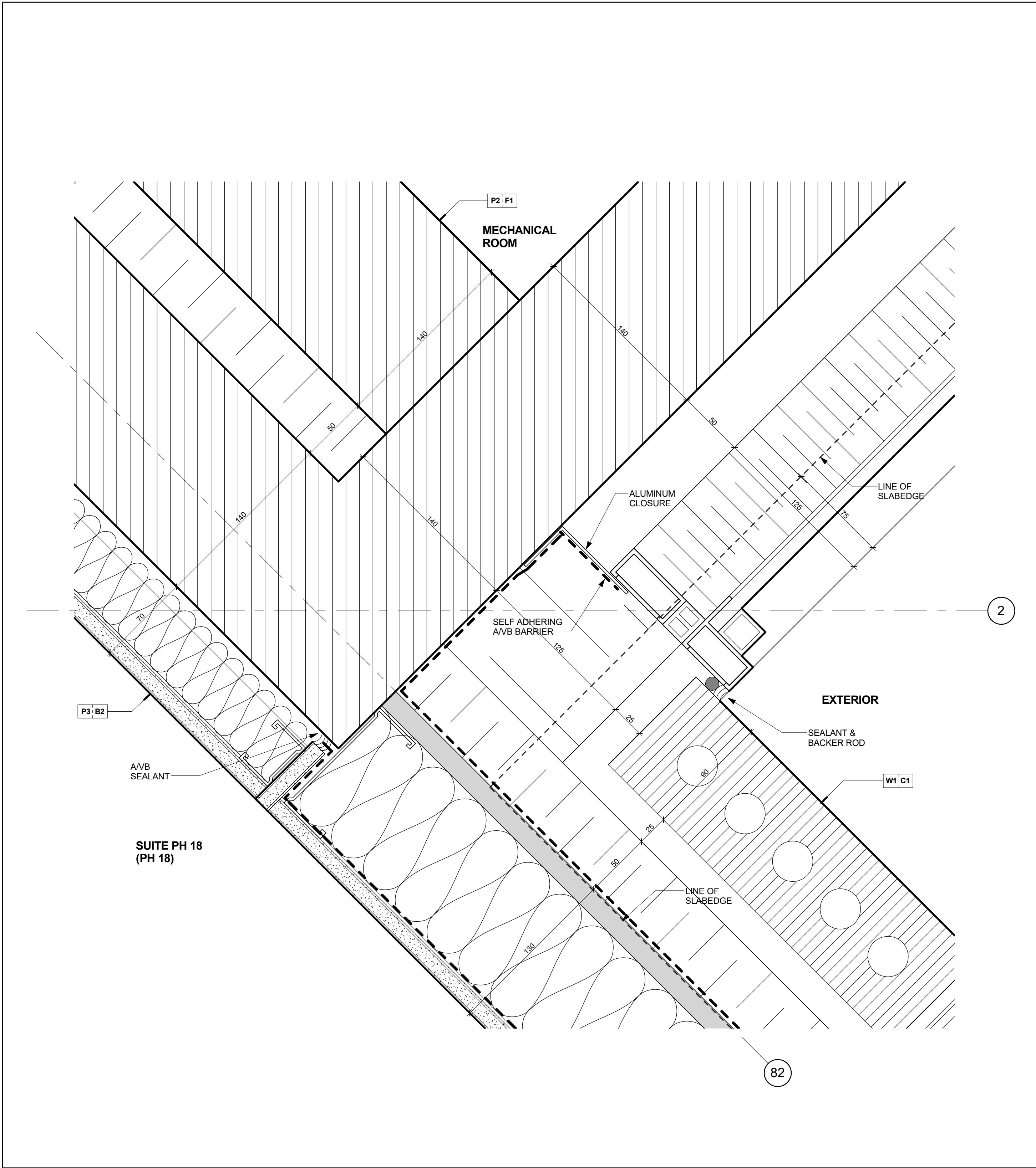
Enlarged Plan Detail @ Window Jamb @ Brick Veneer Wall with Metal Studs 5 Scale: 1 : 2 A7-25
