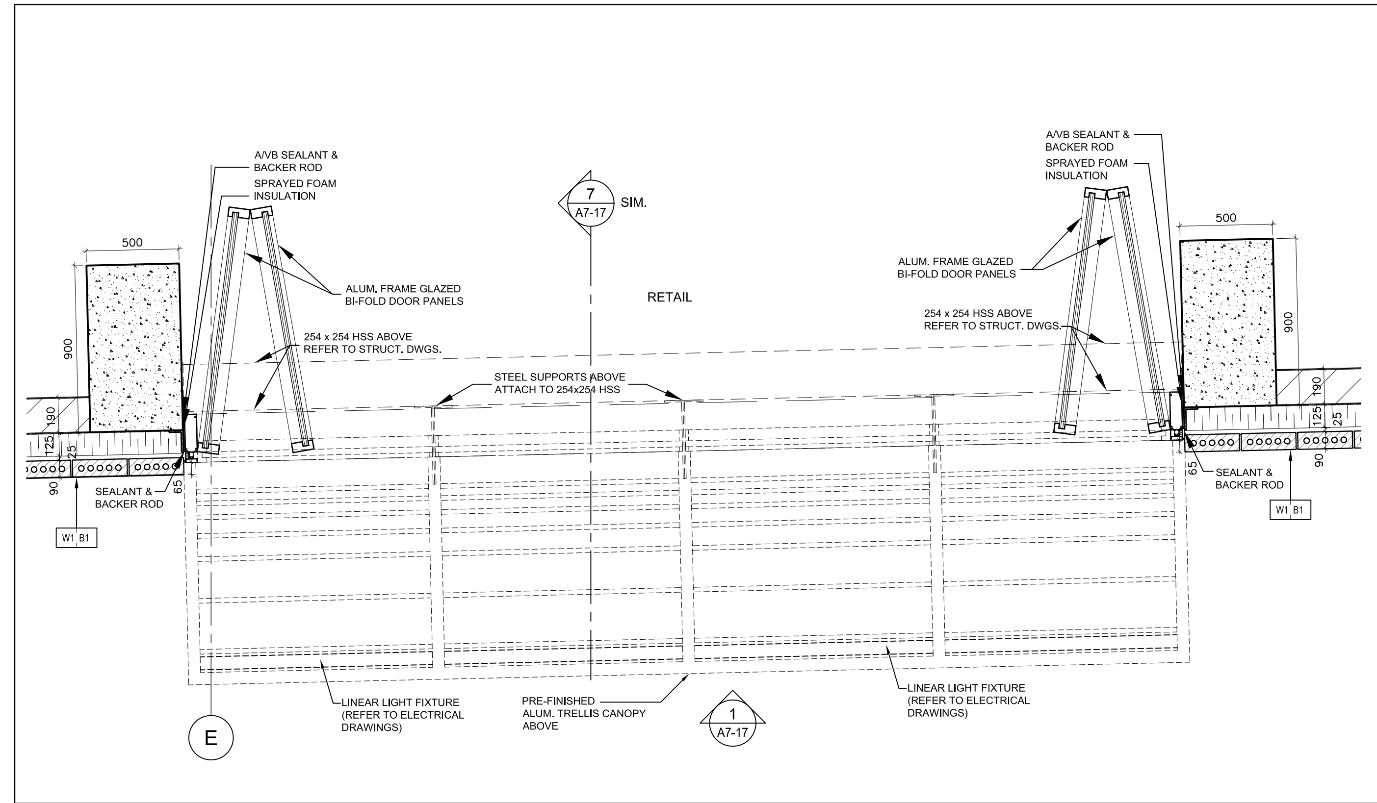
Plan - Bi-Fold Door 1 @ Retail @ Level 1 2 A7-17 SCALE 1:20
