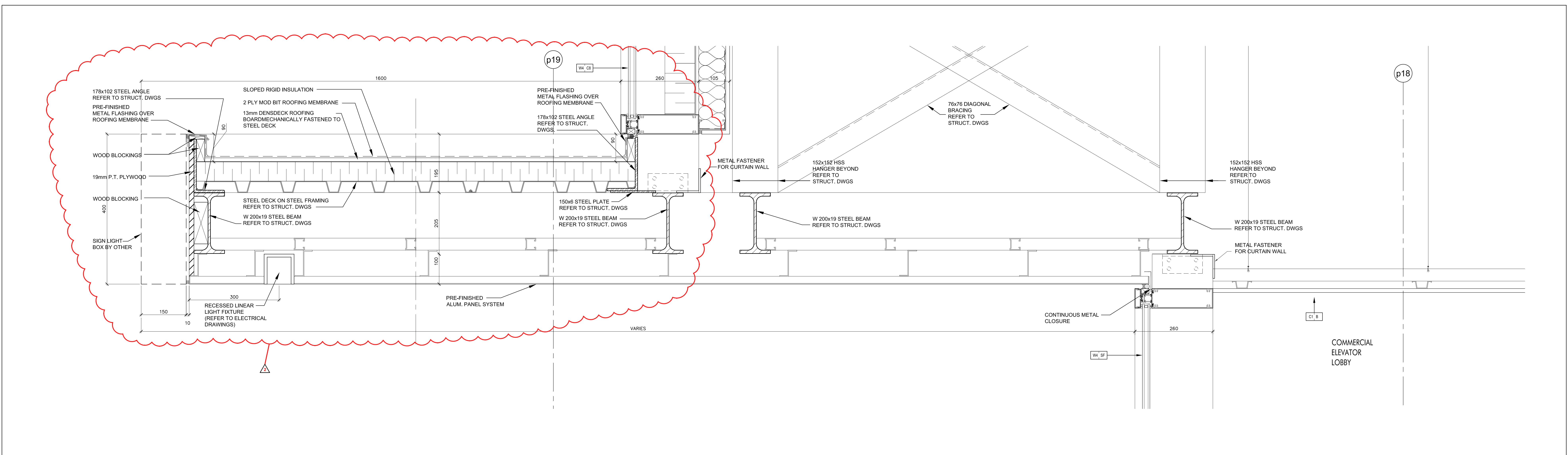
Pre-Finished Aluminum Canopy @ Commercial Elevator Lobby @ Level 1 SCALE 1:5 A7-16
