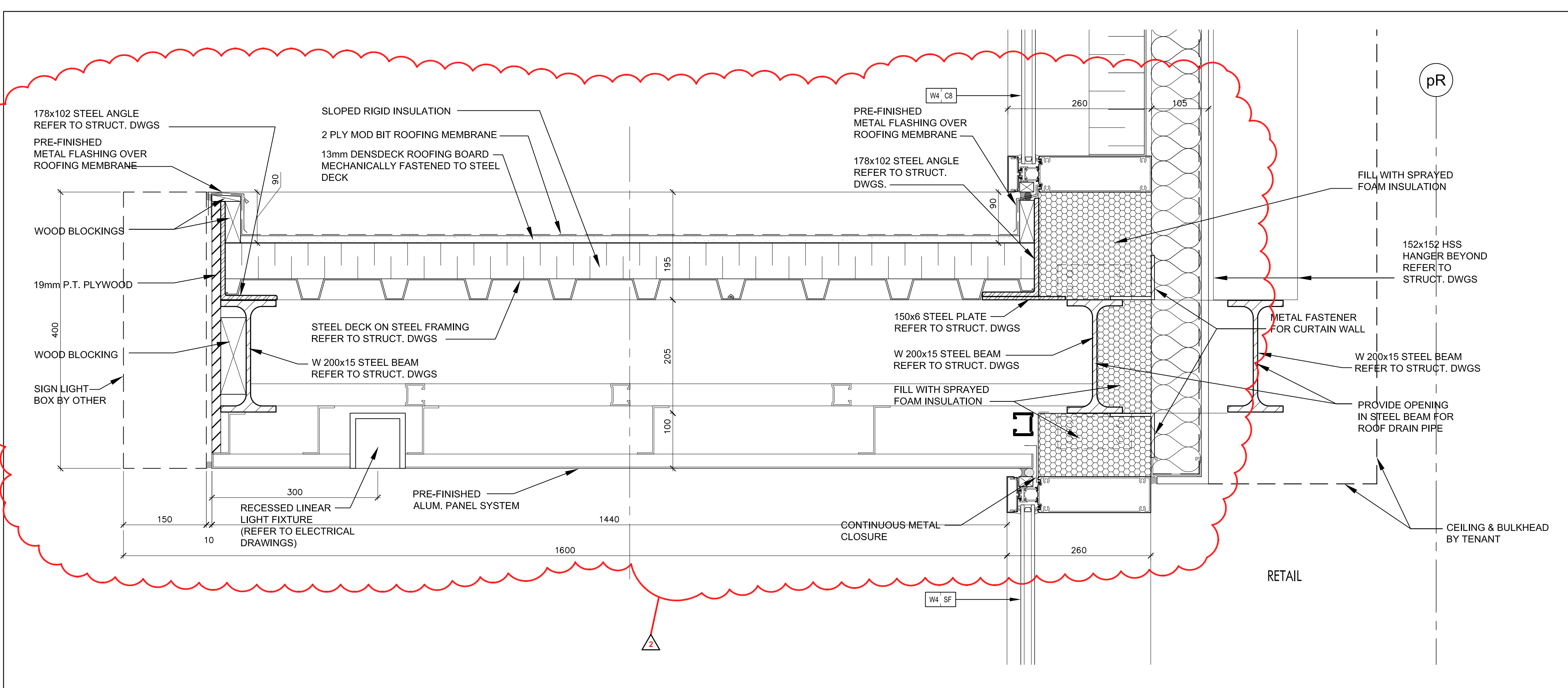
Pre-Finished Aluminum Canopy @ Retail @ Level 1 (Ref. Wall Section 4/A7-04) SCALE 1:5 A7-16
