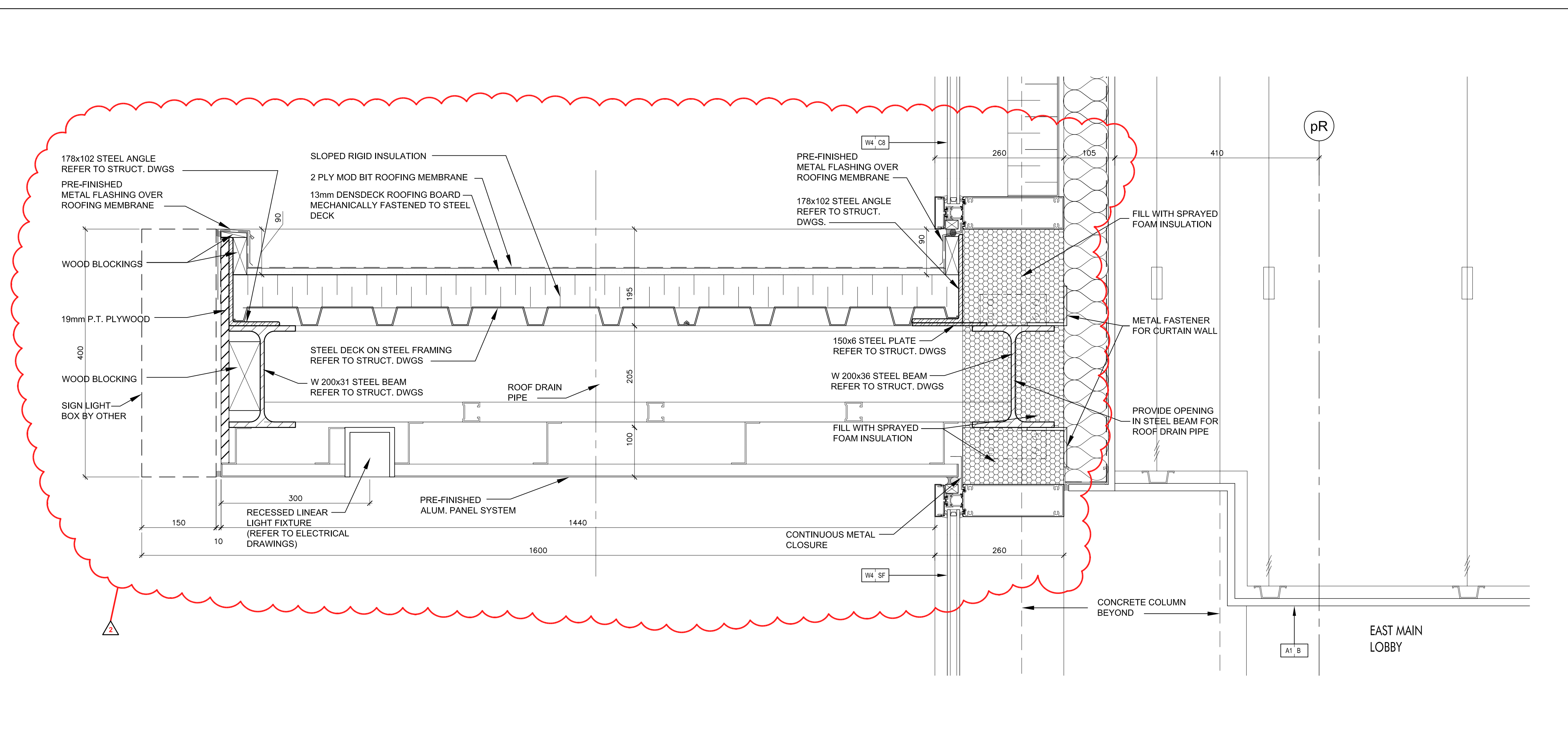
Pre-Finished Aluminum Canopy @ East Main Lobby @ Level 1 (Ref. Wall Section 7/A7-02) SCALE 1:5 A7-16
