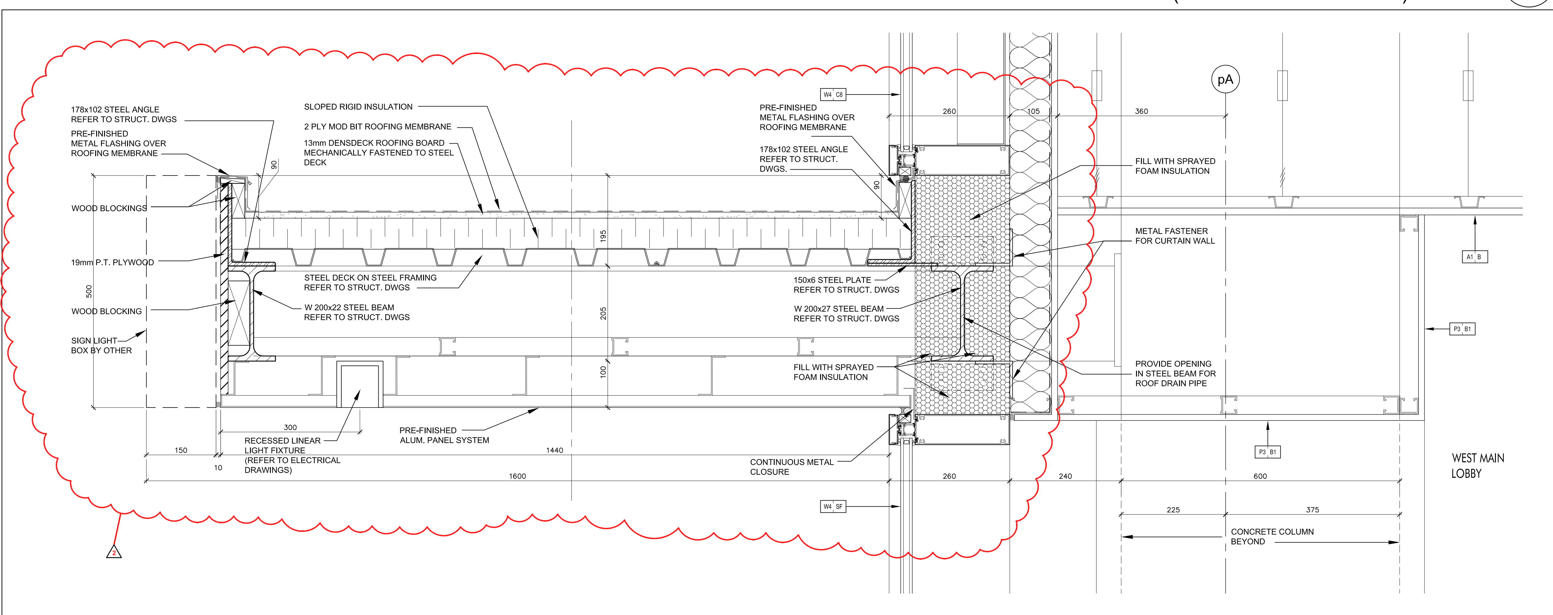
Pre-Finished Aluminum Canopy @ West Main Lobby @ Level 1 (Ref. Wall Section 10/A7-04) SCALE 1:5 A7-16
