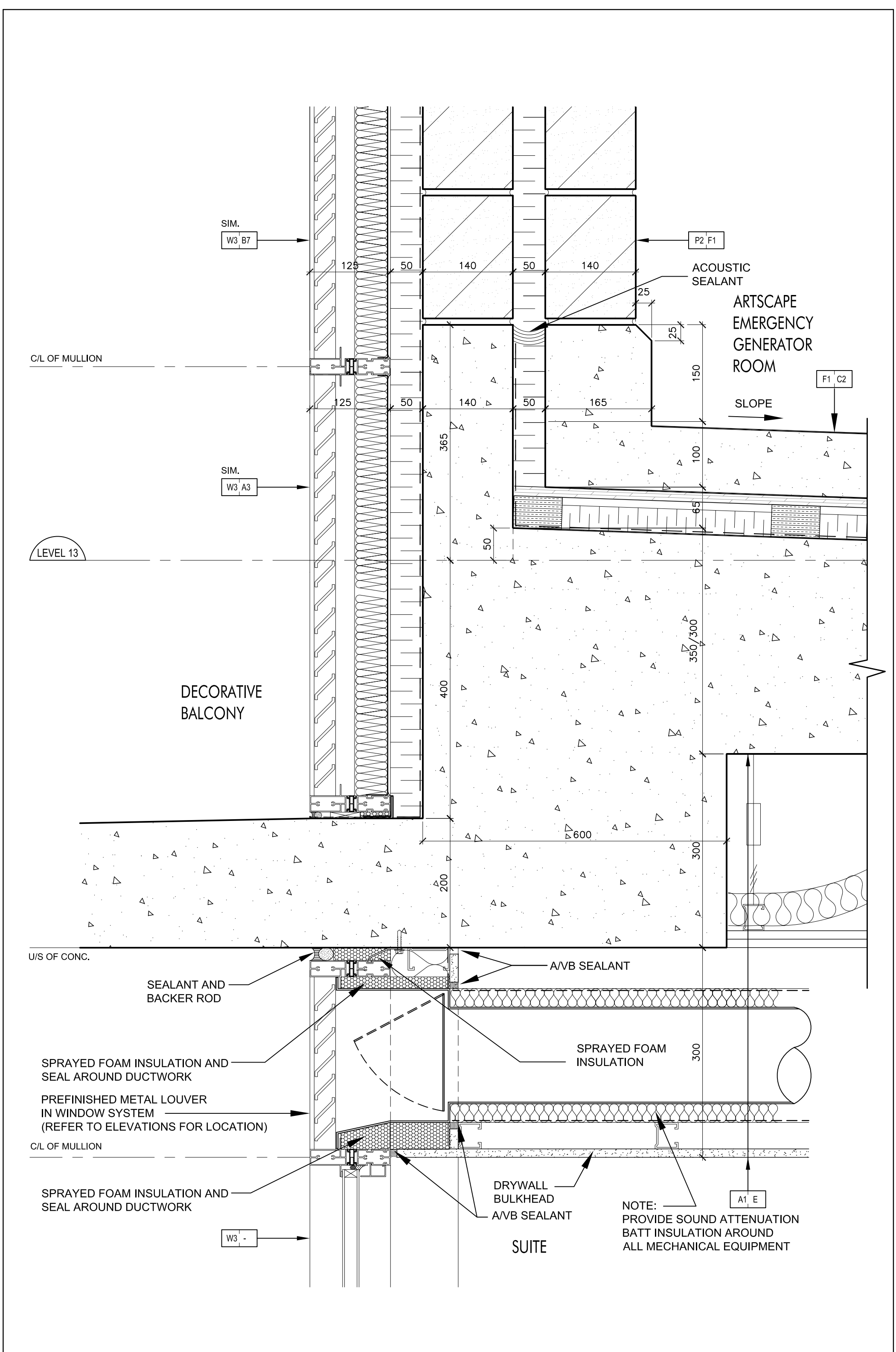
Floating Floor @ Emergency Generator Room @ Level 13 8 (Ref. Wall Section 6/A7-01) SCALE 1:5 A7-14
