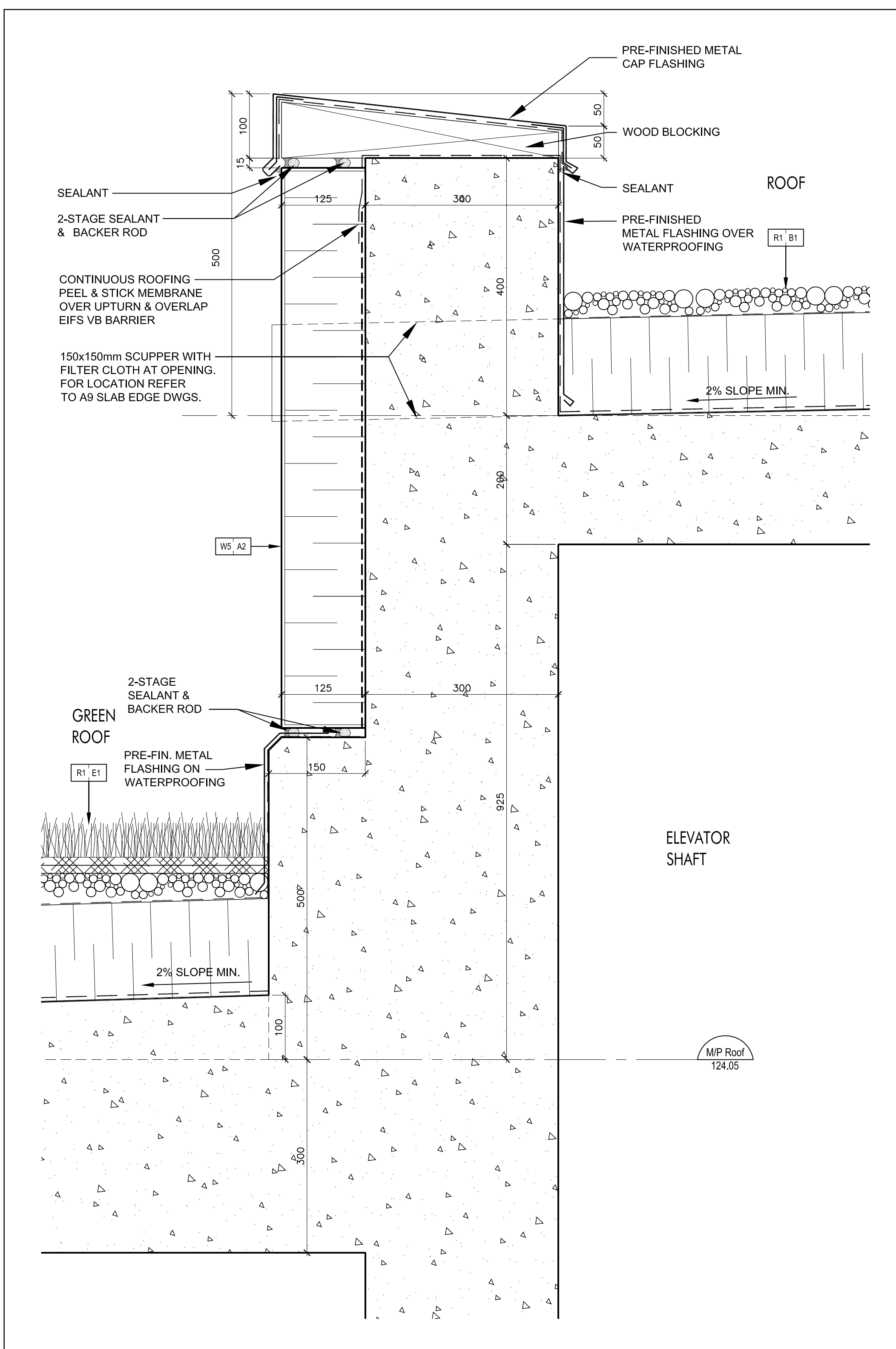
Parapet @ Elevator Shaft Roof 12 SCALE 1:5 A7-14
