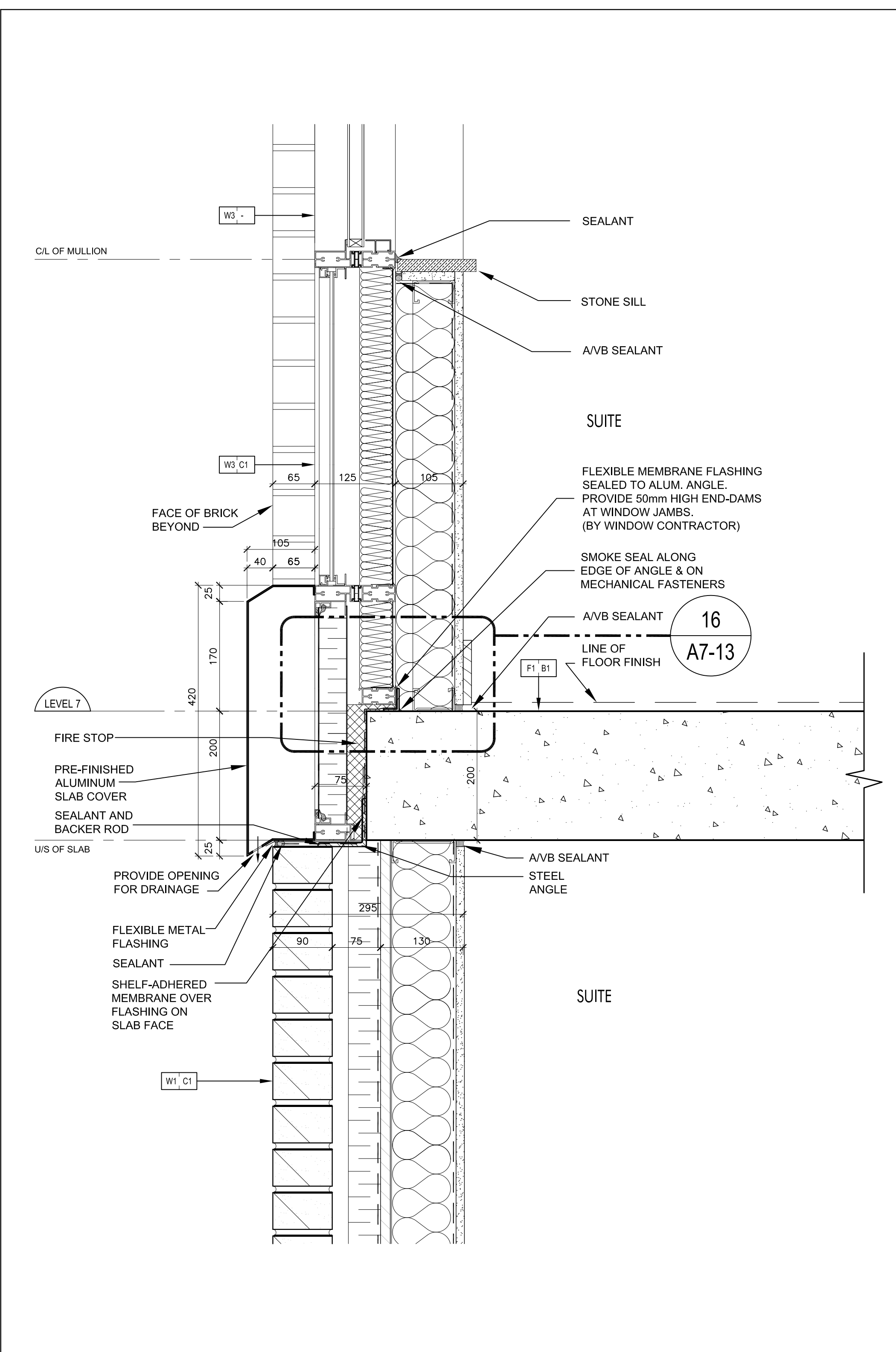
Pre-Finished Aluminum Slab Cover @ Level 7 7 (Ref. Wall Section 5/A7-01) SCALE 1:5 A7-14
