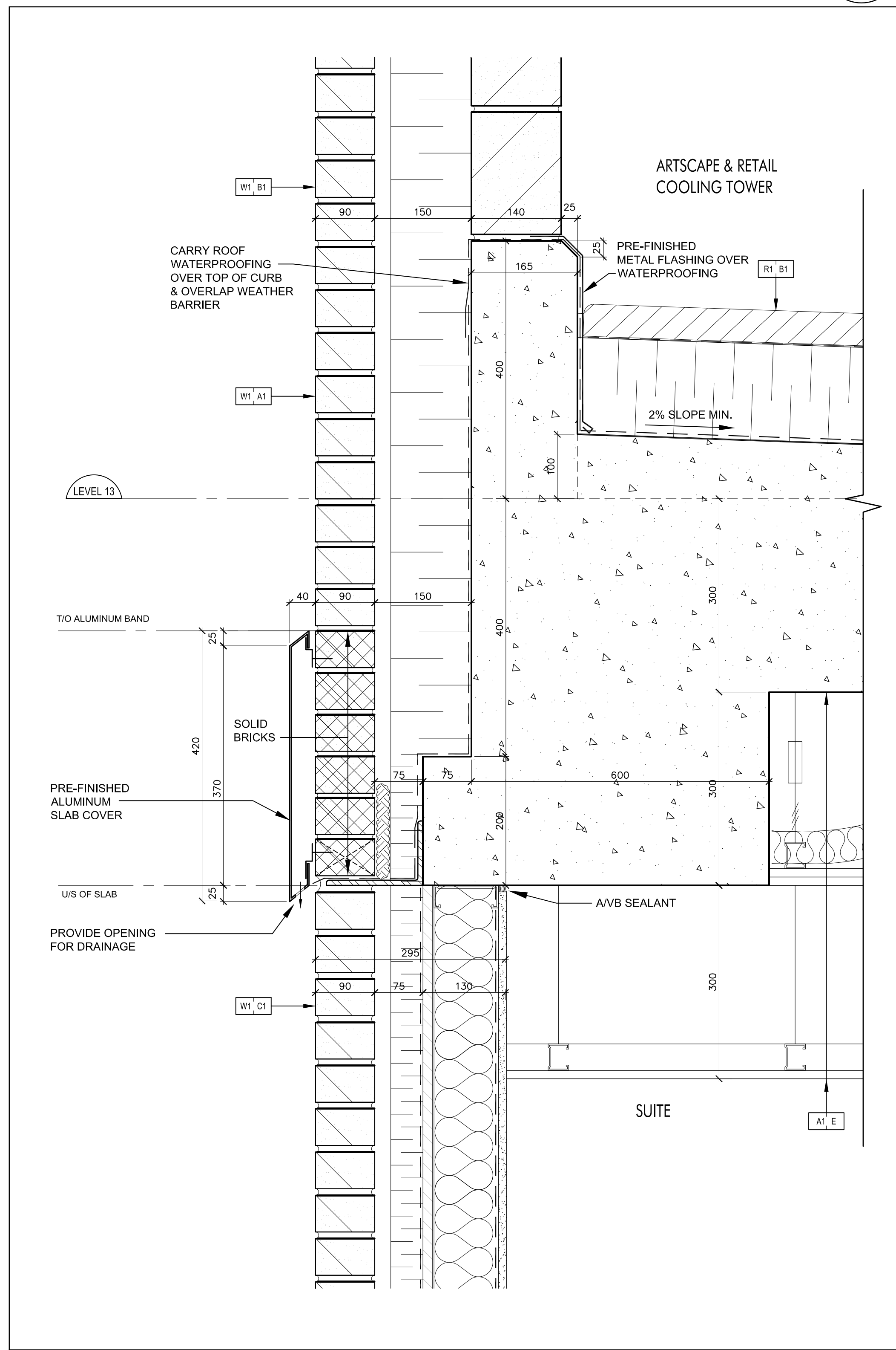
Pre-Finished Aluminum Slab Cover @ Level 13 5 (Ref. Wall Section 5/A7-01) SCALE 1:5 A7-14
