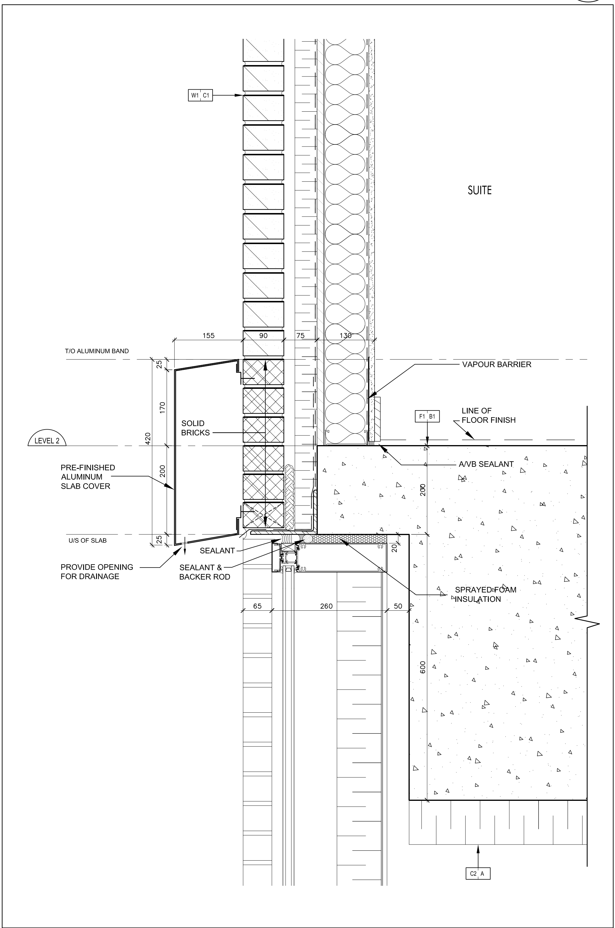
Pre-Fin. Alum. Slab Cover @ Brick Wall & Curtain Wall-Level 2 2 (Ref. Wall Section 5/A7-01) SCALE 1:5 A7-14
