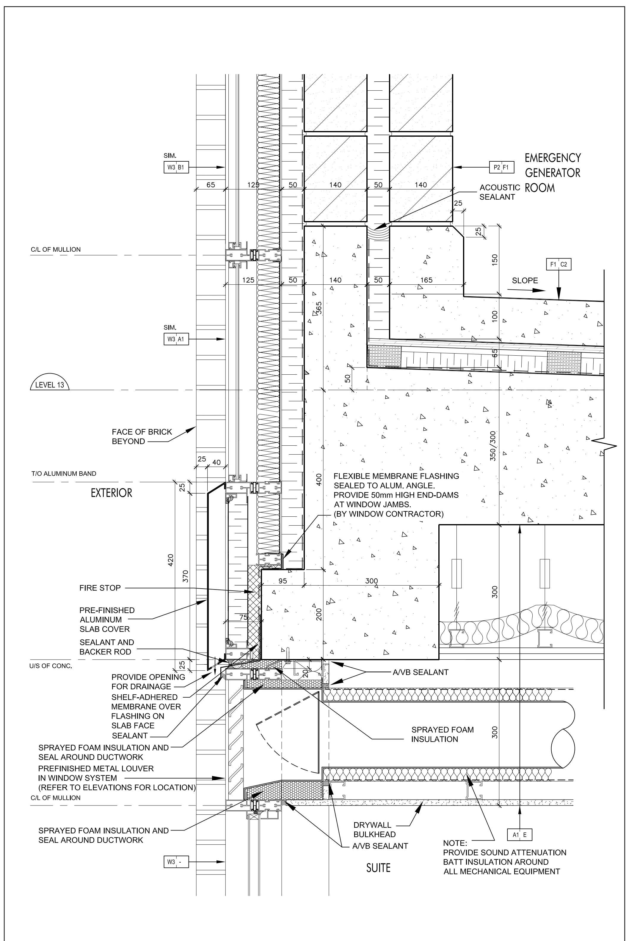
Floating Floor @ Emergency Generator Room @ Level 13 9 (Ref. Wall Section 7/A7-02) SCALE 1:5 A7-14
