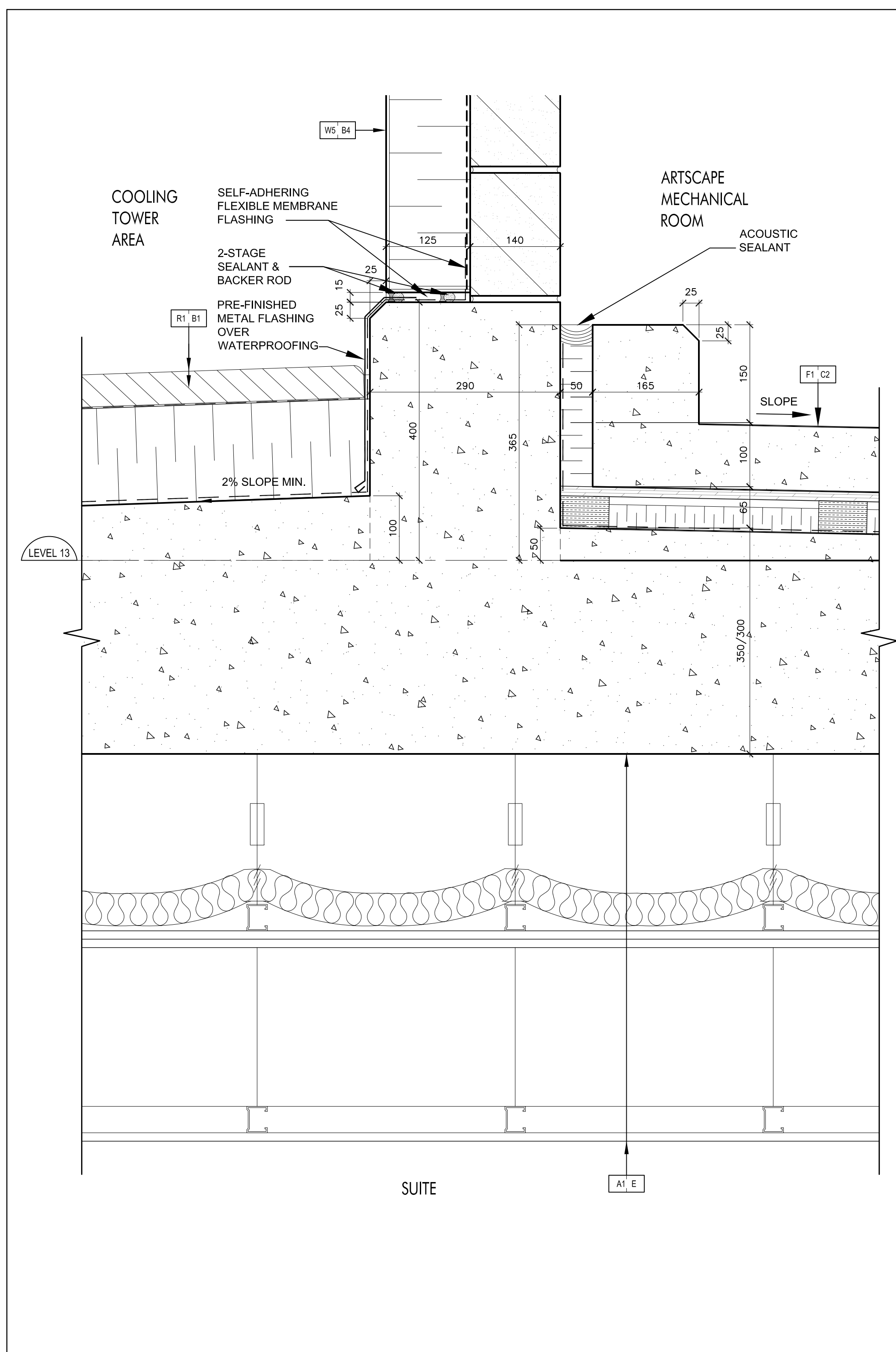
Conc. Curb @ Mechanical Room Floating Slab @ Level 13 10 (Ref. Wall Section 4/A7-01) SCALE 1:5 A7-14
