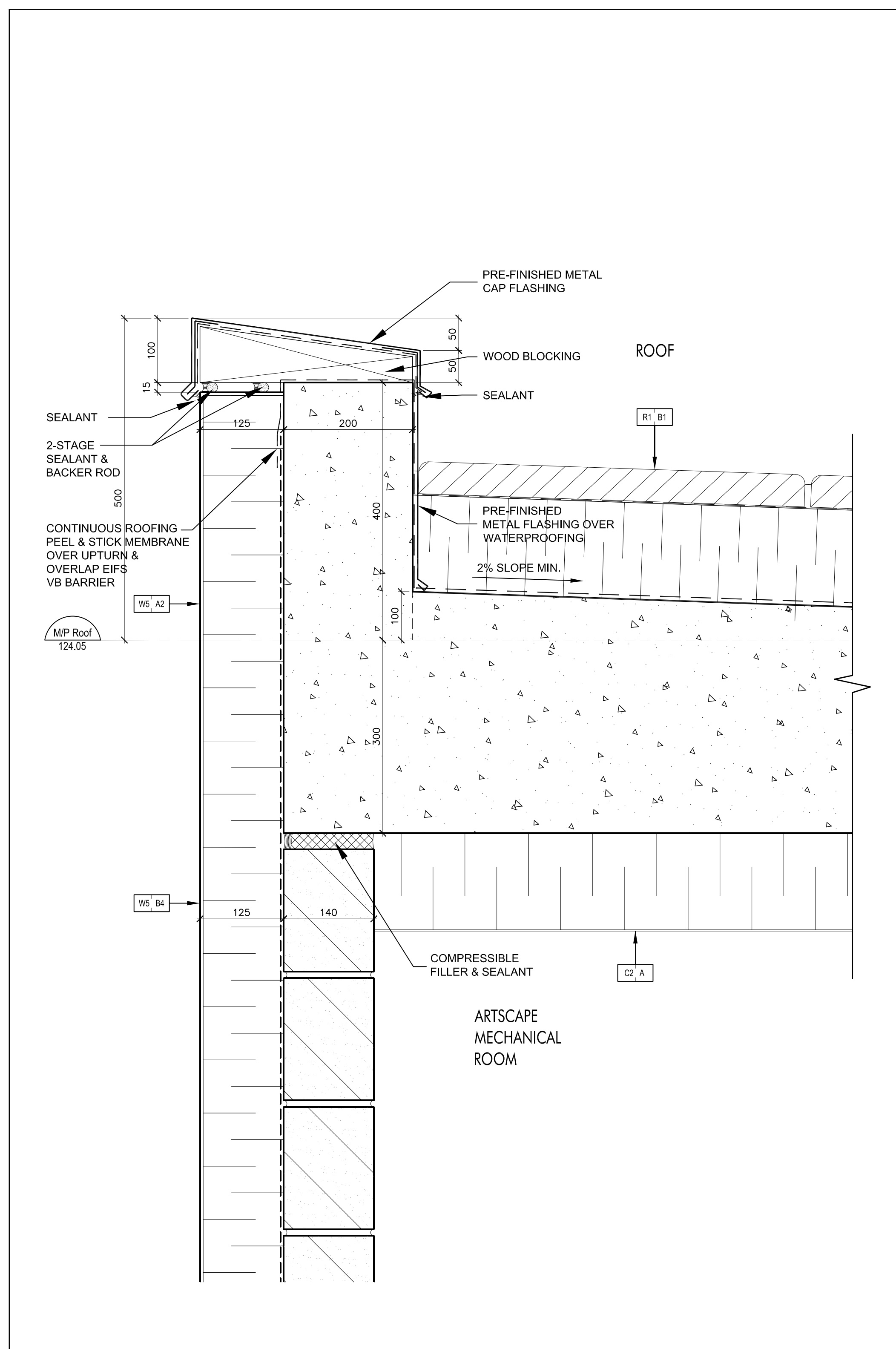
Parapet @ Mechanical Penthouse Roof 11 (Ref. Wall Section 4/A7-01) SCALE 1:5 A7-14
