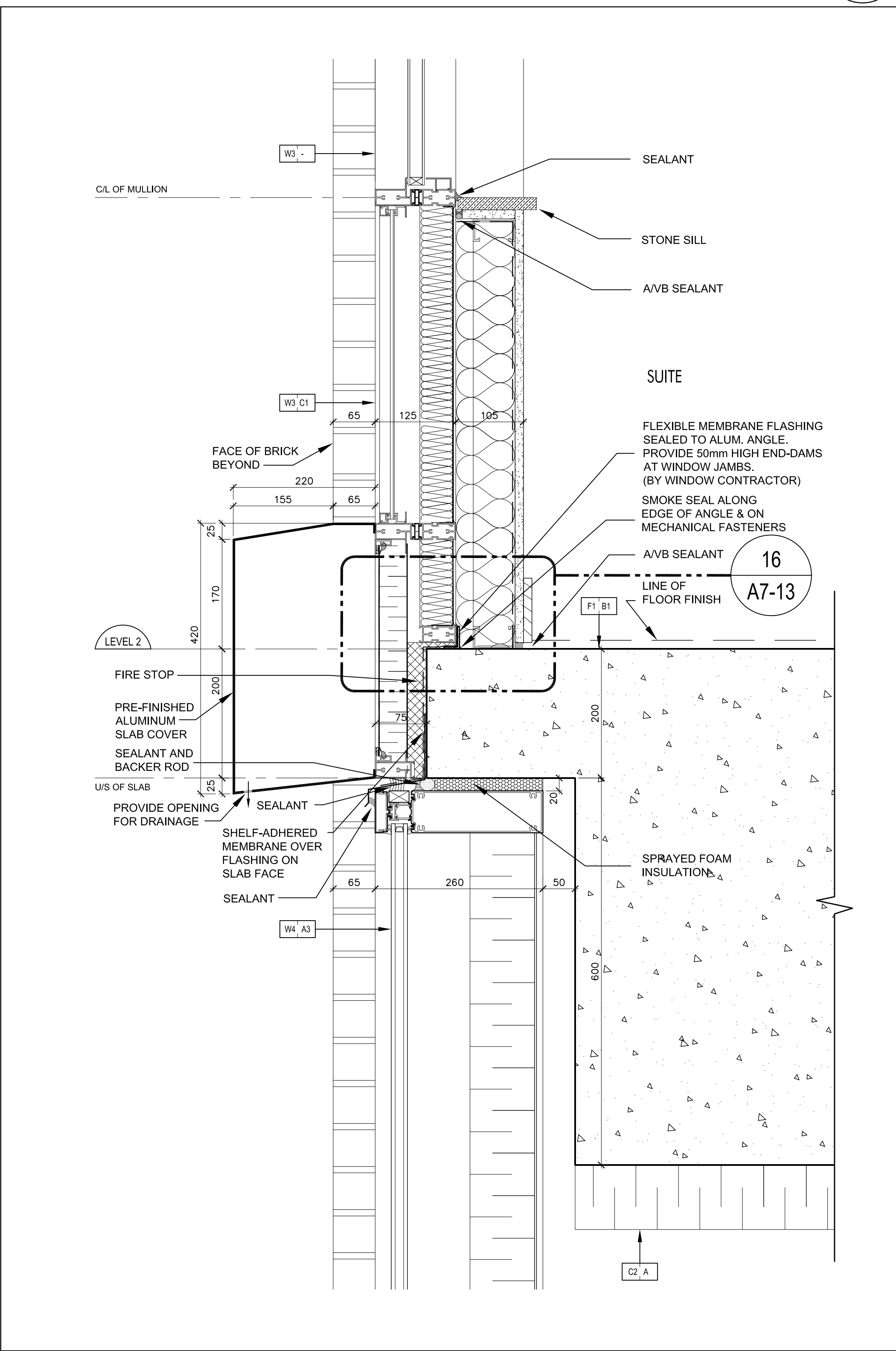
Pre-Fin. Alum. Slab Cover @ Window Wall & Curtain Wall-Level 2 1 (Ref. Wall Section 4/A7-01) SCALE 1:5 A7-14
