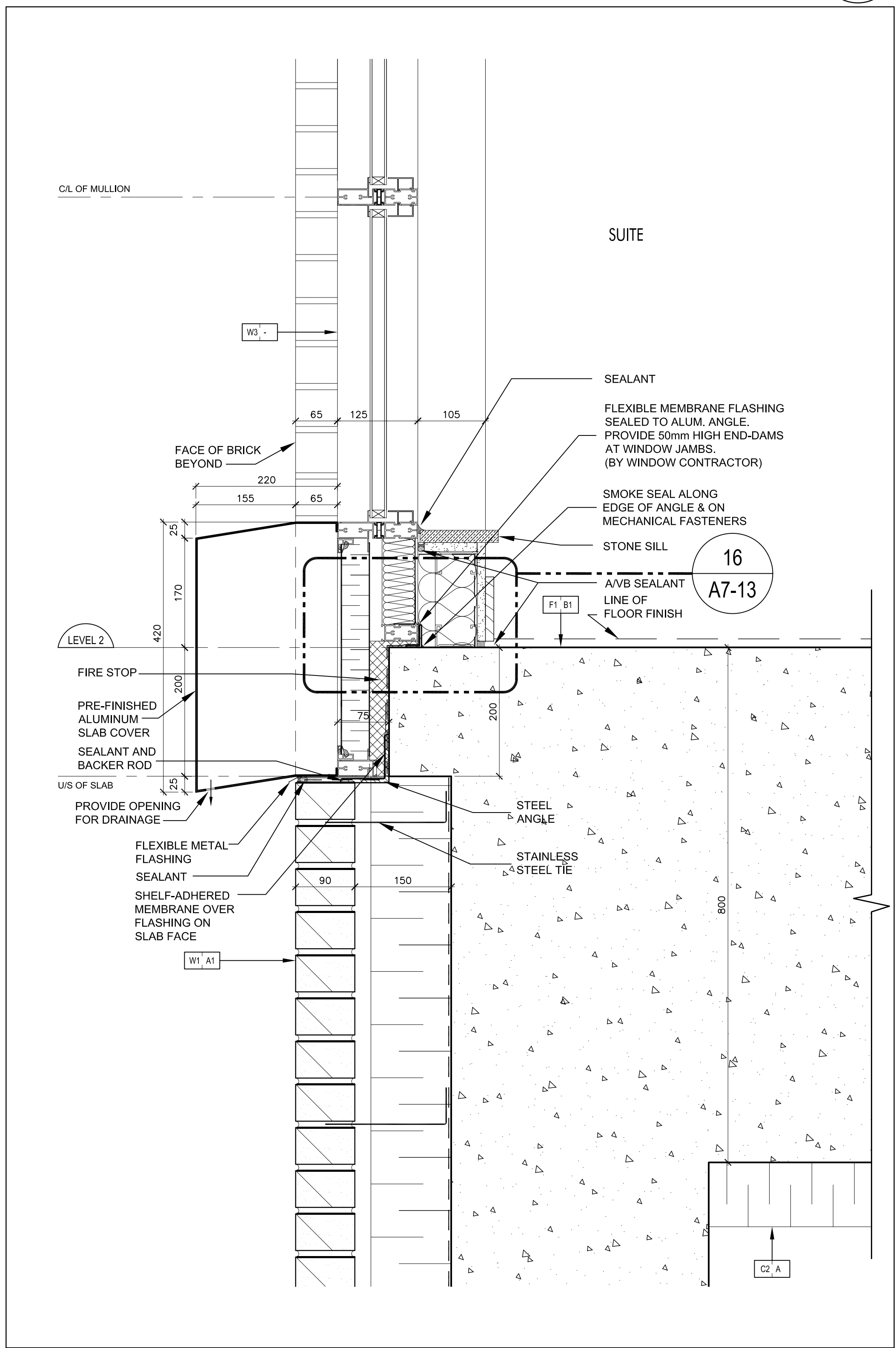
Pre-Fin. Alum. Slab Cover @ Window Wall & Brick Wall-Level 2 3 (Ref. Wall Section 4/A7-09) SCALE 1:5 A7-14
