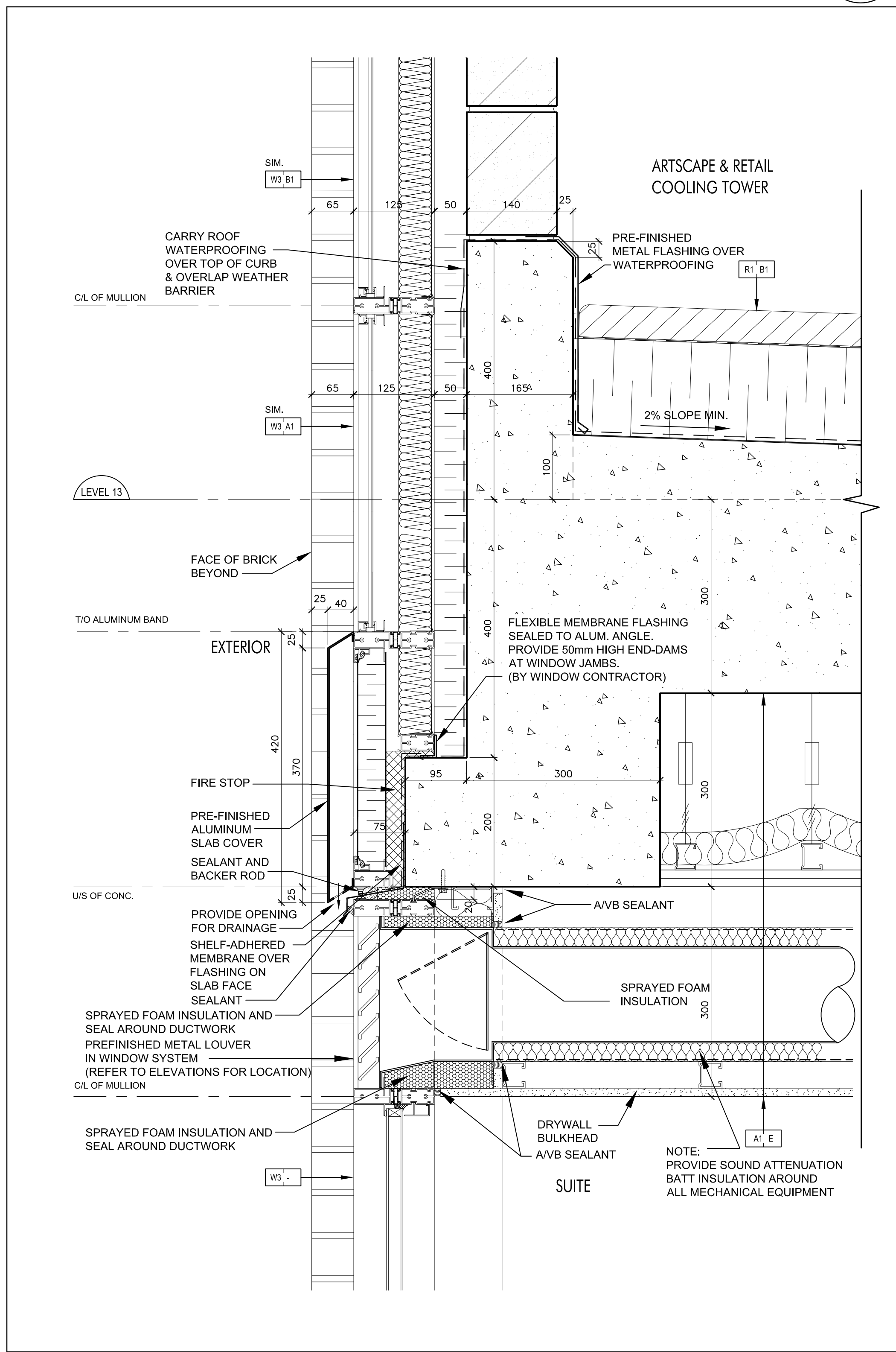
Window Wall Bypass & Pre-Fin. Alum. Slab Cover @ Level 13 4 (Ref. Wall Section 4/A7-01) SCALE 1:5 A7-14
