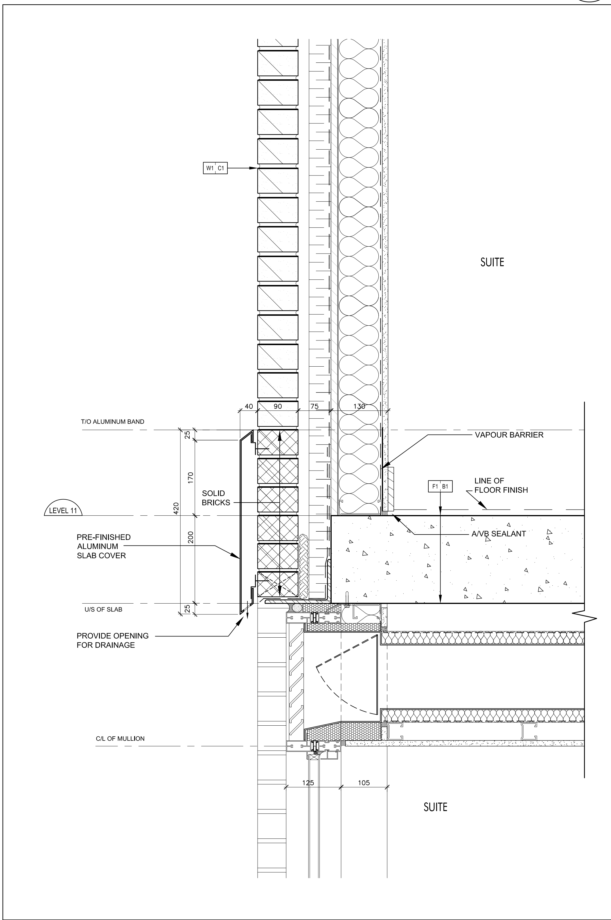
Pre-Finished Aluminum Slab Cover @ Level 11 6 (Ref. Wall Section 5/A7-01) SCALE 1:5 A7-14
