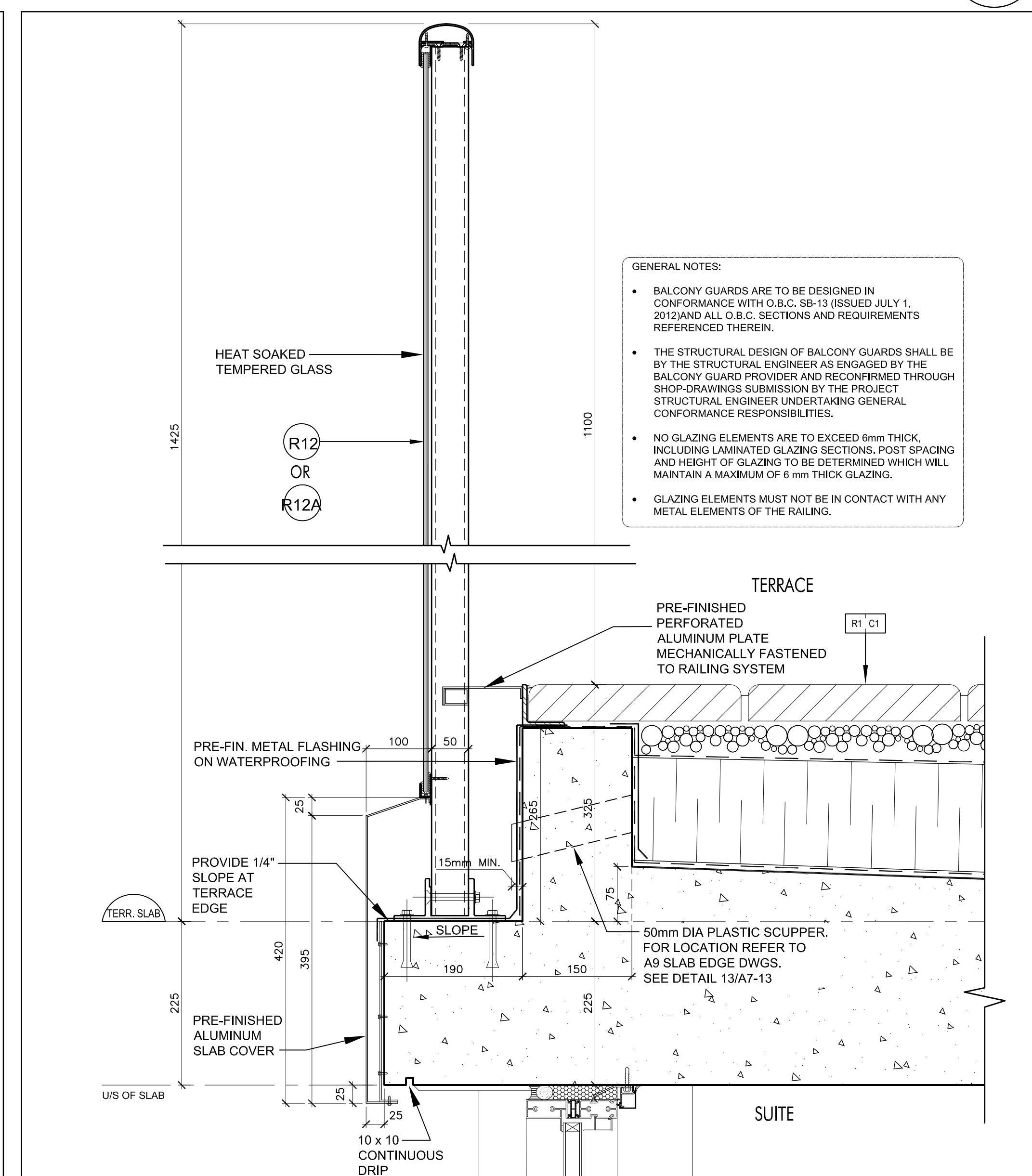
Railing R12 / R12A @ Terrace @ Level 7 +11
