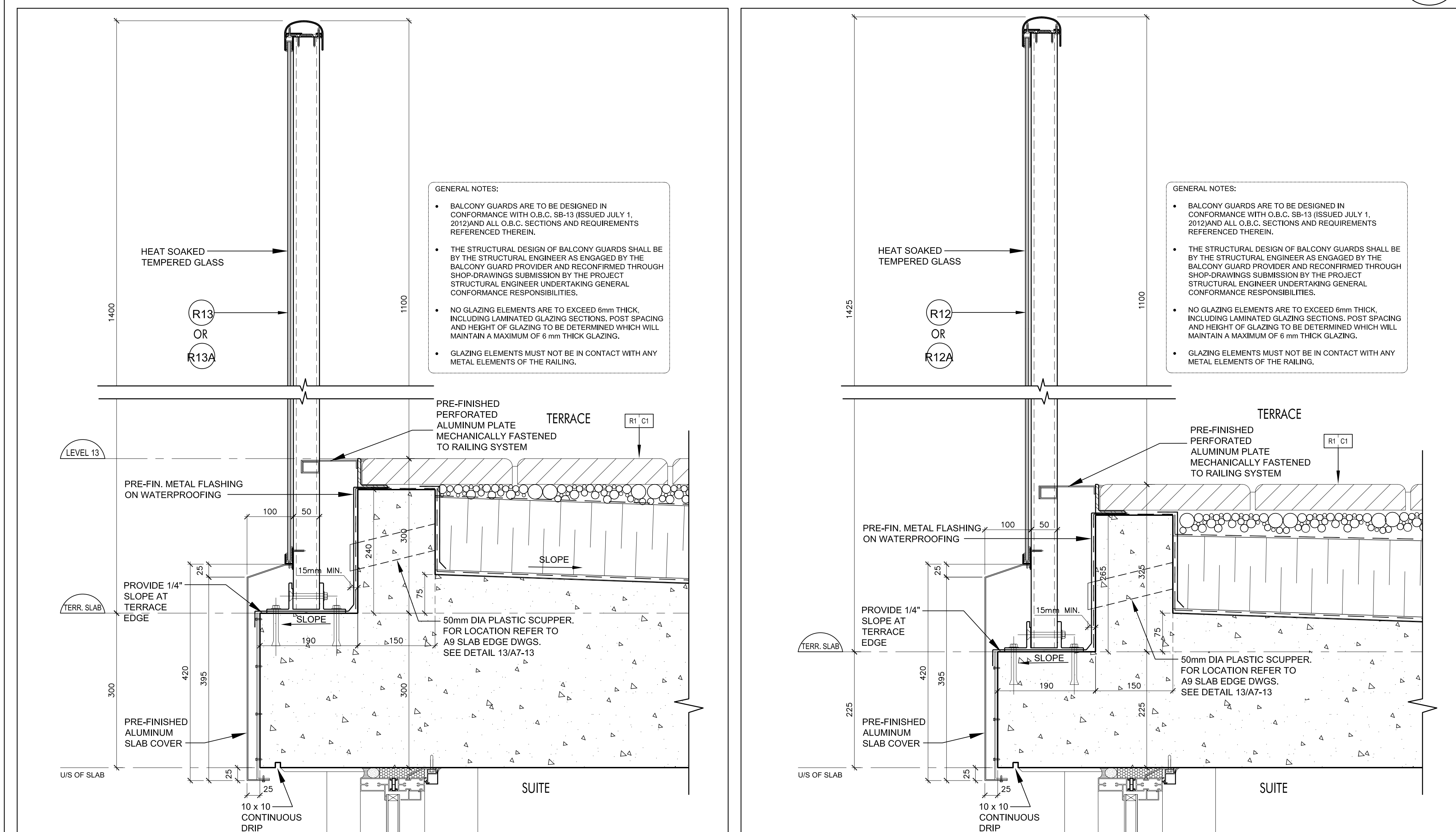
Railing 13 / 13A @ Terrace @ Level 13
