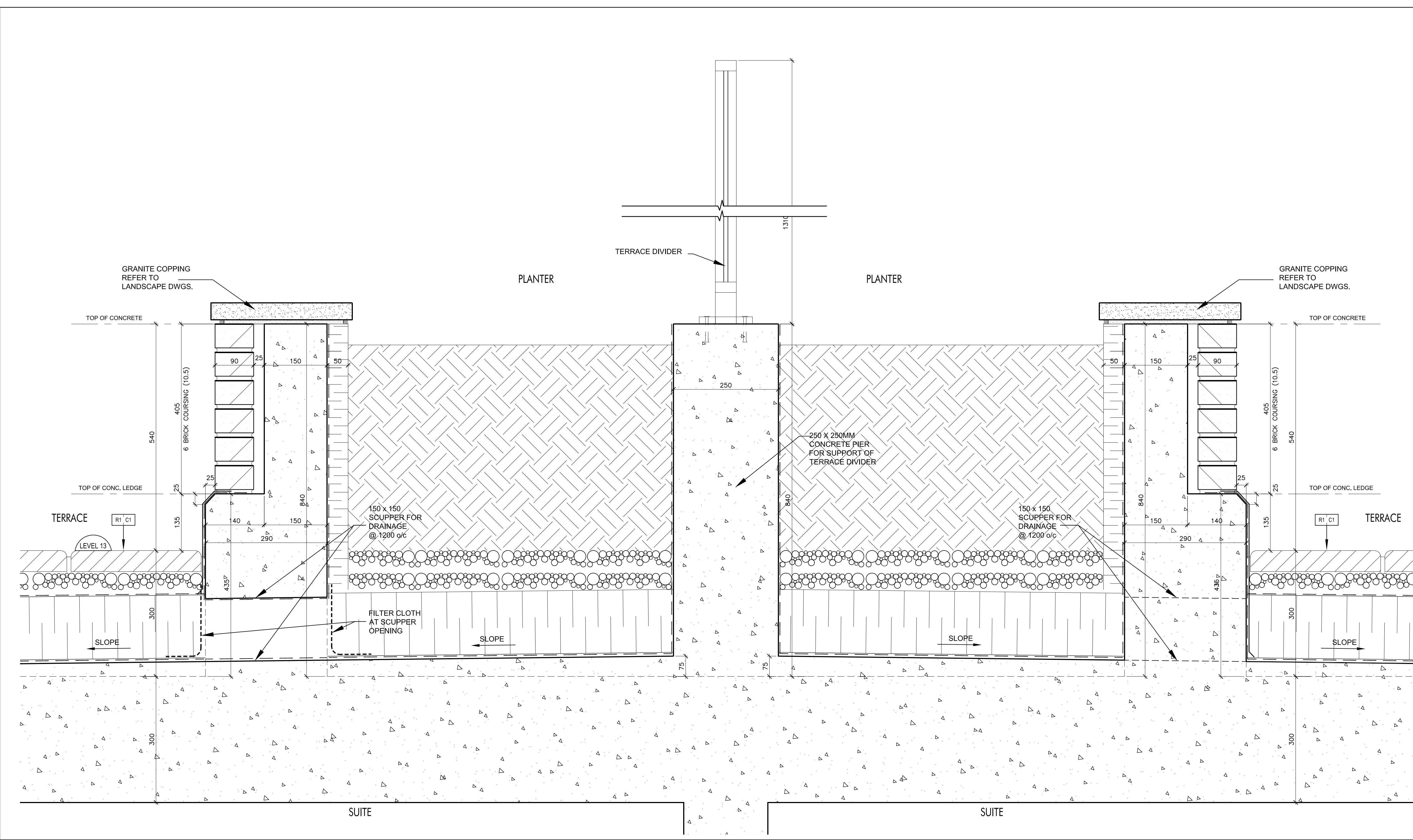
Section Thru Planter @ Terrace @ Level 13
