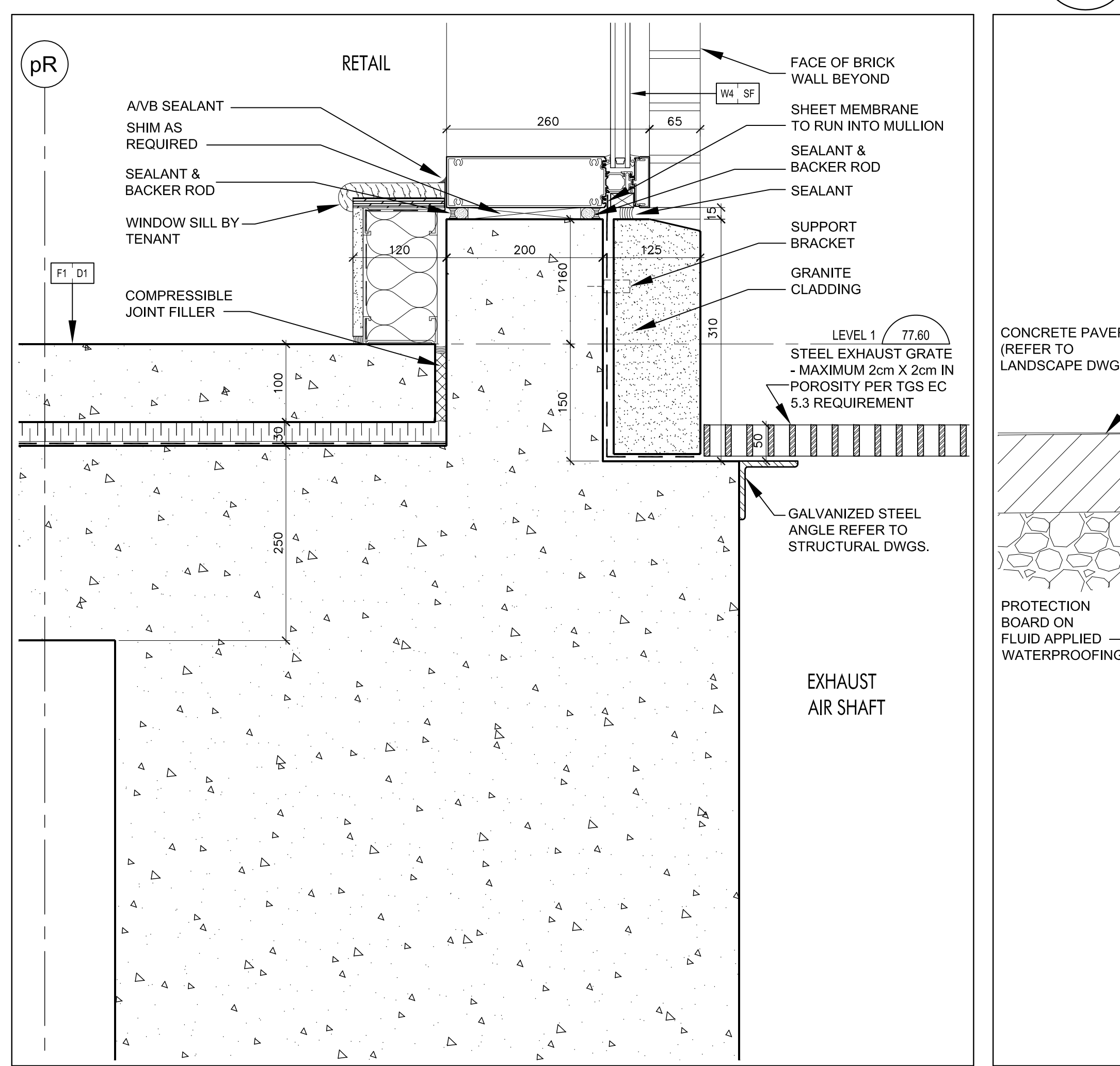
Curtain Wall Sill @ Retail & Steel Grade 4 SCALE 1:5 A7-08
