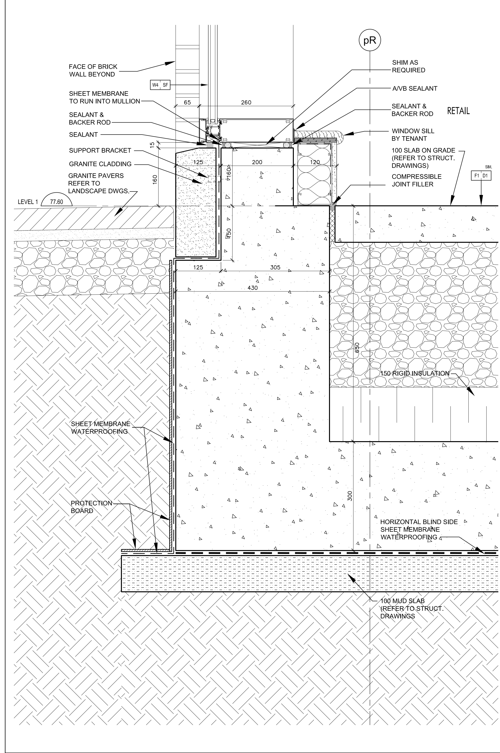
Curtain Wall Sill @ Retail 7 SCALE 1:5 A7-04
