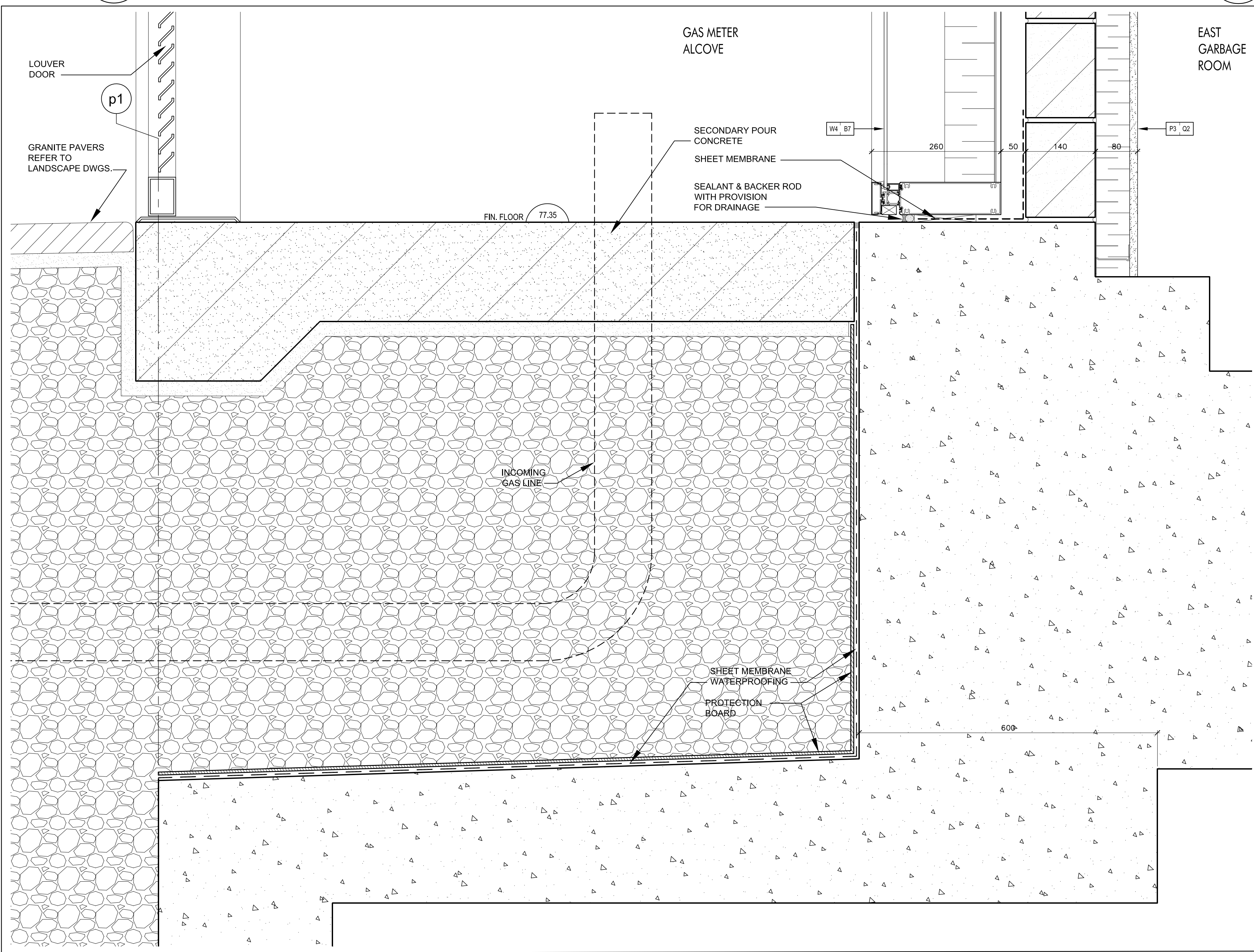
Curtain Wall Sill @ Gas Meter Alcove 9 SCALE 1:5 A7-02
