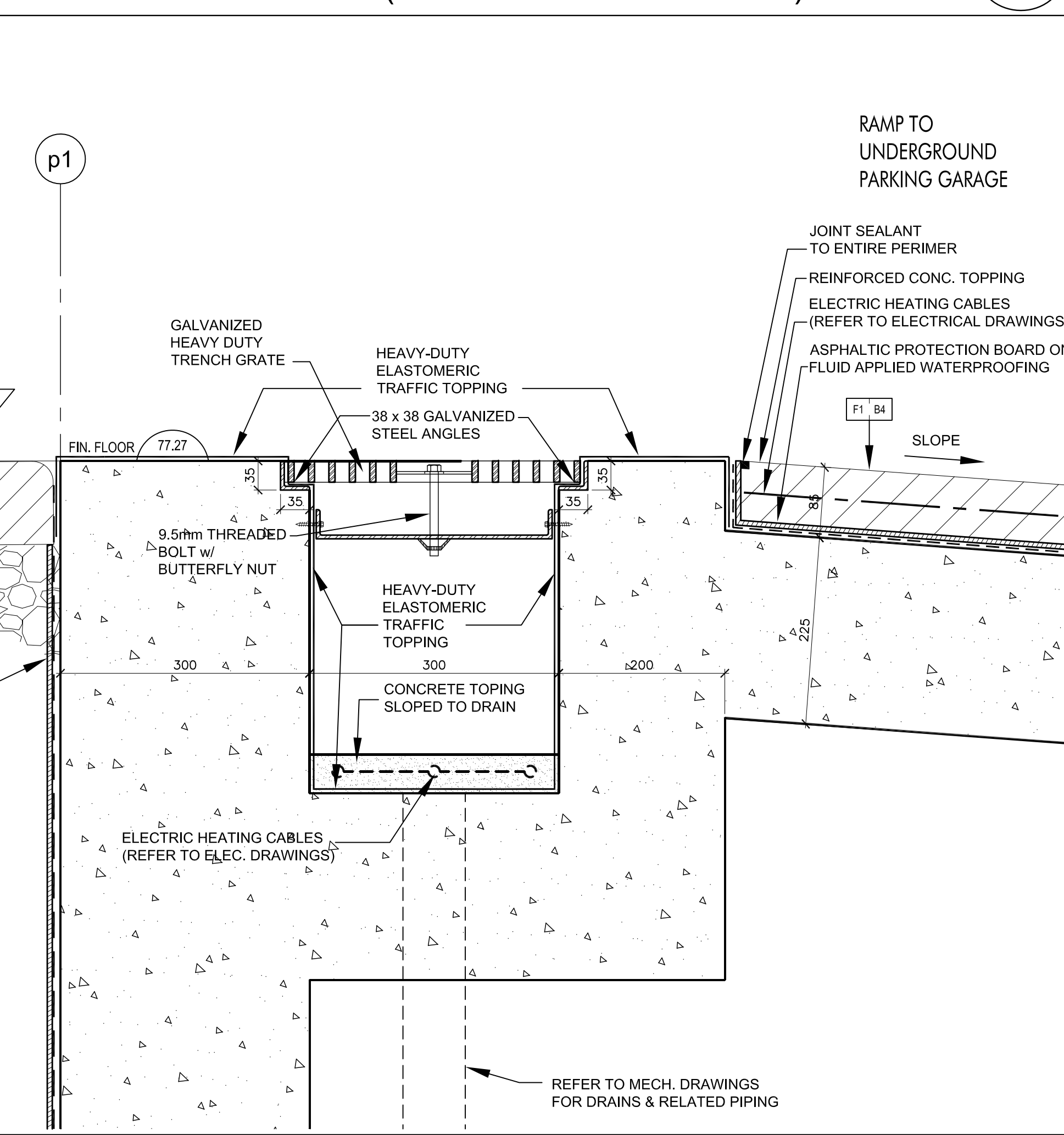
Entrance to Residential Parking 1 SCALE 1:5 A7-08
