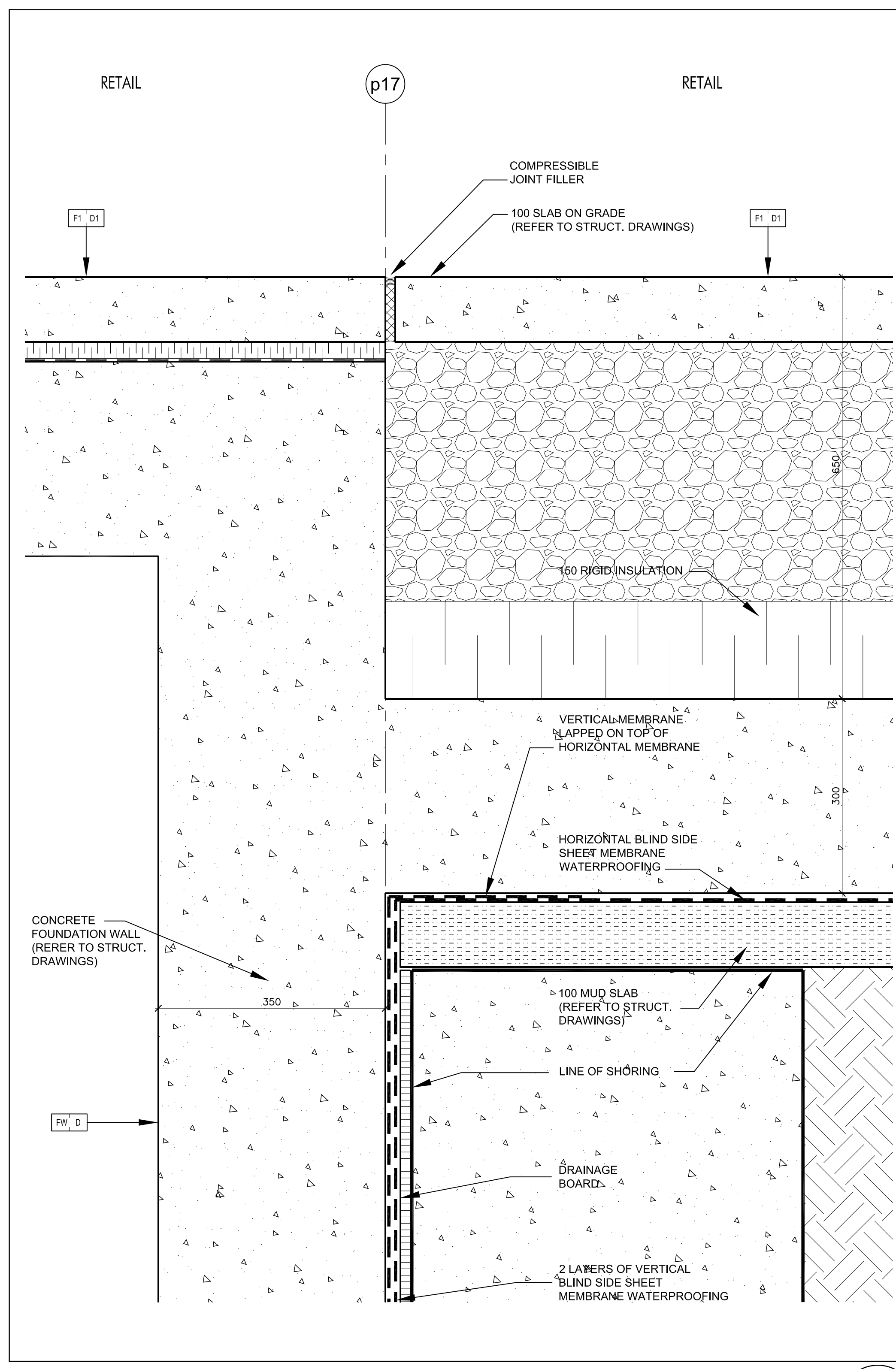
Foundation Wall @ Caisson Wall 8 SCALE 1:5 A7-08
