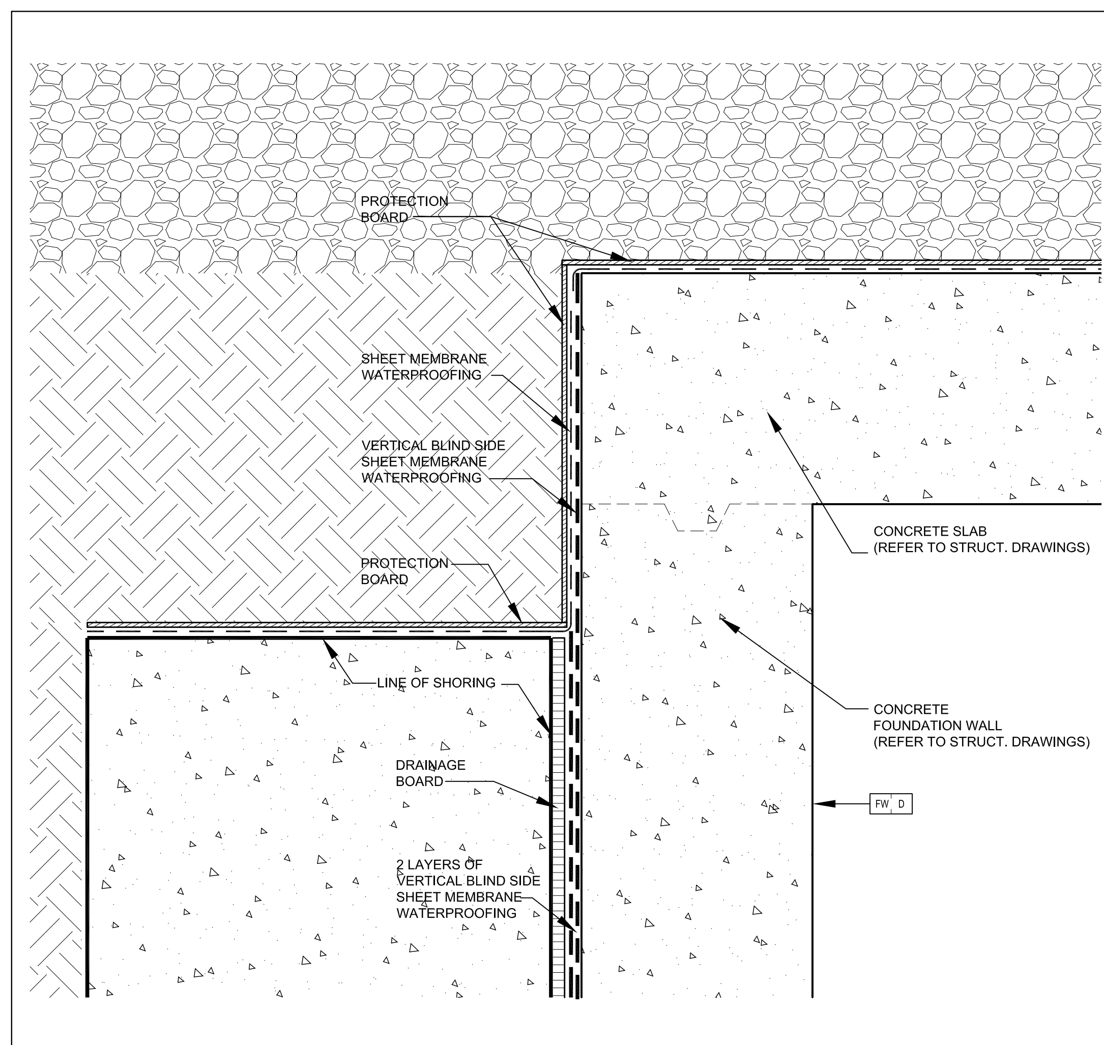
Foundation Wall @ Caisson Wall 6 SCALE 1:5 A7-08
