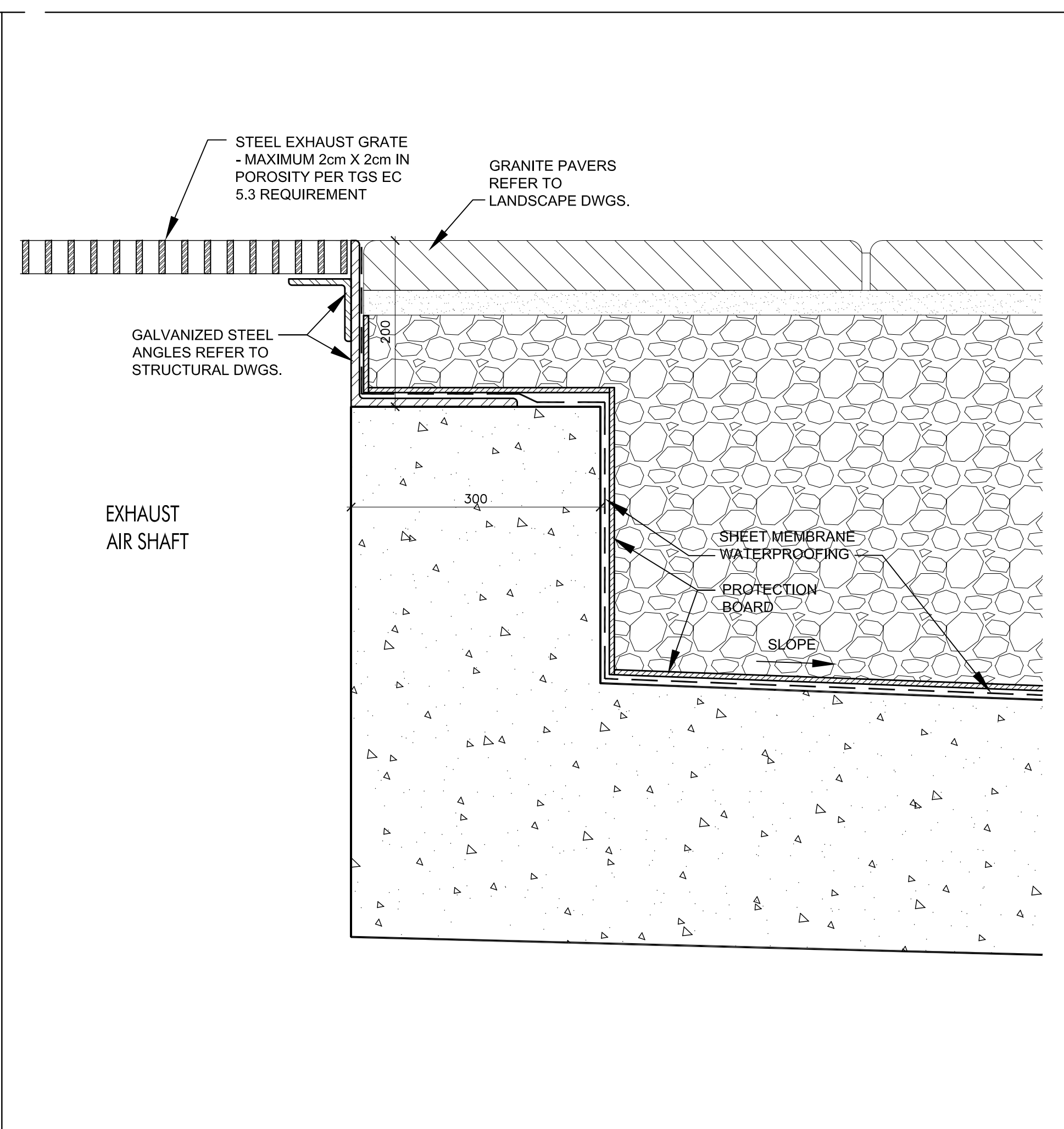
Section thru Exhaust Air Shaft Steel Grate @ Level 1 3 SCALE 1:5 A7-08
