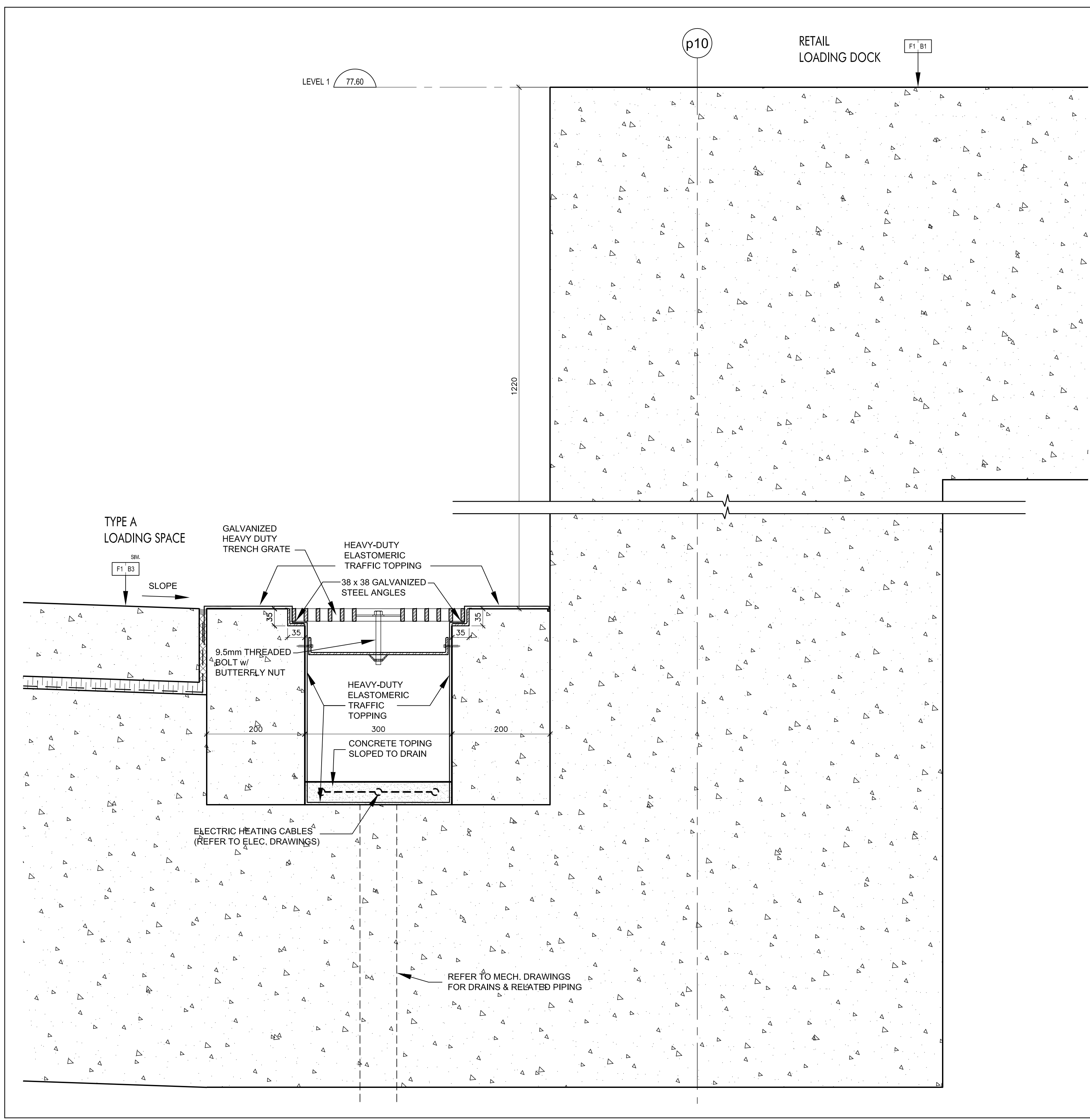
Trench Detail @ Loading Space 10 SCALE 1:5 A7-08
