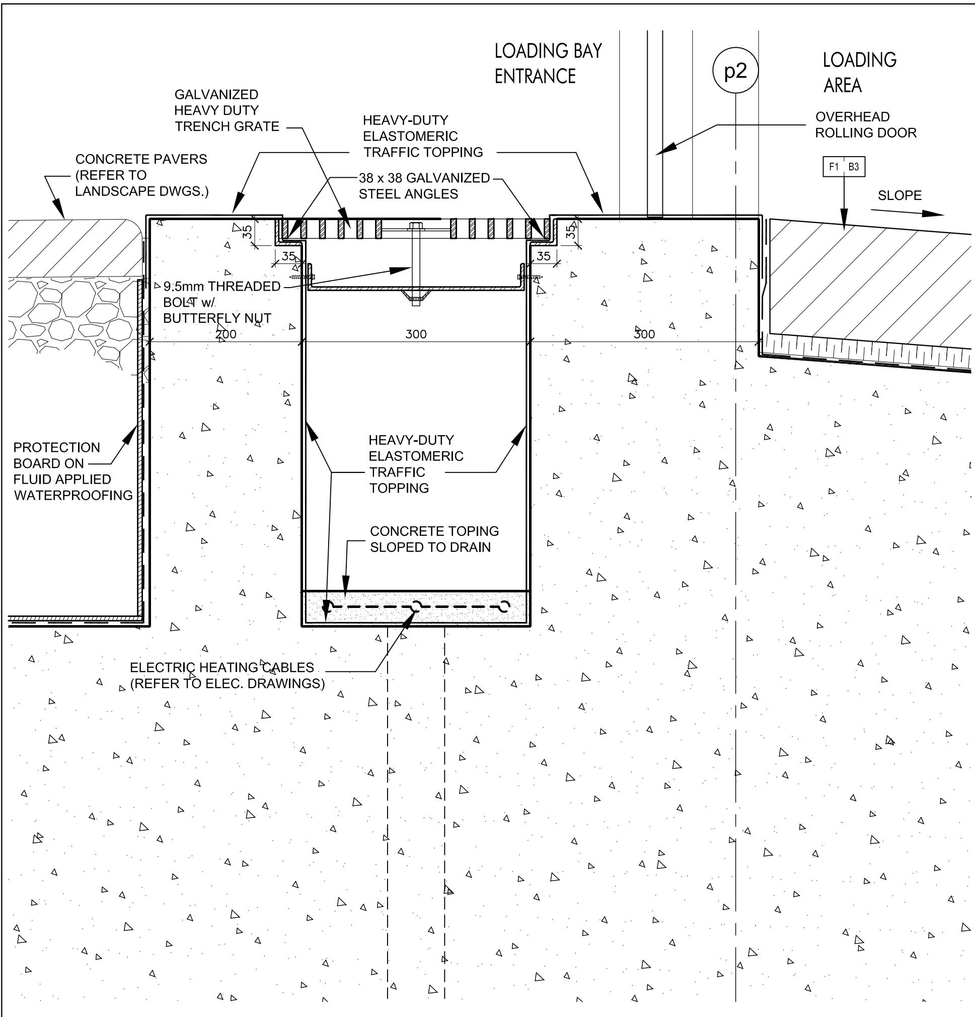
Entrance & O/H Door @ Loading Area 2 SCALE 1:5 A7-08
