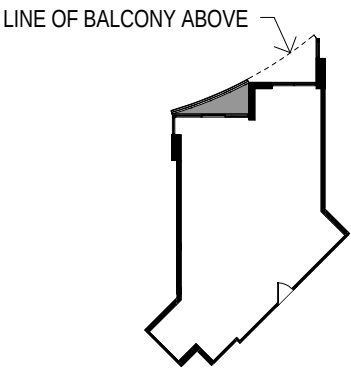
BALCONY PLAN: FLOORS 4, 6 2C1
