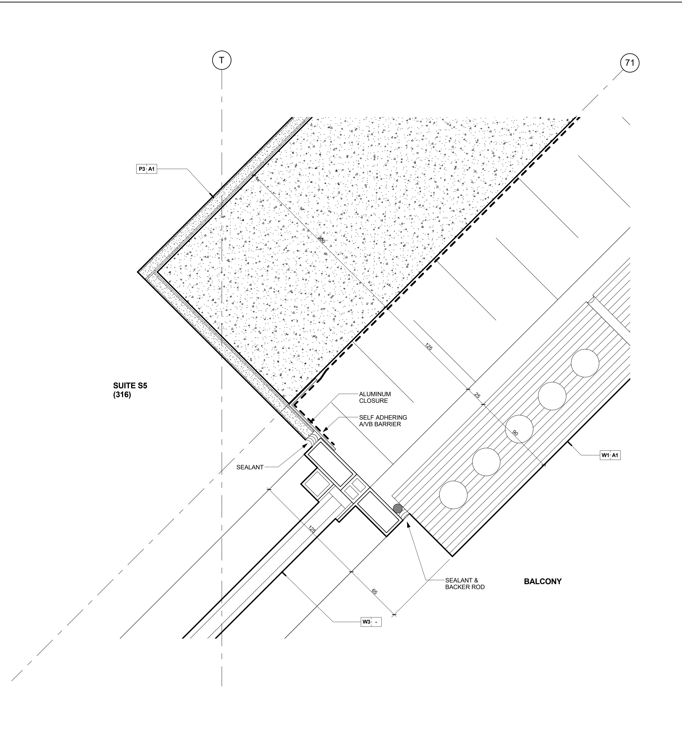
Enlarged Plan Detail @ Window Wall Brick Veneer Wall on Struct. Conc. Scale: 1 : 2 2 A7-25
