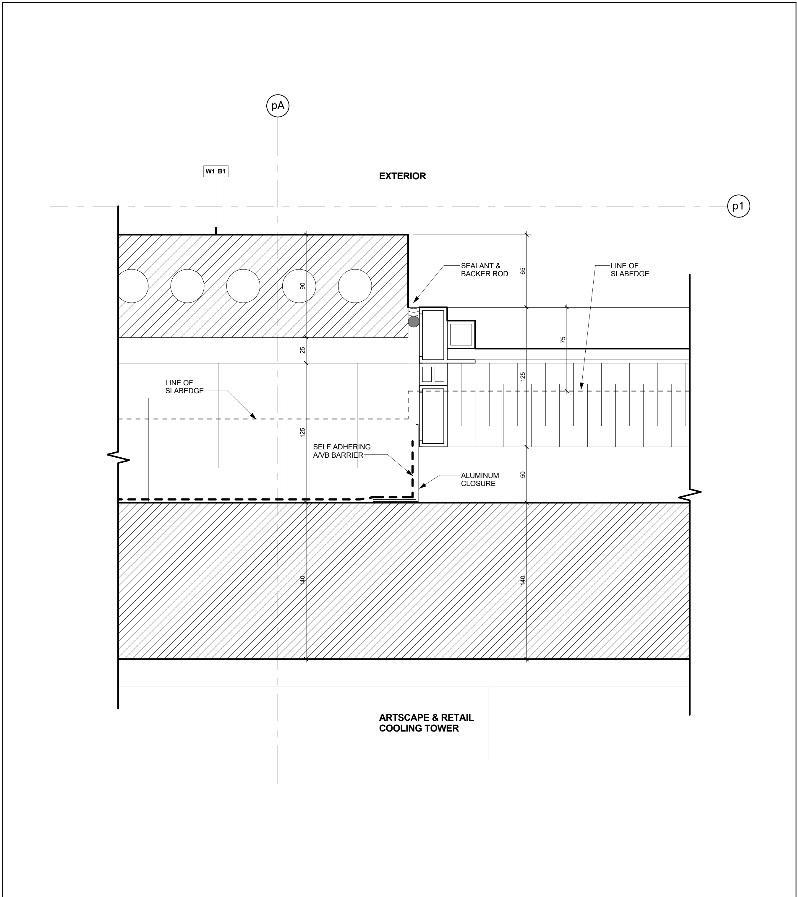
Enlarged Plan Detail @ Window Jamb @ Brick Veneer Wall with Conc. Block Scale: 1 : 2 4 A7-25
