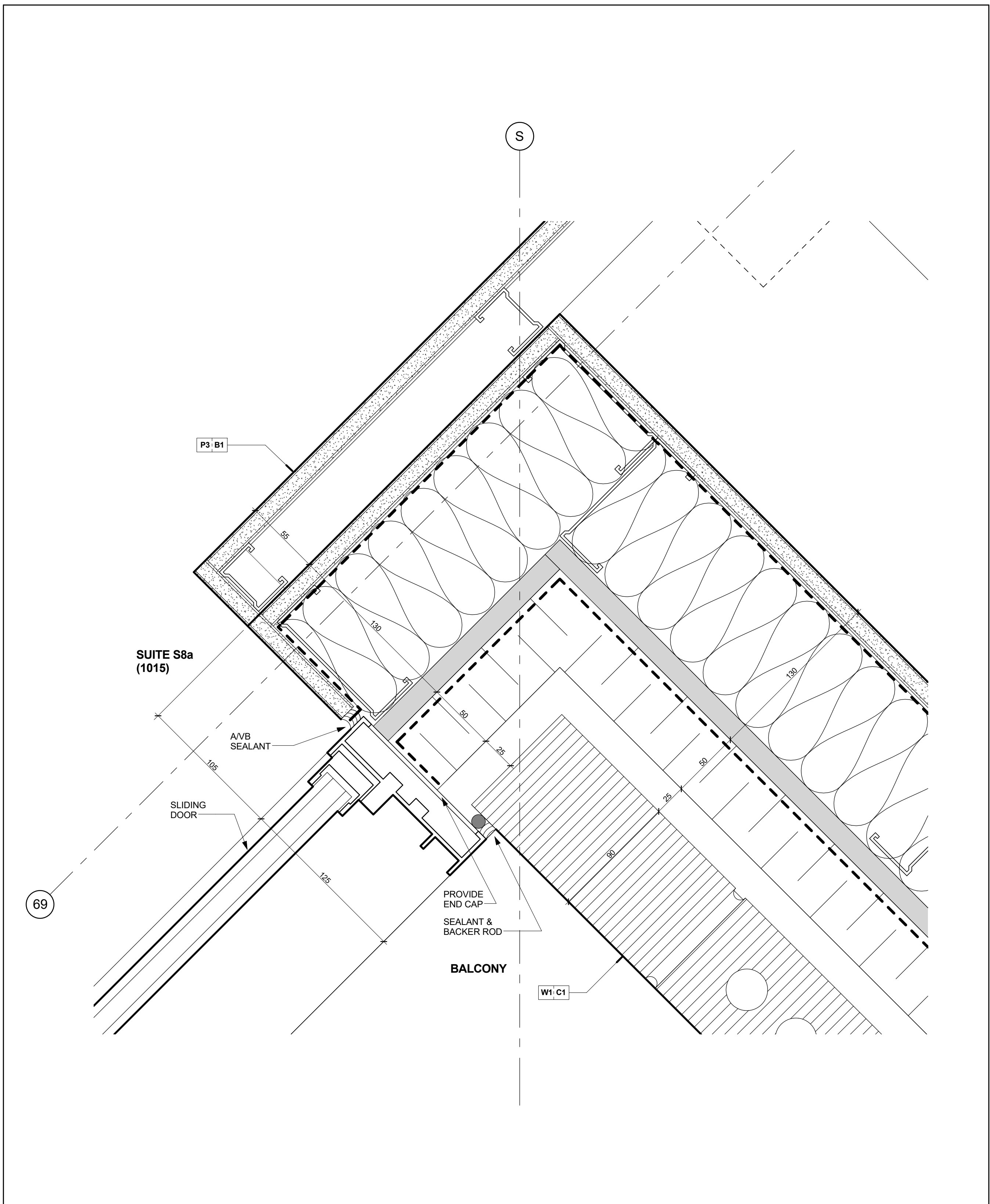
Enlarged Plan Detail @ Window Jamb @ Brick Veneer Wall with Metal Studs Scale: 1 : 2 3 A7-25
