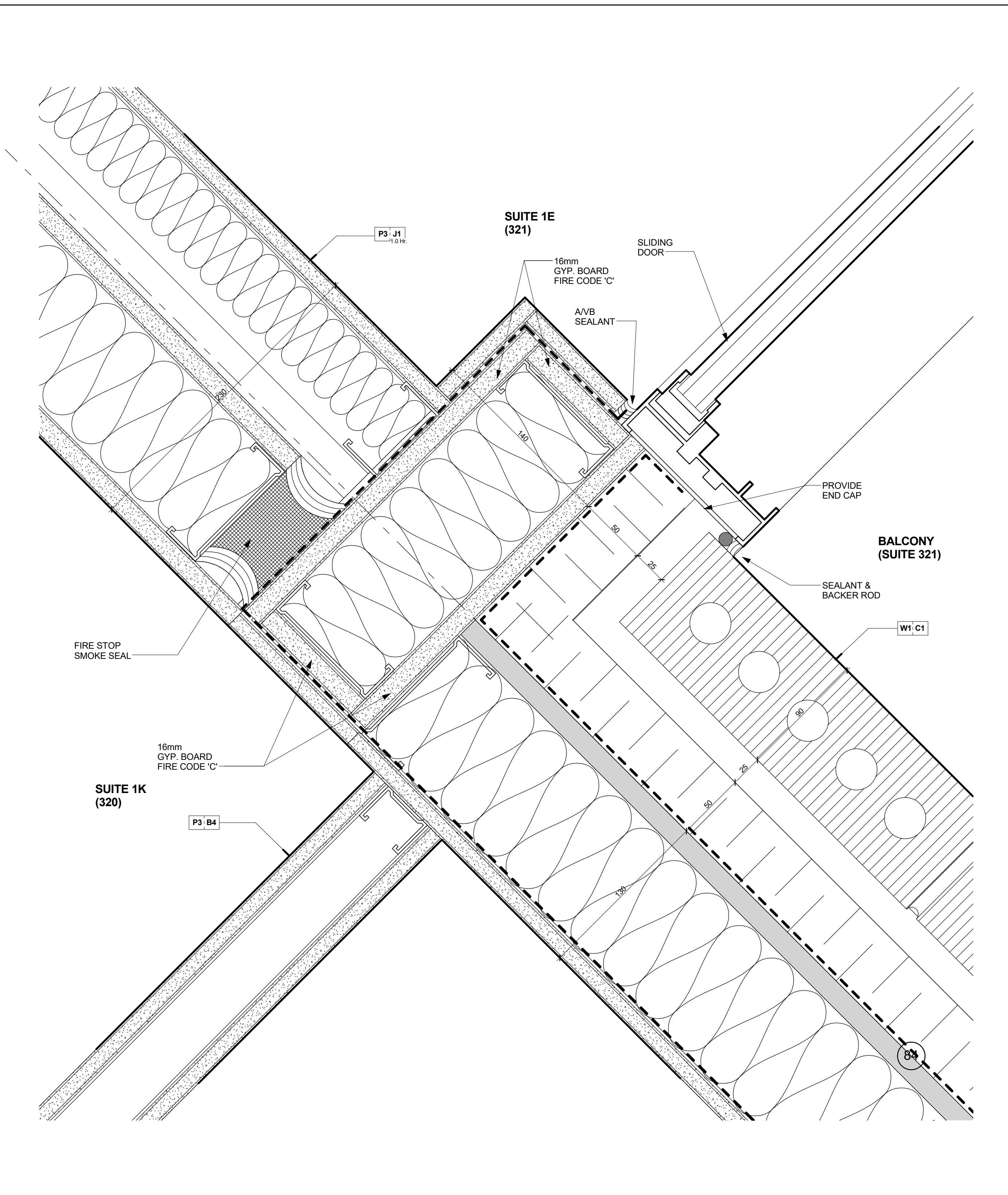
Enlarged Plan Detail @ Demising Wall (M/Studs) @ Brick Veneer Wall with Metal Studs Scale: 1 : 2 1 A7-25
