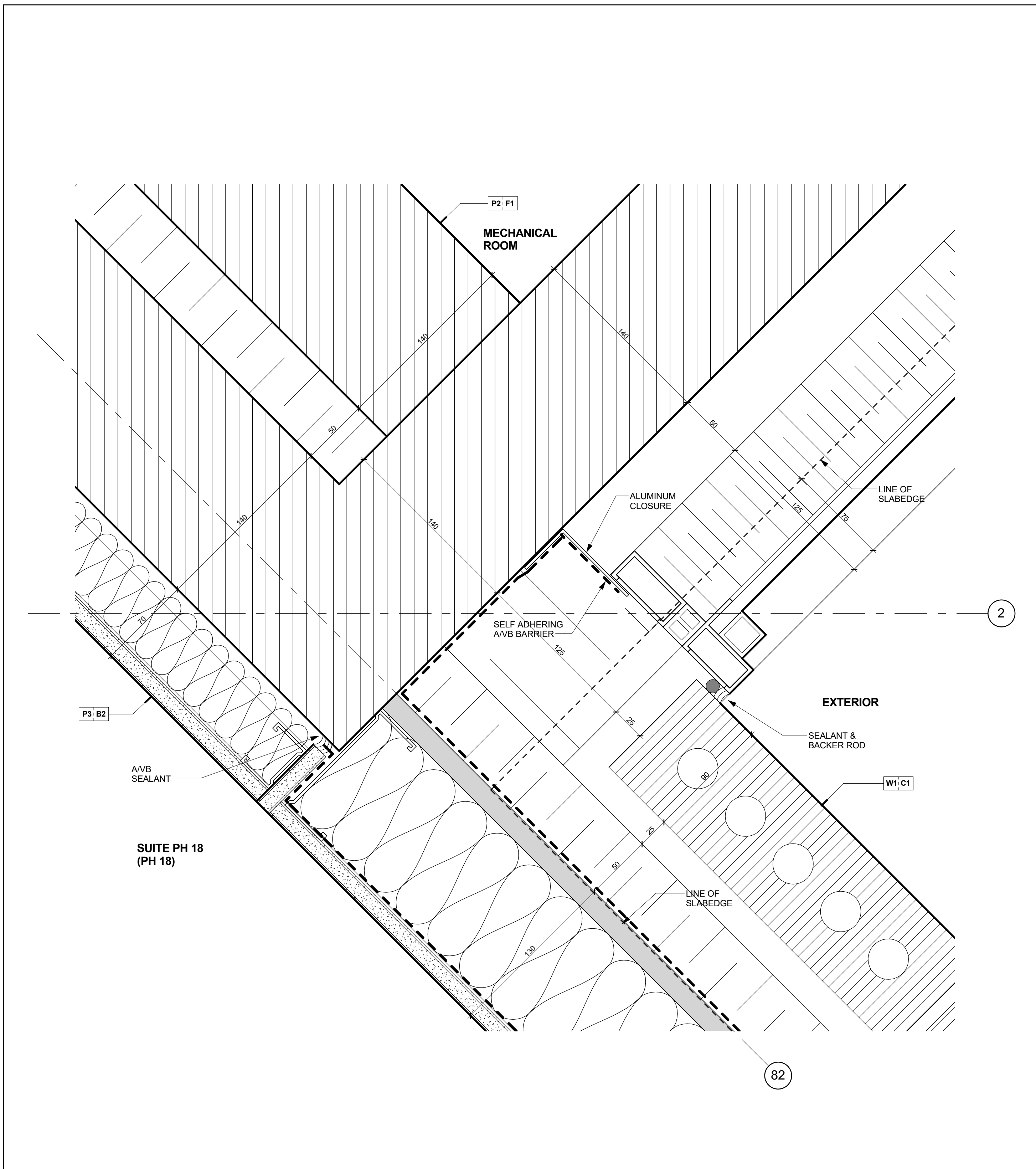
Enlarged Plan Detail @ Window Jamb @ Brick Veneer Wall with Metal Studs Scale: 1 : 2 5 A7-25
