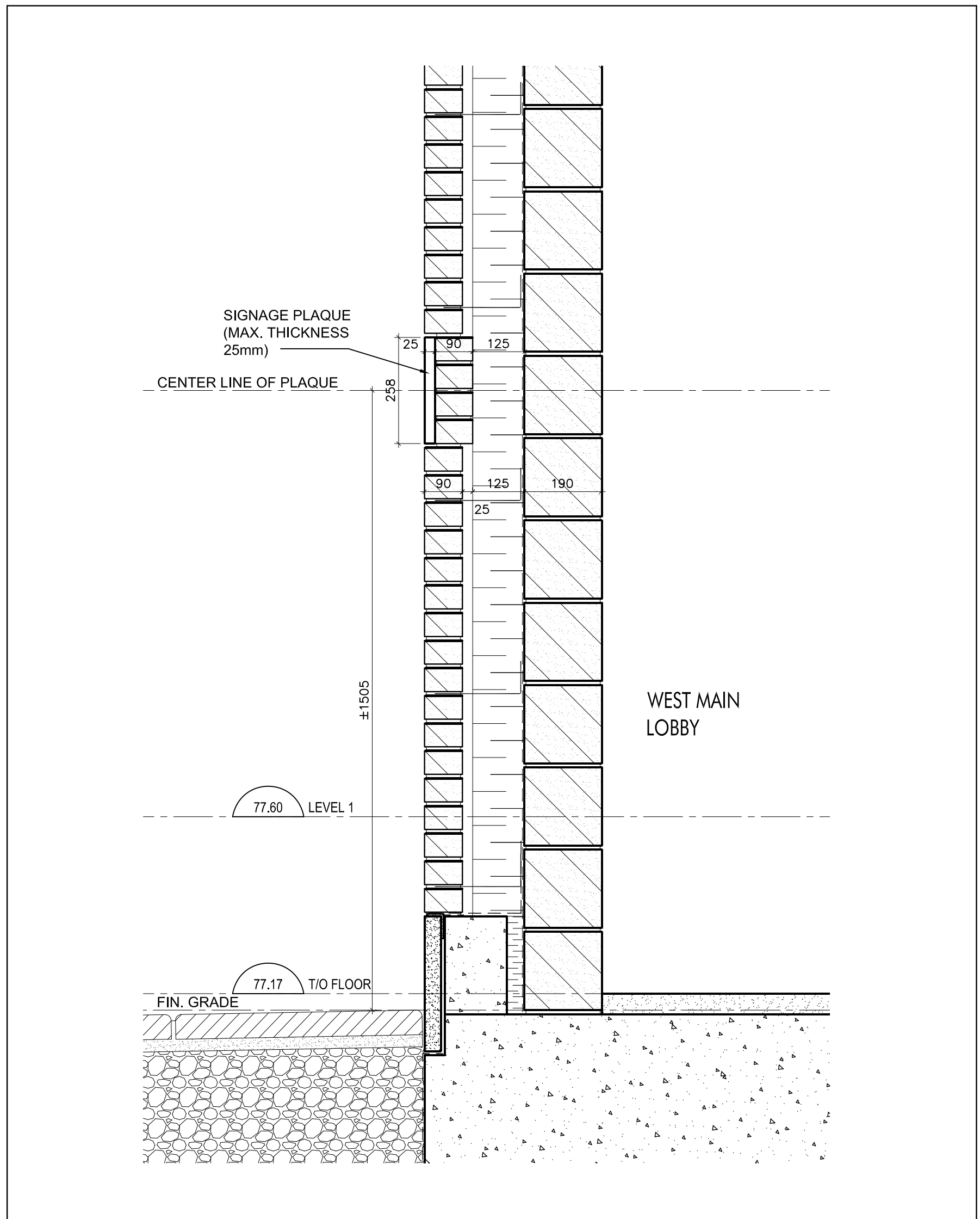
Section Thru Entrance Signage Plaque 7 A7-18
