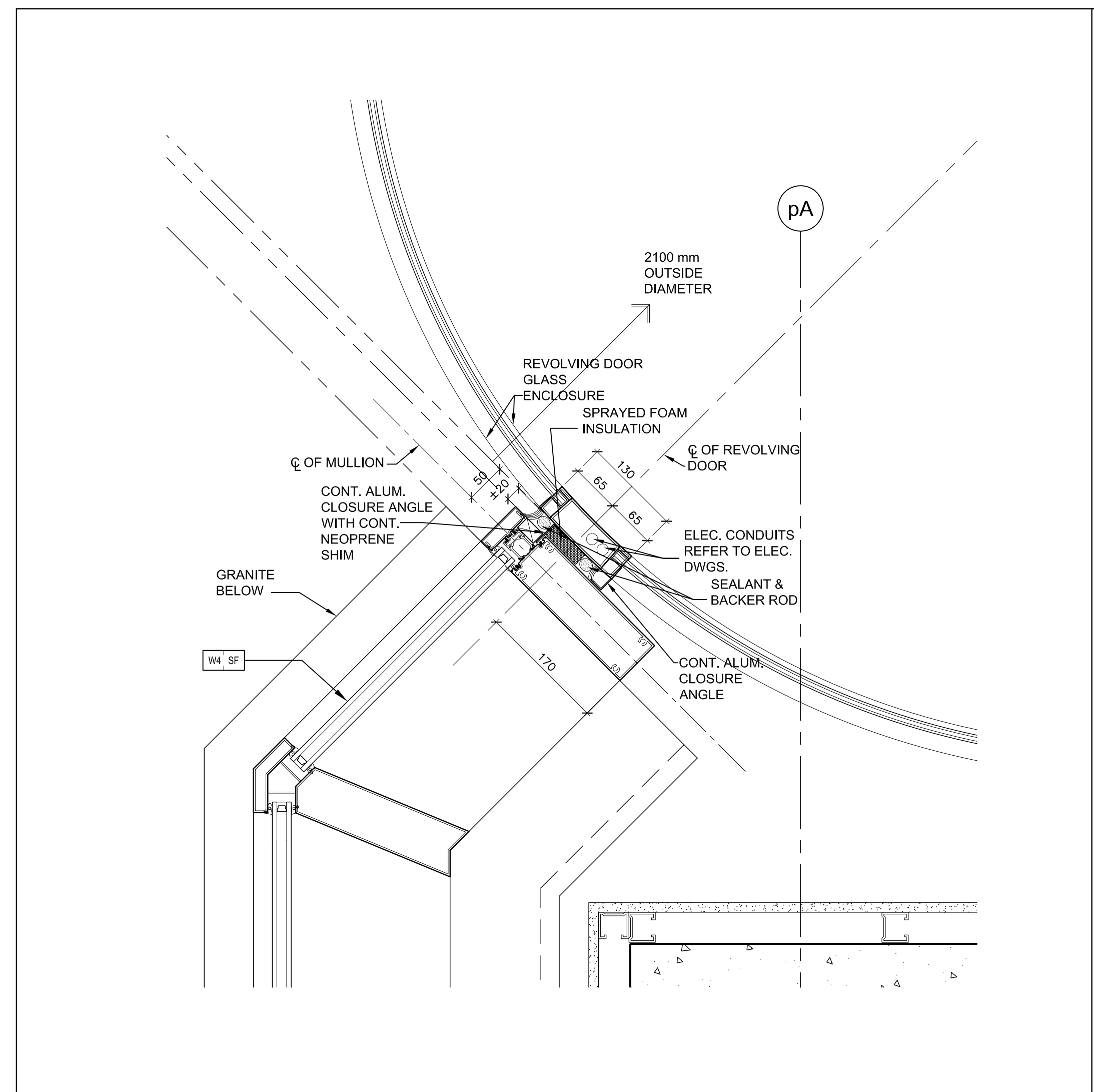
Plan Detail @ Revolving Door / Window Jamb 3 A7-18
