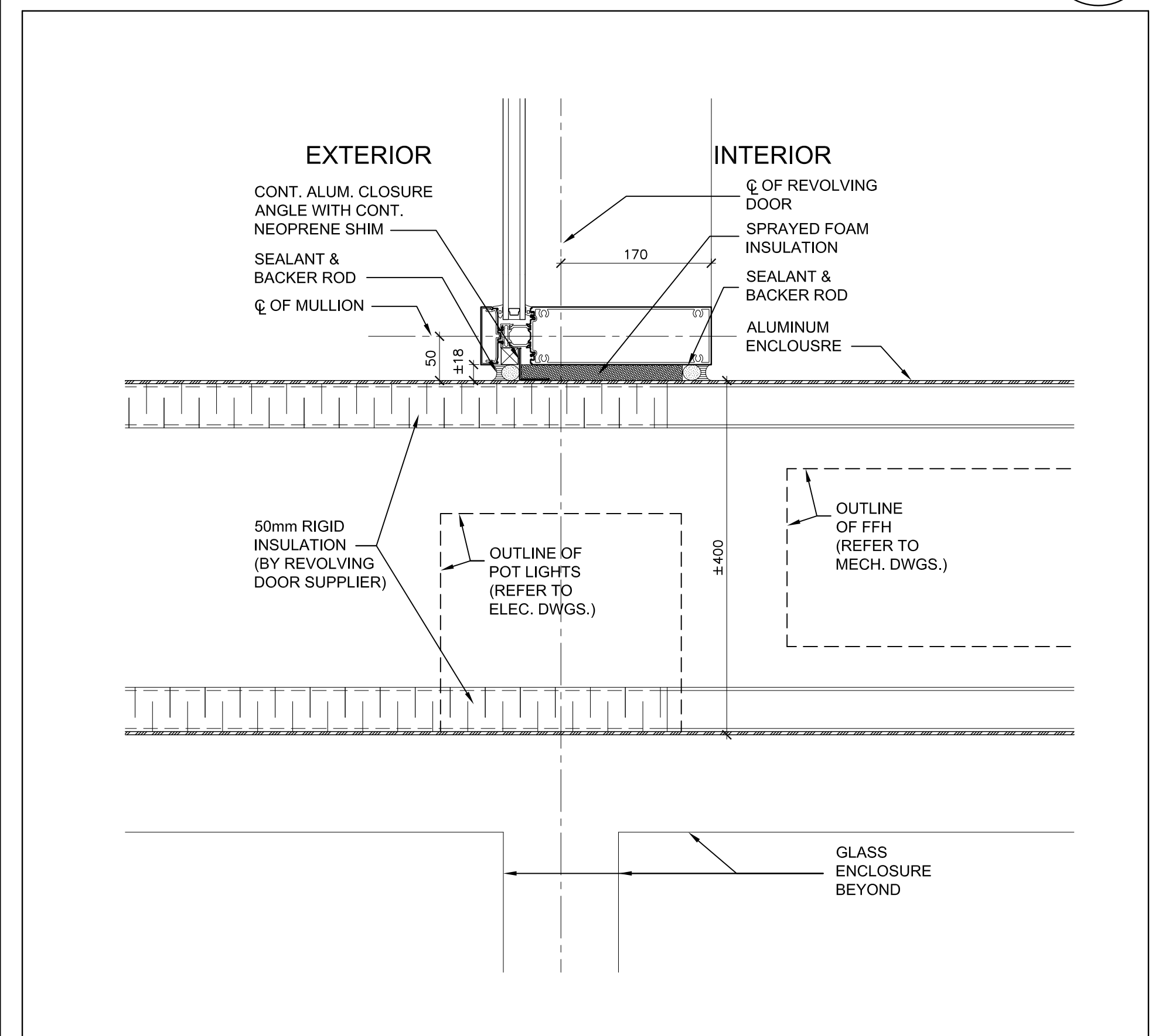
Section Detail @ Revolving Door Roof 4 A7-18
