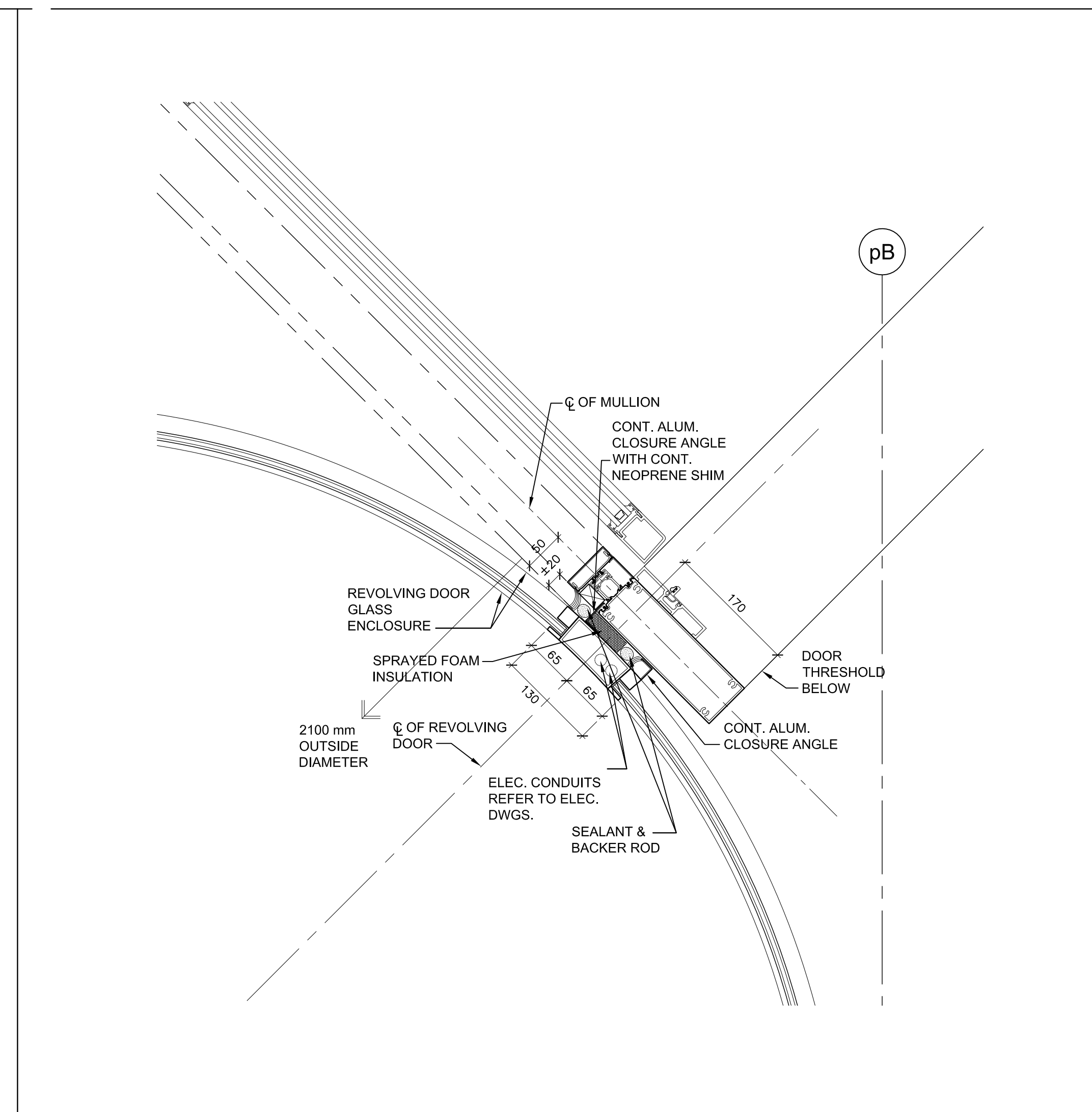
Plan Detail @ Revolving Door / Swing Door Jamb 2 A7-18
