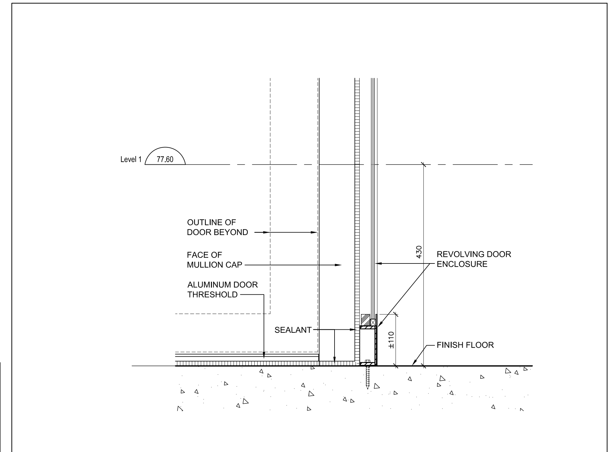
Section Detail @ Revolving Door Enclosure 5 A7-18
