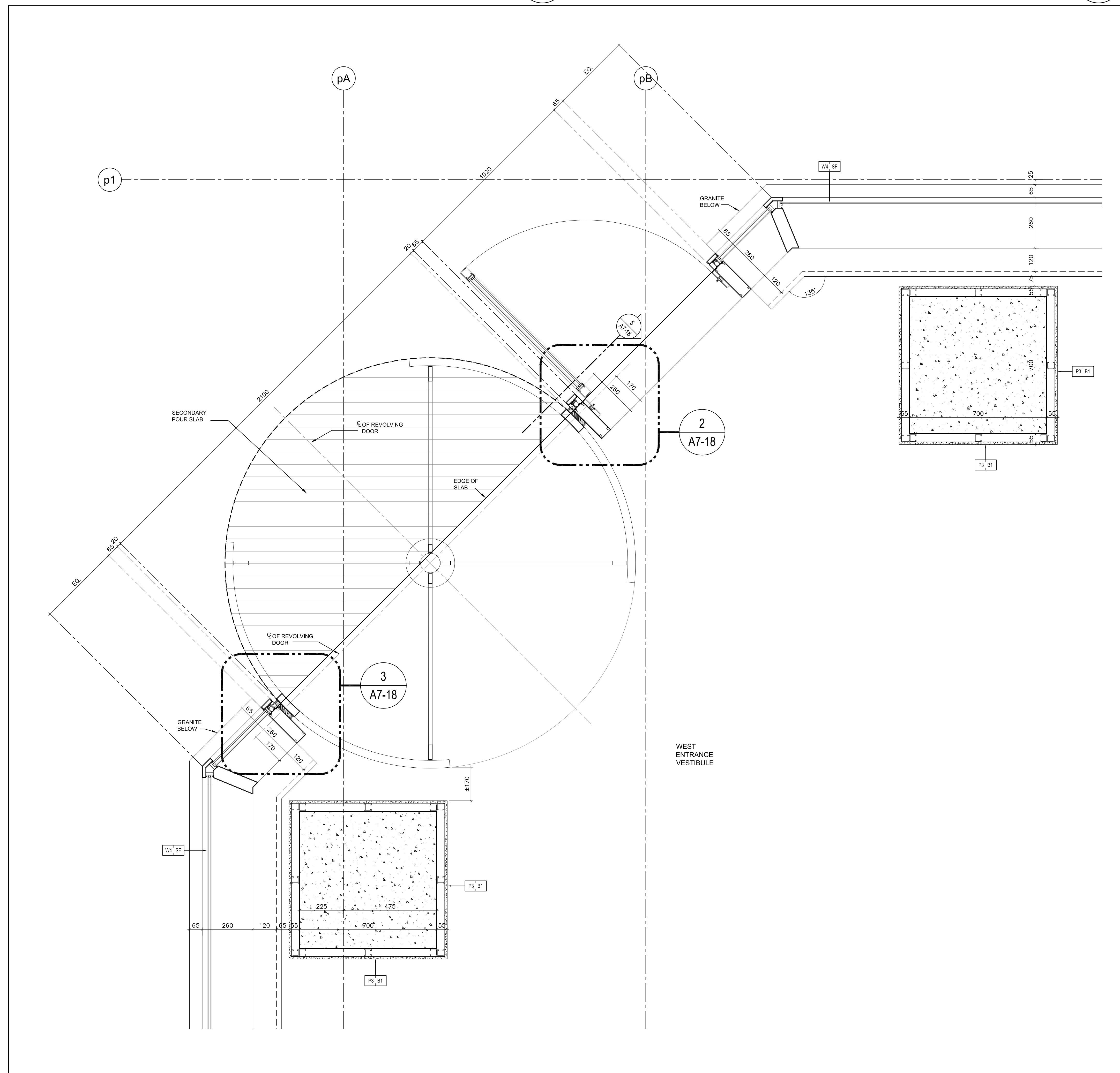
Plan Detail @ Revolving Door @ West Entrance Vestibule @ Level 1 1 A7-18
