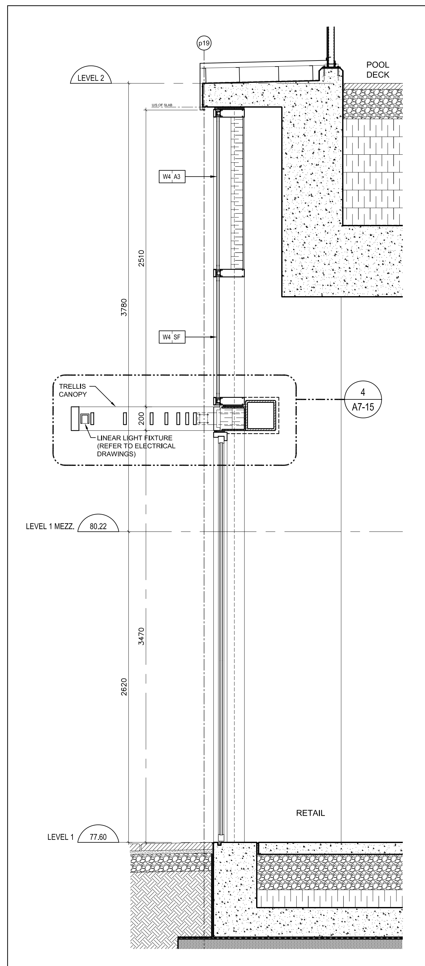
Section thru Bi-Fold Door @ Retail @ Level 1 7 A7-17 SCALE 1:20
