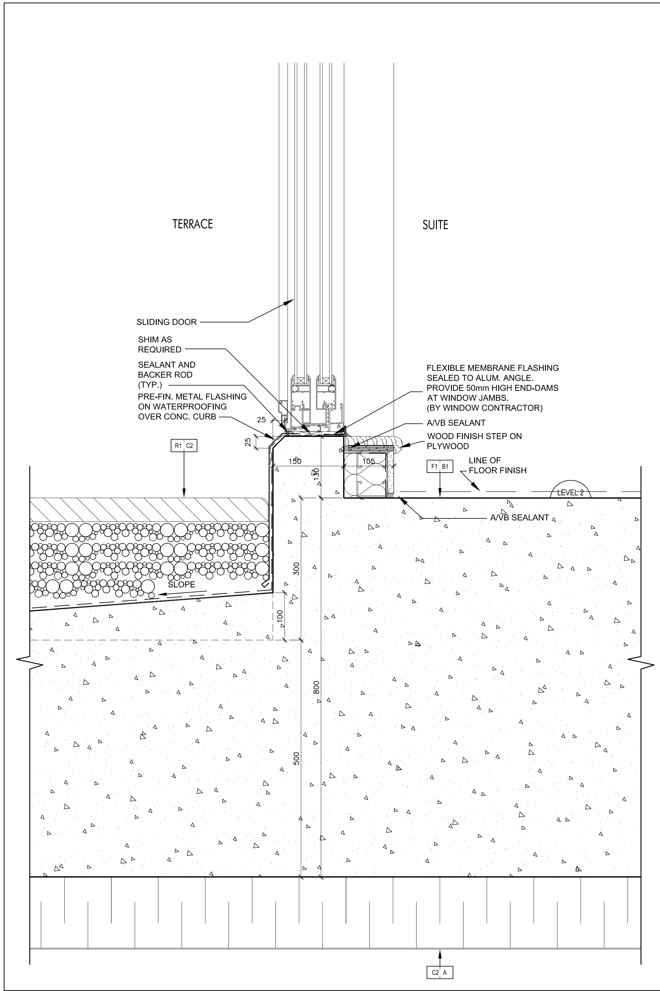
Concrete Curb @ Sliding Door @ Terrace At Level 2 SCALE: 1:5 A7-11
